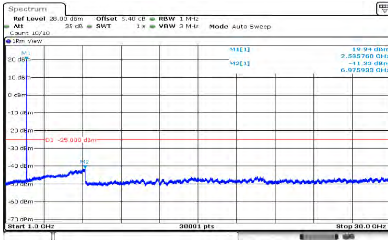
Band38-20MHz-16QAM-38000-1RB#0-Range2:1000~30000MHz
