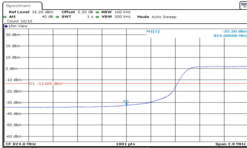
Band5-10MHz-16QAM-20450-50RB#0
