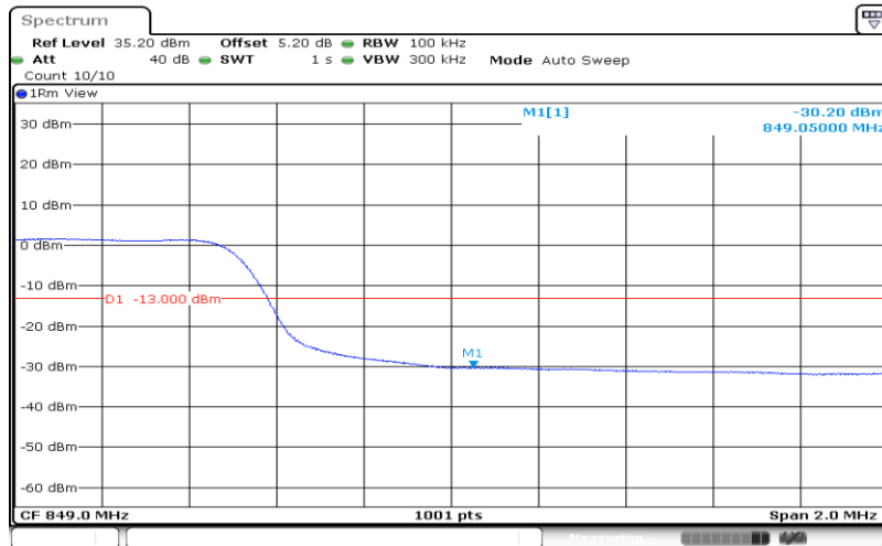
Band5-10MHz-QPSK-20600-50RB#0
