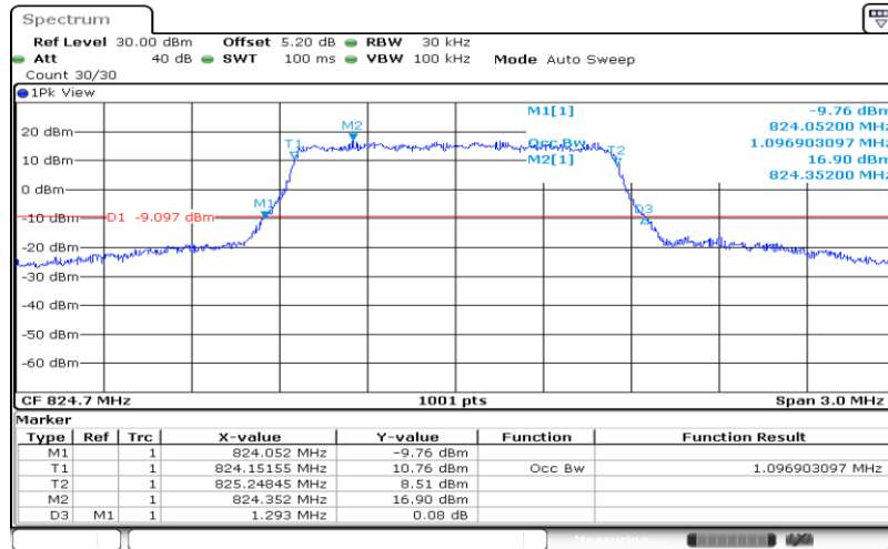
Band5-1.4MHz-QPSK-20407-6RB#0-1.097
