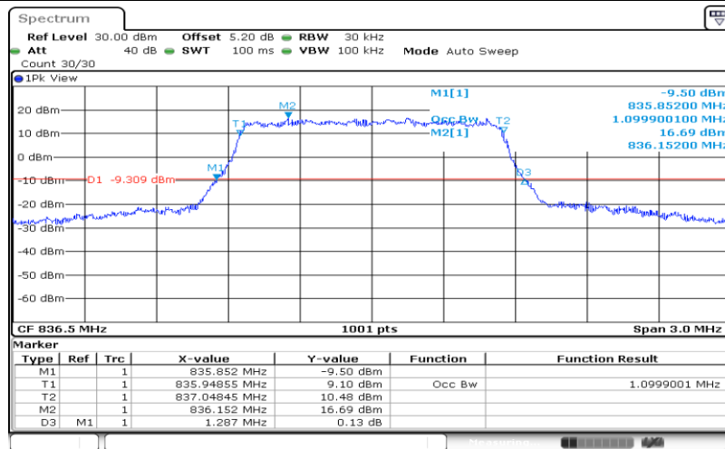
Band5-1.4MHz-QPSK-20525-6RB#0-1.1
