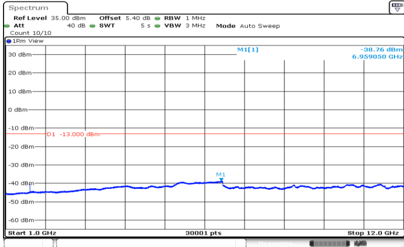
Band5-10MHz-16QAM-20525-1RB#0-Range2:1000~12000MHz
