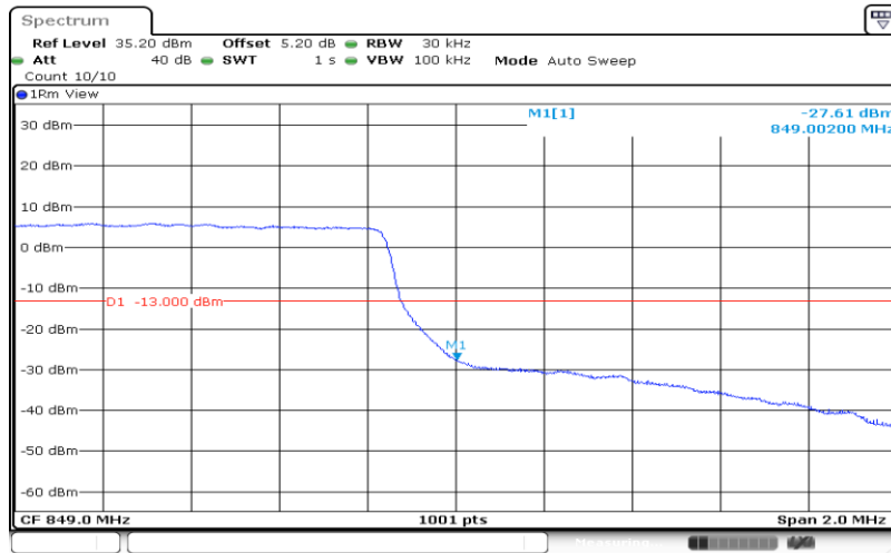
Band5-1.4MHz-16QAM-20643-6RB#0
