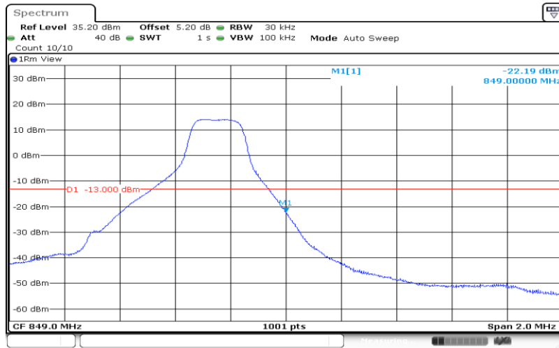
Band5-1.4MHz-16QAM-20643-6RB#0
