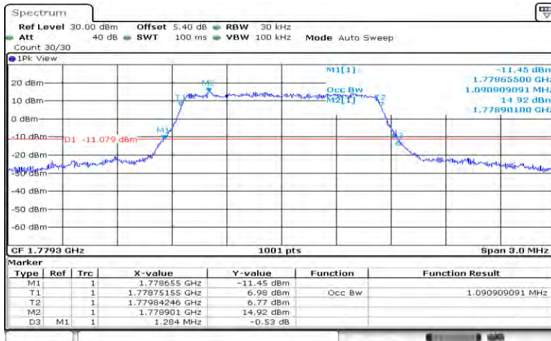
Band66-1.4MHz-16QAM-132665-6RB#0-1.091
