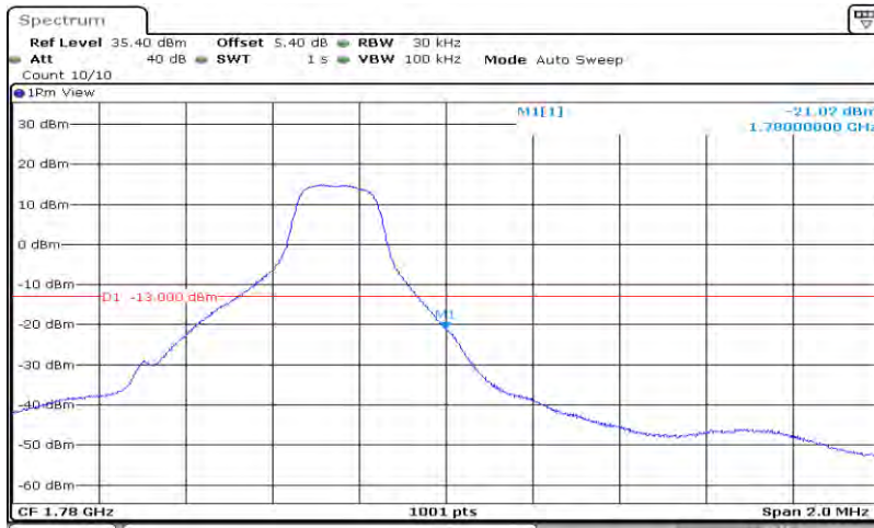
Band66-1.4MHz-QPSK-132665-6RB#0
