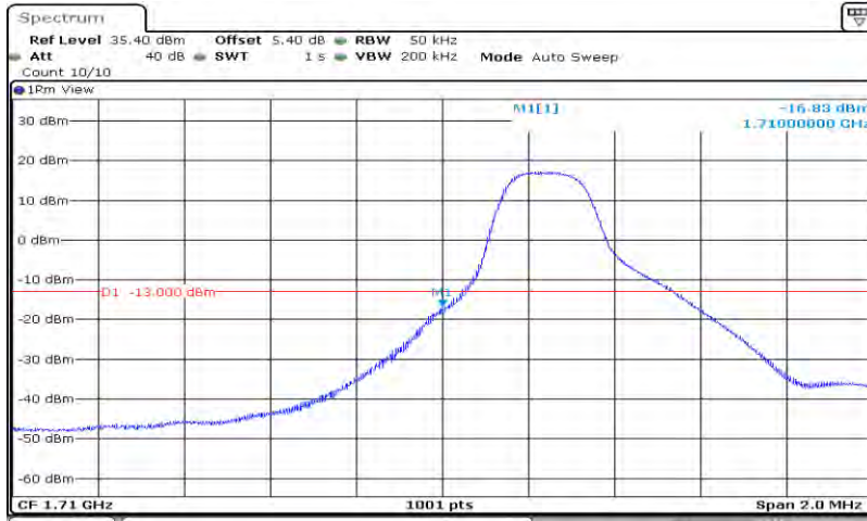
Band66-3MHz-QPSK-131987-15RB#0
