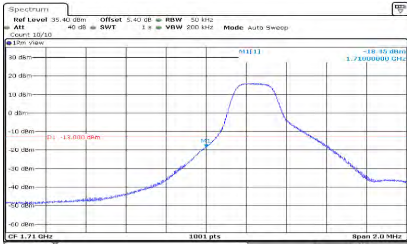
Band66-3MHz-16QAM-131987-15RB#0
