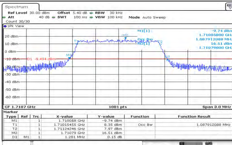
Band66-1.4MHz-QPSK-131979-6RB#0-1.088
