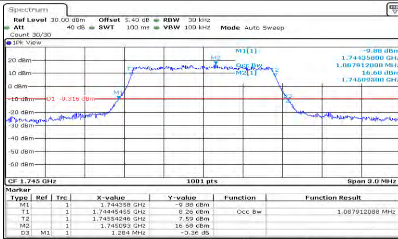
Band66-1.4MHz-QPSK-132322-6RB#0-1.088
