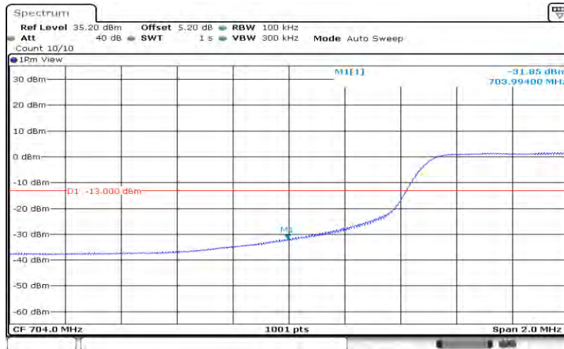
Band17-10MHz-16QAM-23780-50RB#0
