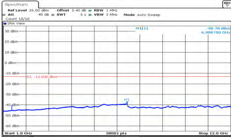
Band17-10MHz-16QAM-23790-1RB#0-Range2:1000~12000MHz
