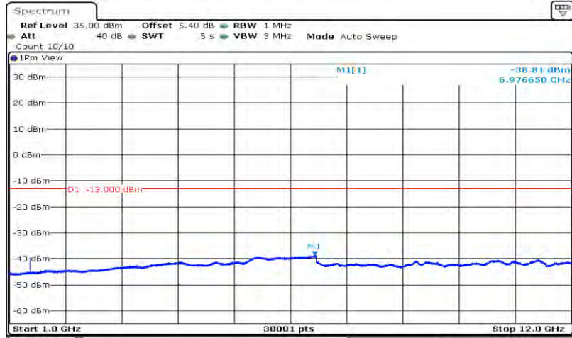
Band17-10MHz-16QAM-23780-1RB#0-Range2:1000~12000MHz
