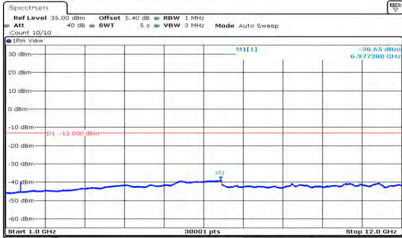
Band17-10MHz-QPSK-23790-1RB#0-Range2:1000~12000MHz
