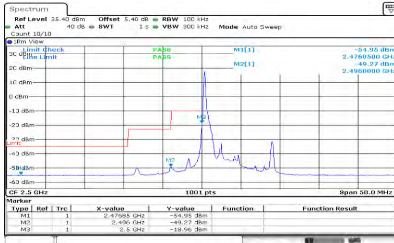
Band7-5MHz-16QAM-20775-25RB#0
