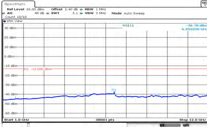
Band5-10MHz-16QAM-20525-1RB#0-Range2:1000~12000MHz
