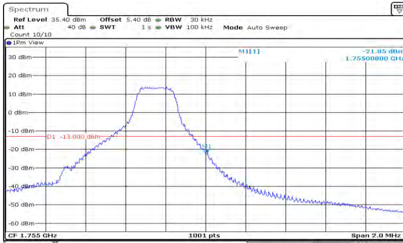
Band4-1.4MHz-16QAM-20393-6RB#0
