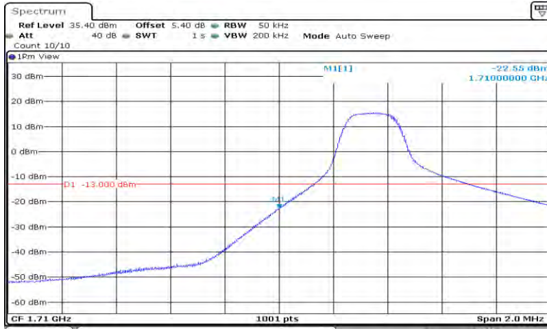
Band4-5MHz-16QAM-19975-25RB#0
