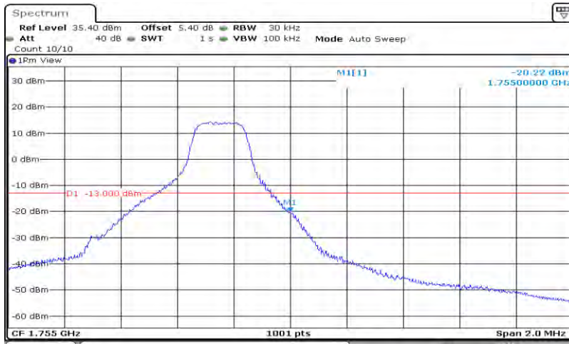
Band4-1.4MHz-QPSK-20393-6RB#0
