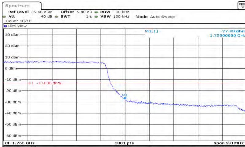
Band4-1.4MHz-QPSK-20393-6RB#0
