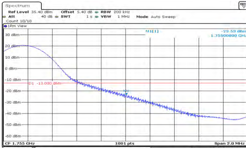
Band4-15MHz-QPSK-20325-75RB#0
