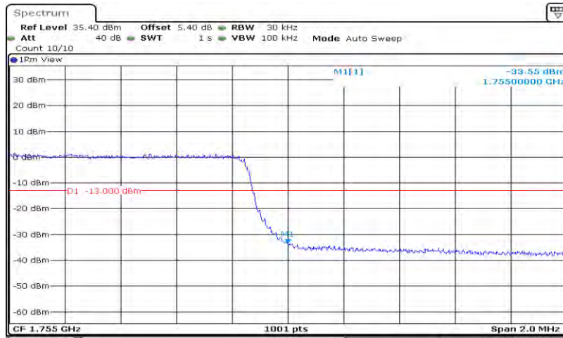
Band4-3MHz-16QAM-20385-15RB#0
