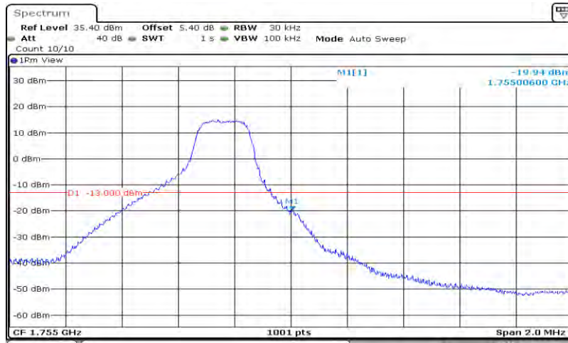
Band4-3MHz-QPSK-20385-15RB#0
