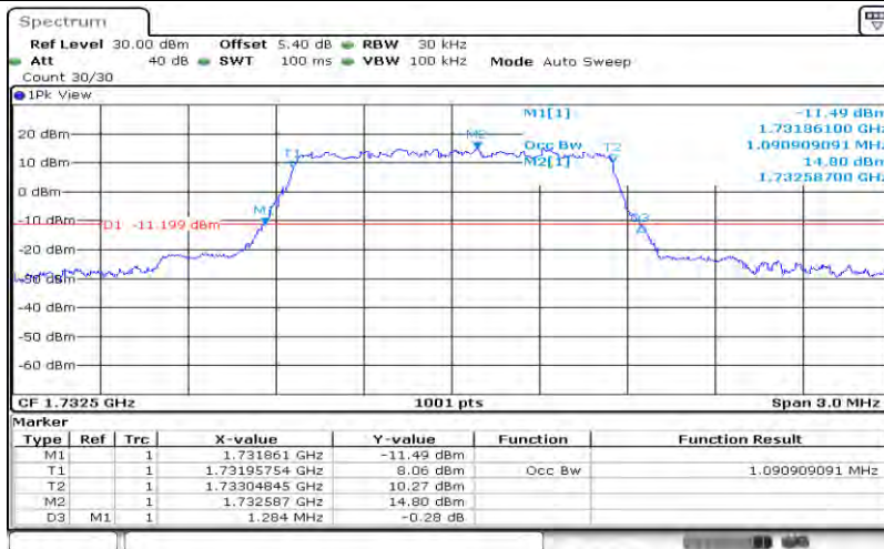
Band4-1.4MHz-QPSK-20175-6RB#0-1.091
