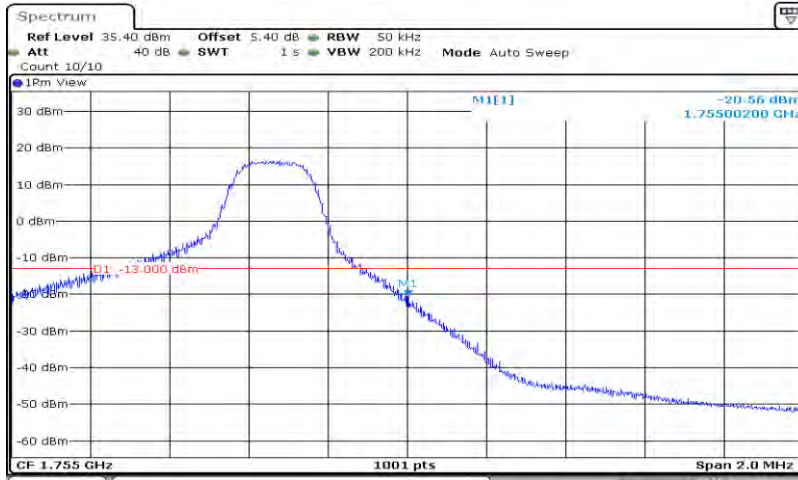
Band4-5MHz-QPSK-20375-25RB#0
