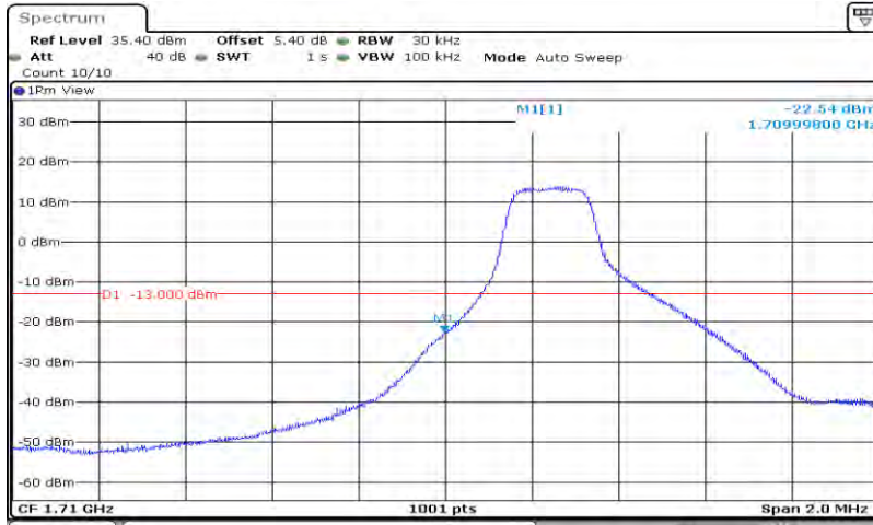
Band4-3MHz-16QAM-19965-15RB#0
