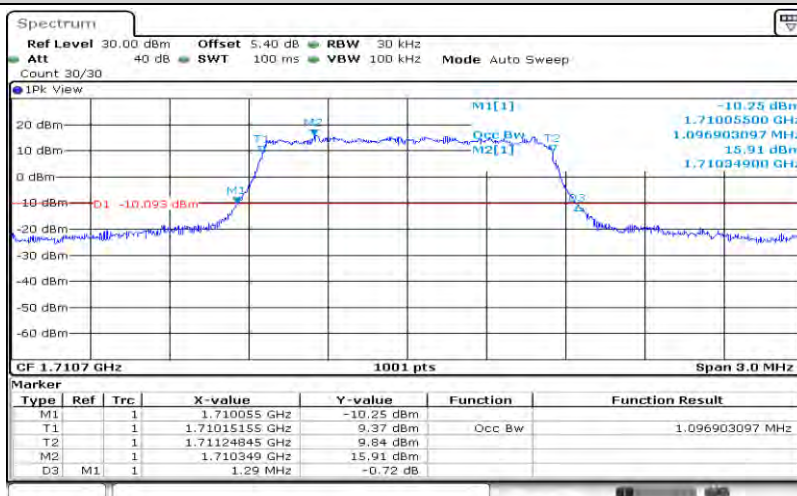
Band4-1.4MHz-QPSK-19957-6RB#0-1.097
