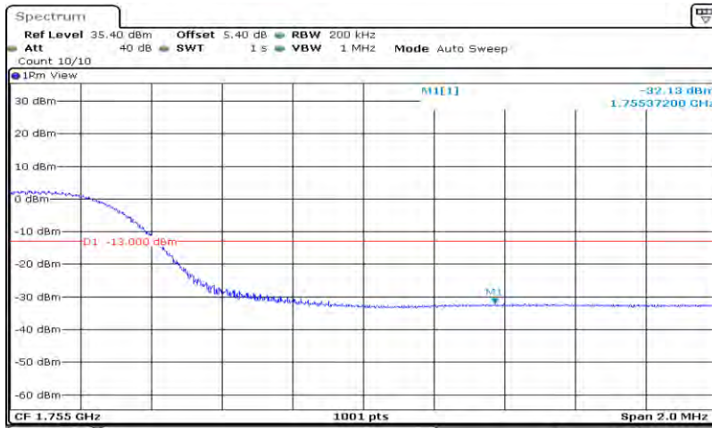
Band4-15MHz-QPSK-20325-75RB#0
