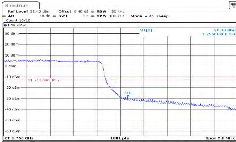
Band4-1.4MHz-16QAM-20393-6RB#0
