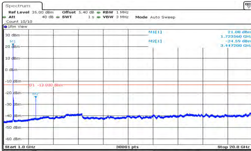
Band4-20MHz-16QAM-20175-1RB#0-Range2:1000~20000MHz
