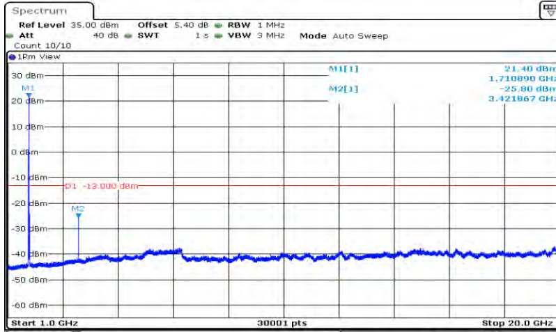
Band4-20MHz-16QAM-20050-1RB#0-Range2:1000~20000MHz
