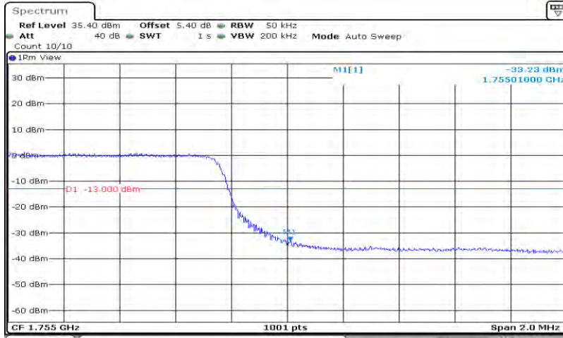
Band4-5MHz-16QAM-20375-25RB#0
