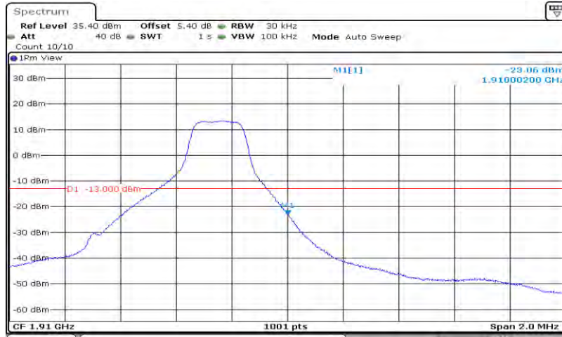
Band2-1.4MHz-16QAM-19193-6RB#0
