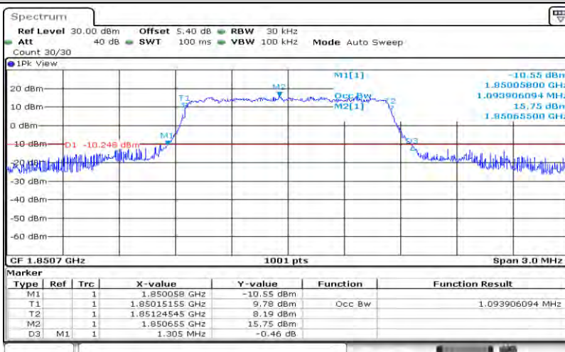
Band2-1.4MHz-QPSK-18607-6RB#0-1.094
