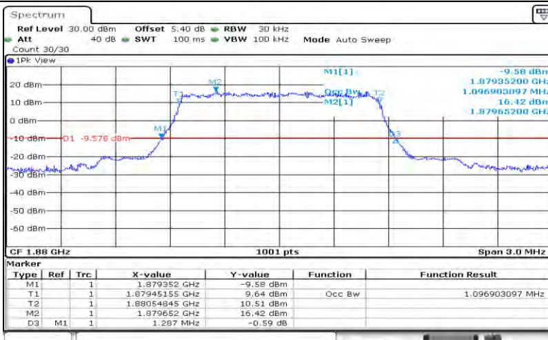
Band2-1.4MHz-QPSK-18900-6RB#0-1.097
