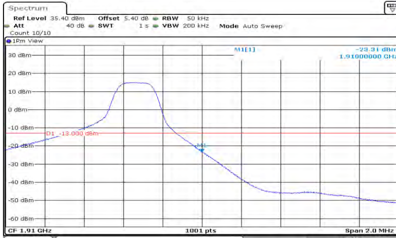
Band2-5MHz-QPSK-19175-25RB#0
