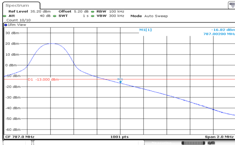
Band13-10MHz-QPSK-23230_Right-1RB#49
