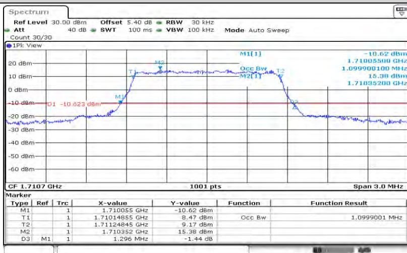
Band4-1.4MHz-QPSK-19957-6RB#0-1.1
