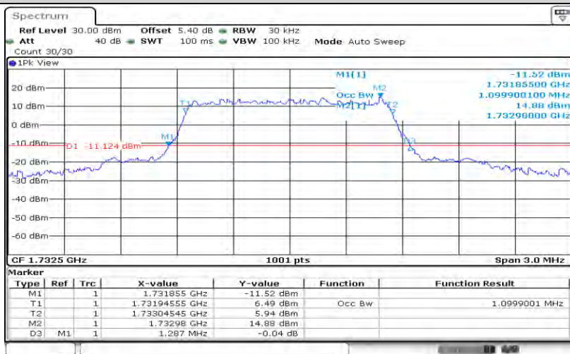
Band4-1.4MHz-QPSK-20175-6RB#0-1.1
