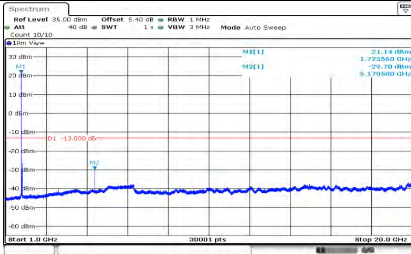
Band4-20MHz-16QAM-20175-1RB#0-Range2:1000~20000MHz
