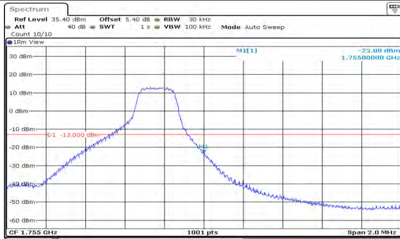
Band4-3MHz-16QAM-20385-15RB#0
