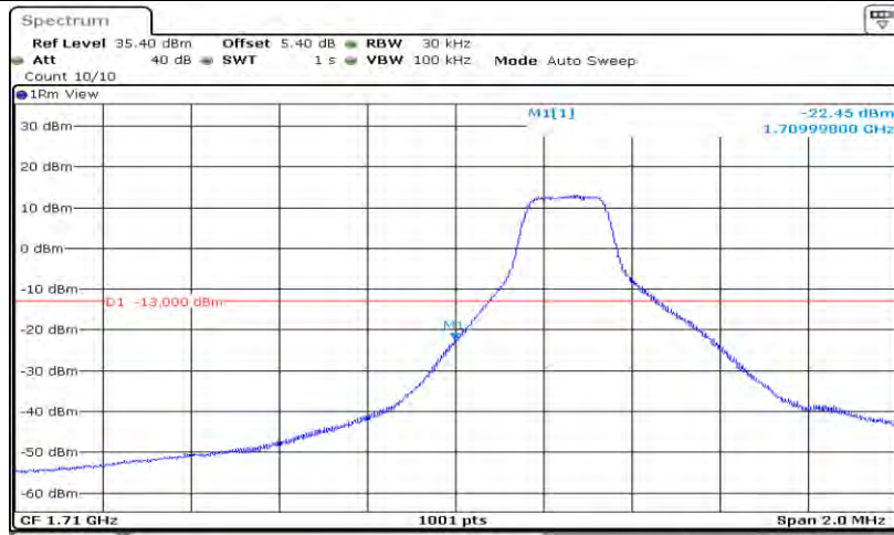
Band4-1.4MHz-16QAM-19957-6RB#0
