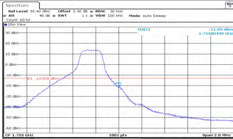
Band4-3MHz-QPSK-20385-15RB#0
