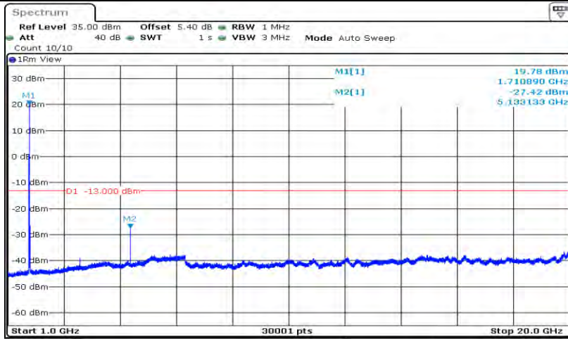
Band4-20MHz-16QAM-20050-1RB#0-Range2:1000~20000MHz
