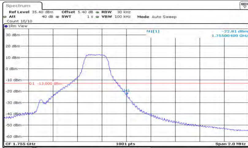
Band4-1.4MHz-16QAM-20393-6RB#0
