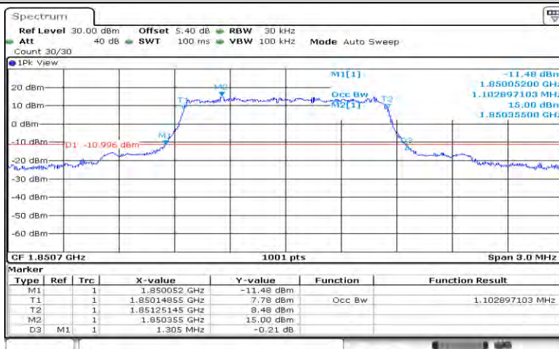
Band2-1.4MHz-QPSK-18607-6RB#0-1.103
