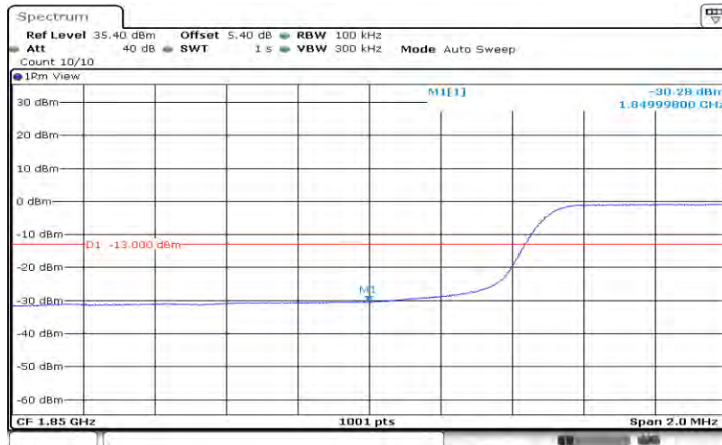
Band2-10MHz-16QAM-18650-50RB#0
