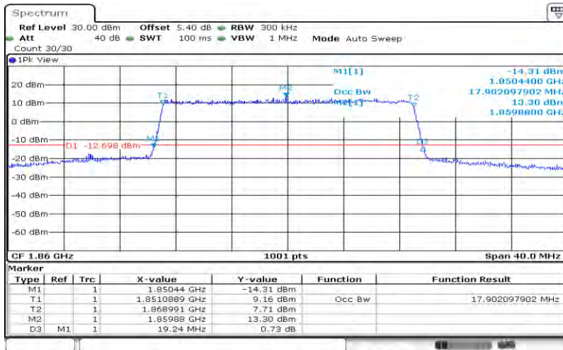
Band2-20MHz-16QAM-18700-100RB#0-17.902
