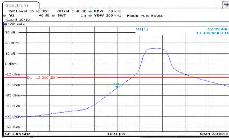
Band2-5MHz-16QAM-18625-25RB#0
