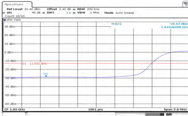
Band2-15MHz-QPSK-18675-75RB#0
