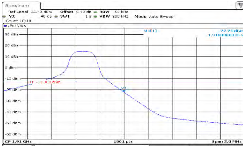
Band2-5MHz-16QAM-19175-25RB#0
