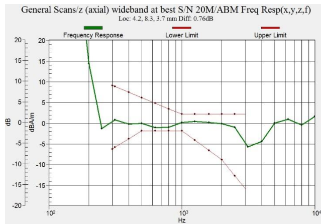
Figure C.17 Frequency Response of LTE B66 - OTT VoIP
