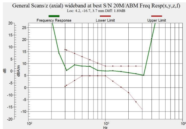
Figure C.18 Frequency Response of LTE B41 Power Class 2 - OTT VoIP
