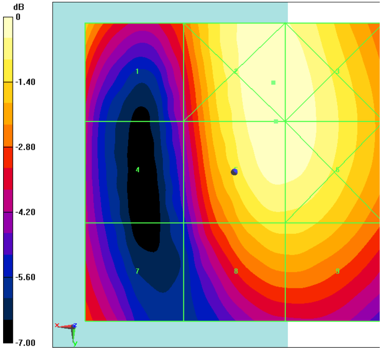
Fig B.9 HAC RF E-Field LTE Band41 Power Class 2 QPSK CH40620
