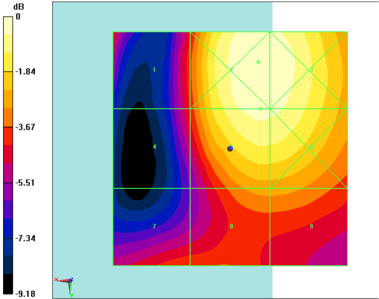
Fig B.19 HAC RF E-Field LTE Band41 Power Class 3 QPSK CH40620
