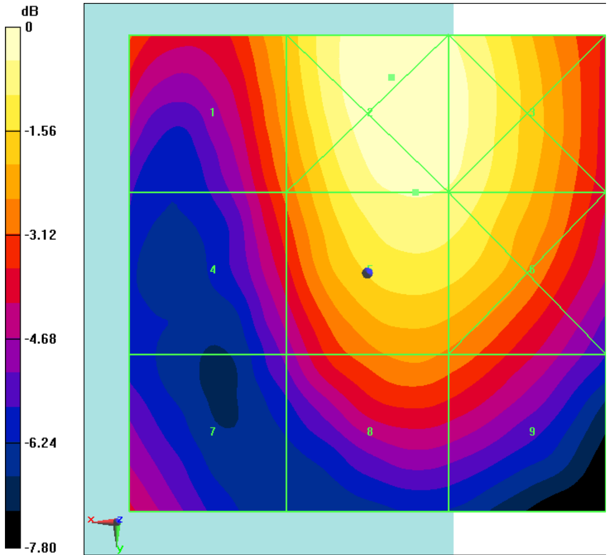
Fig B.11 HAC RF E-Field LTE Band41 Power Class 2 QPSK CH39750
