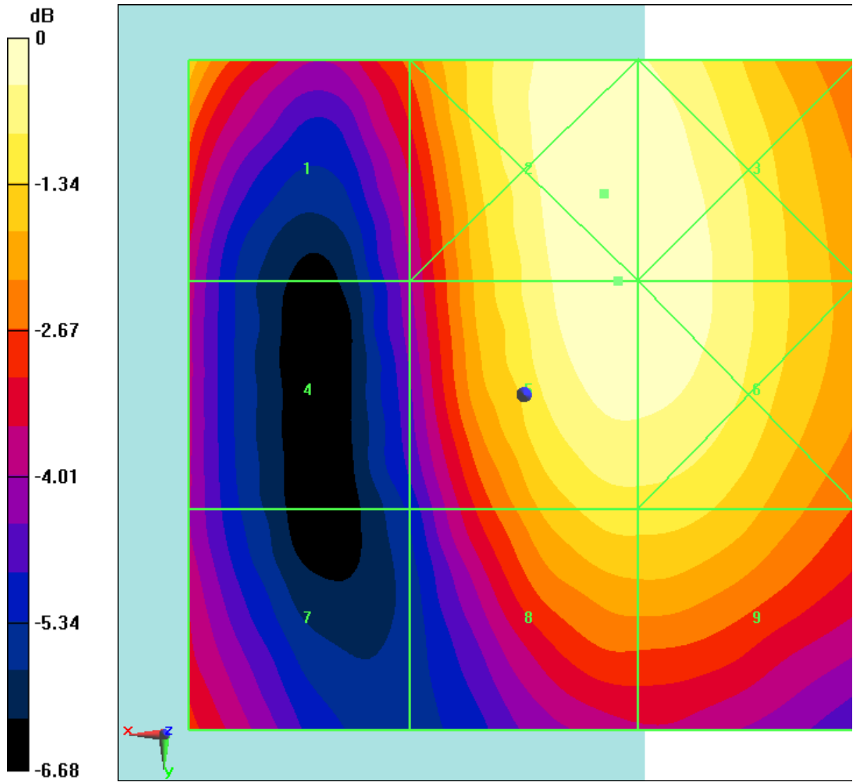
Fig B.14 HAC RF E-Field LTE Band41 Power Class 2 16QAM CH40620
