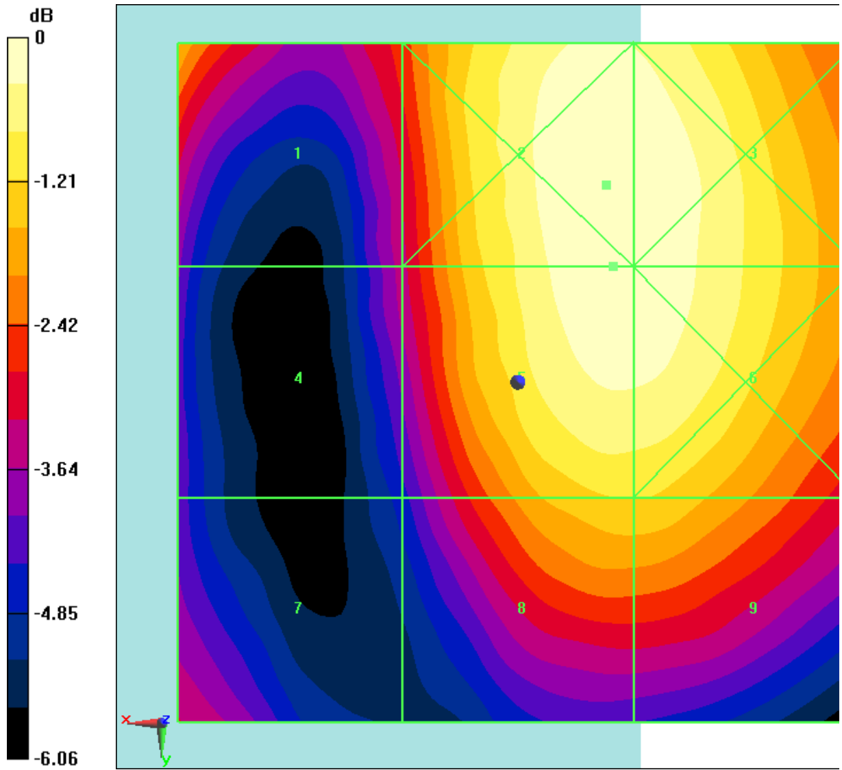
Fig B.25 HAC RF E-Field LTE Band41 Power Class 3 16QAM CH40185
