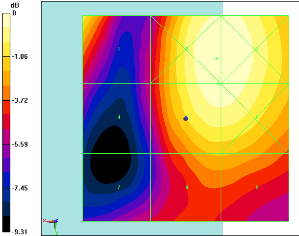
Fig B.18 HAC RF E-Field LTE Band41 Power Class 3 QPSK CH41055
