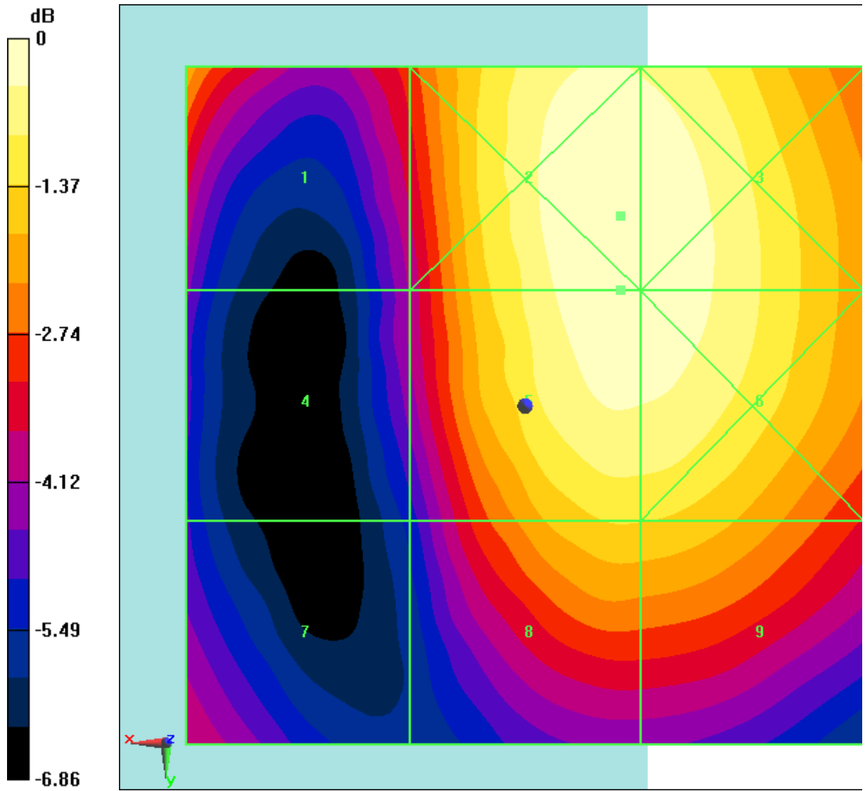
Fig B.10 HAC RF E-Field LTE Band41 Power Class 2 QPSK CH40185
