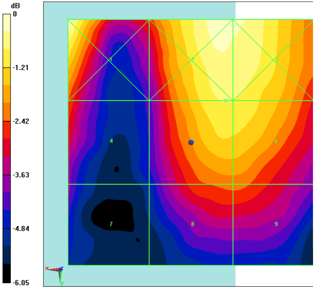
Fig B.12 HAC RF E-Field LTE Band41 Power Class 2 16QAM CH41490
