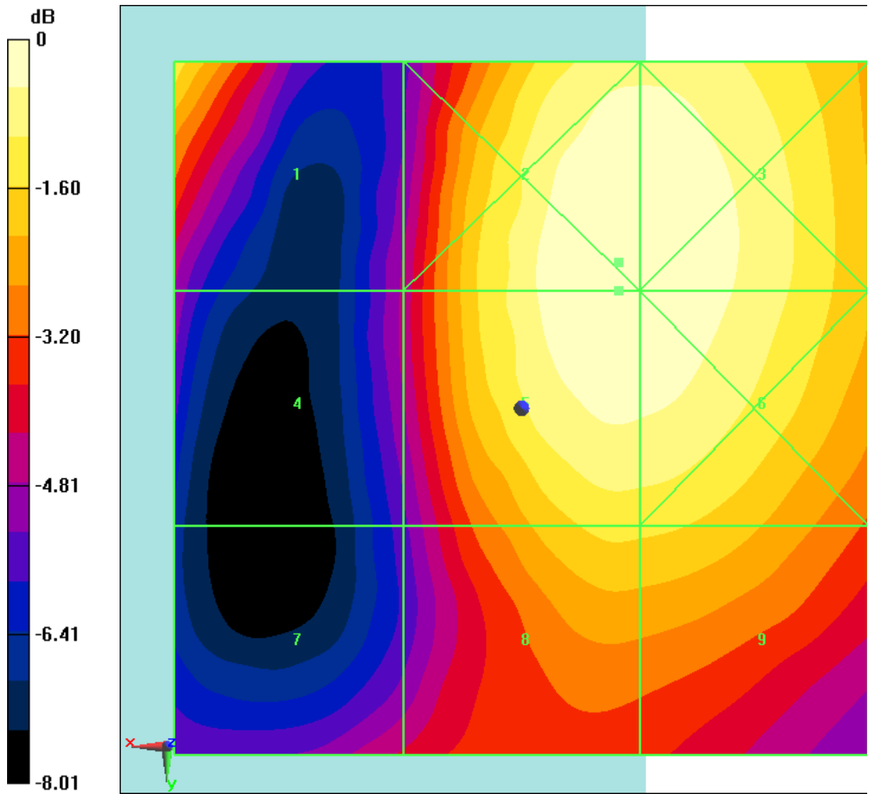
Fig B.17 HAC RF E-Field LTE Band41 Power Class 3 QPSK CH41490
