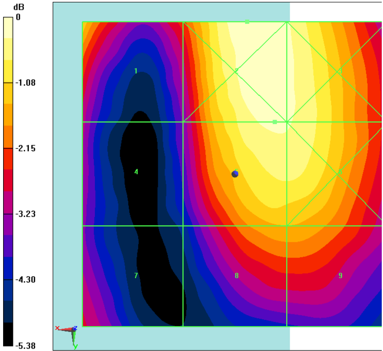
Fig B.8 HAC RF E-Field LTE Band41 Power Class 2 QPSK CH41055
