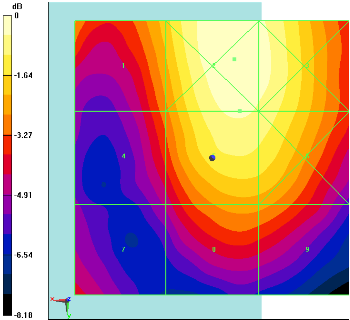
Fig B.16 HAC RF E-Field LTE Band41 Power Class 2 16QAM CH39750
