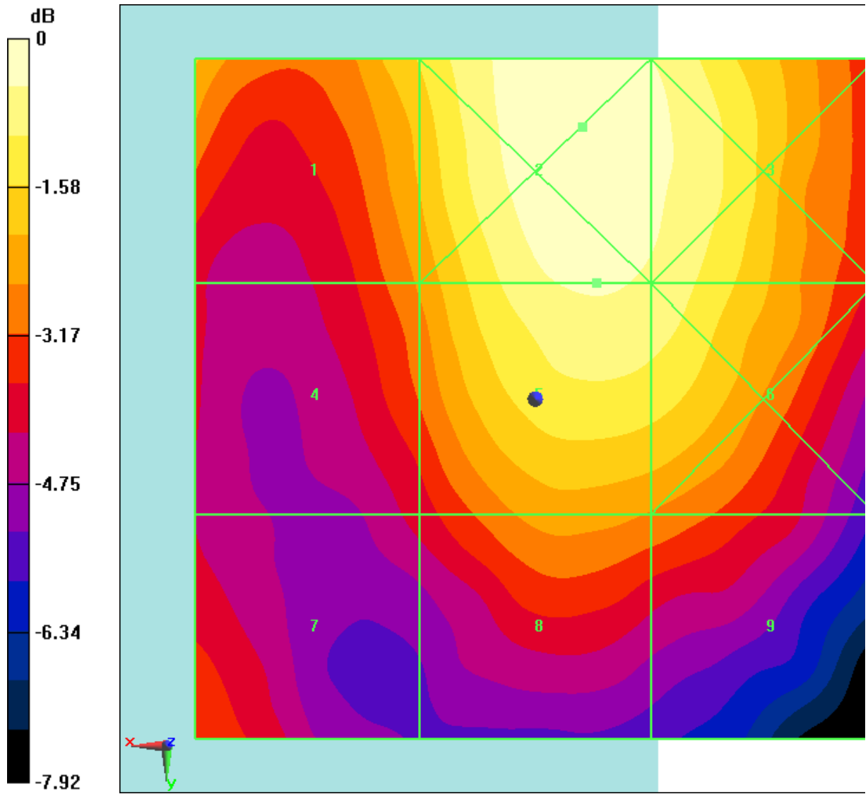
Fig B.26 HAC RF E-Field LTE Band41 Power Class 3 16QAM CH39750
