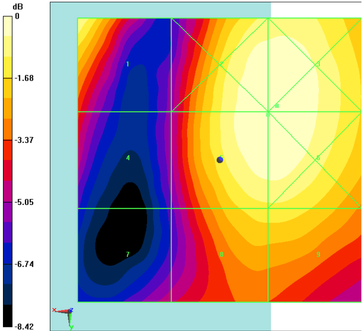
Fig B.22 HAC RF E-Field LTE Band41 Power Class 3 16QAM CH41490
