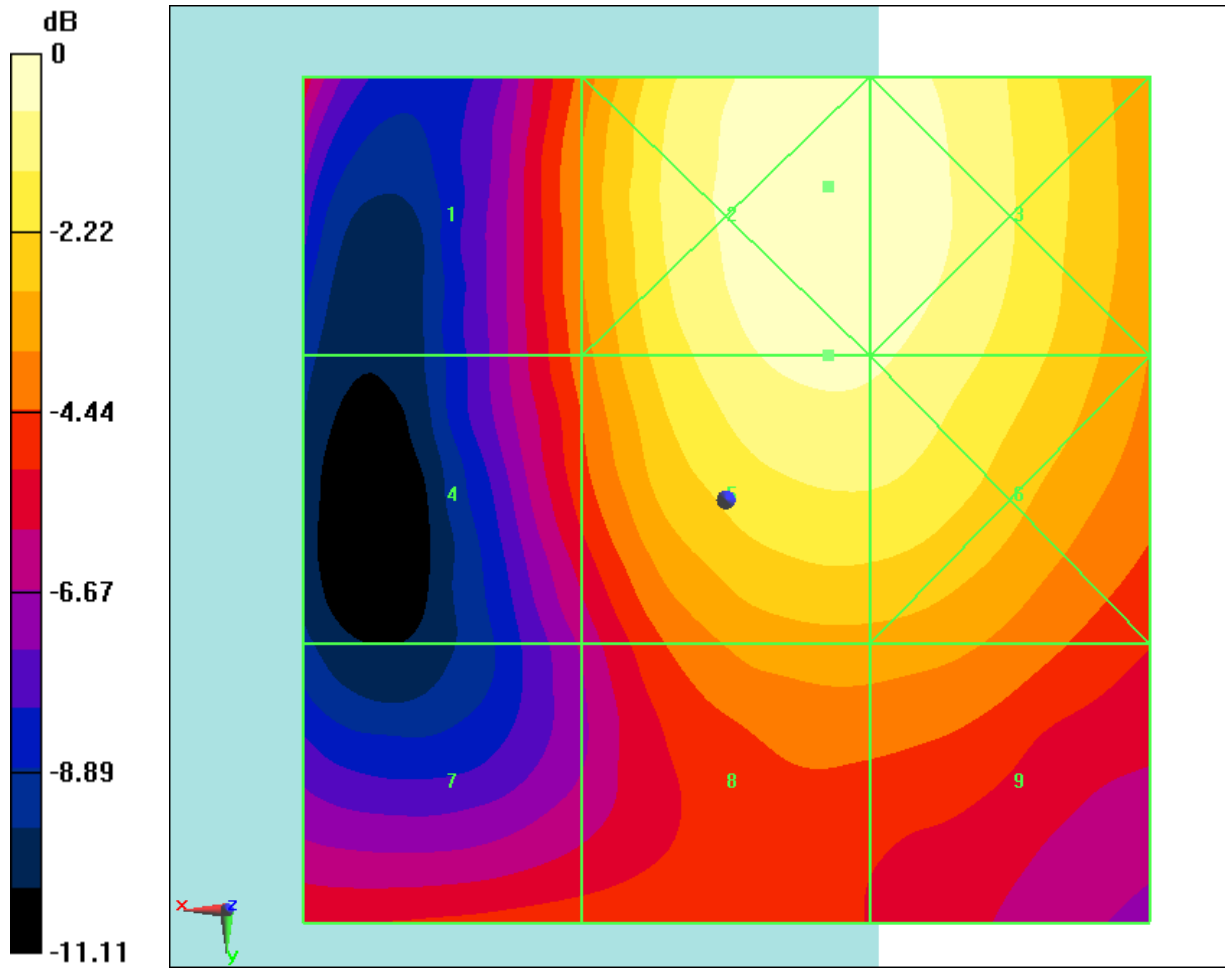
Fig B.21 HAC RF E-Field LTE Band41 Power Class 3 QPSK CH39750
