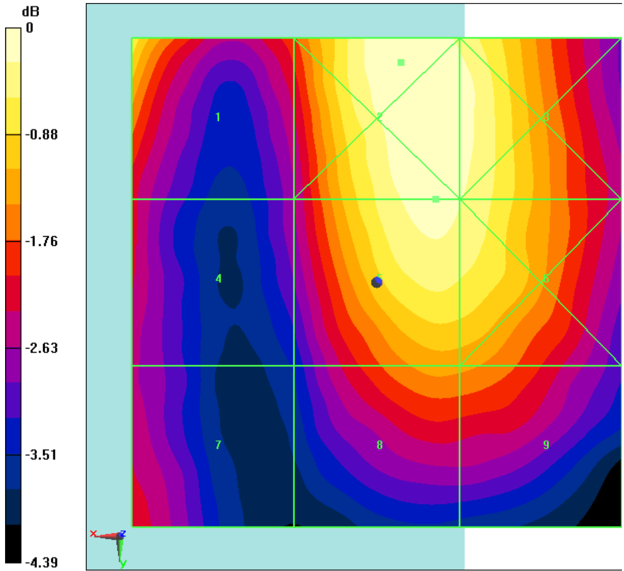
Fig B.23 HAC RF E-Field LTE Band41 Power Class 3 16QAM CH41055
