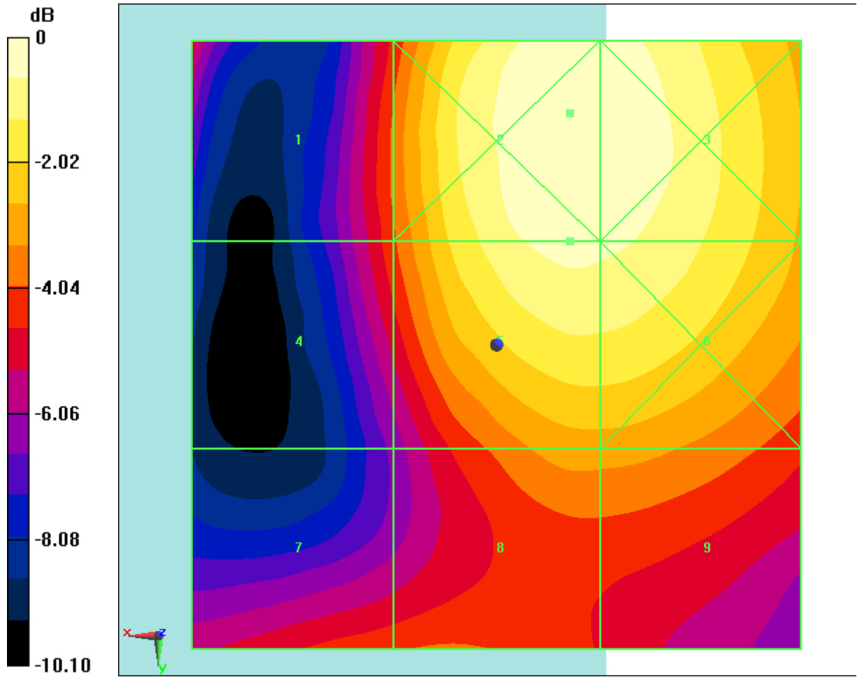
Fig B.20 HAC RF E-Field LTE Band41 Power Class 3 QPSK CH40185
