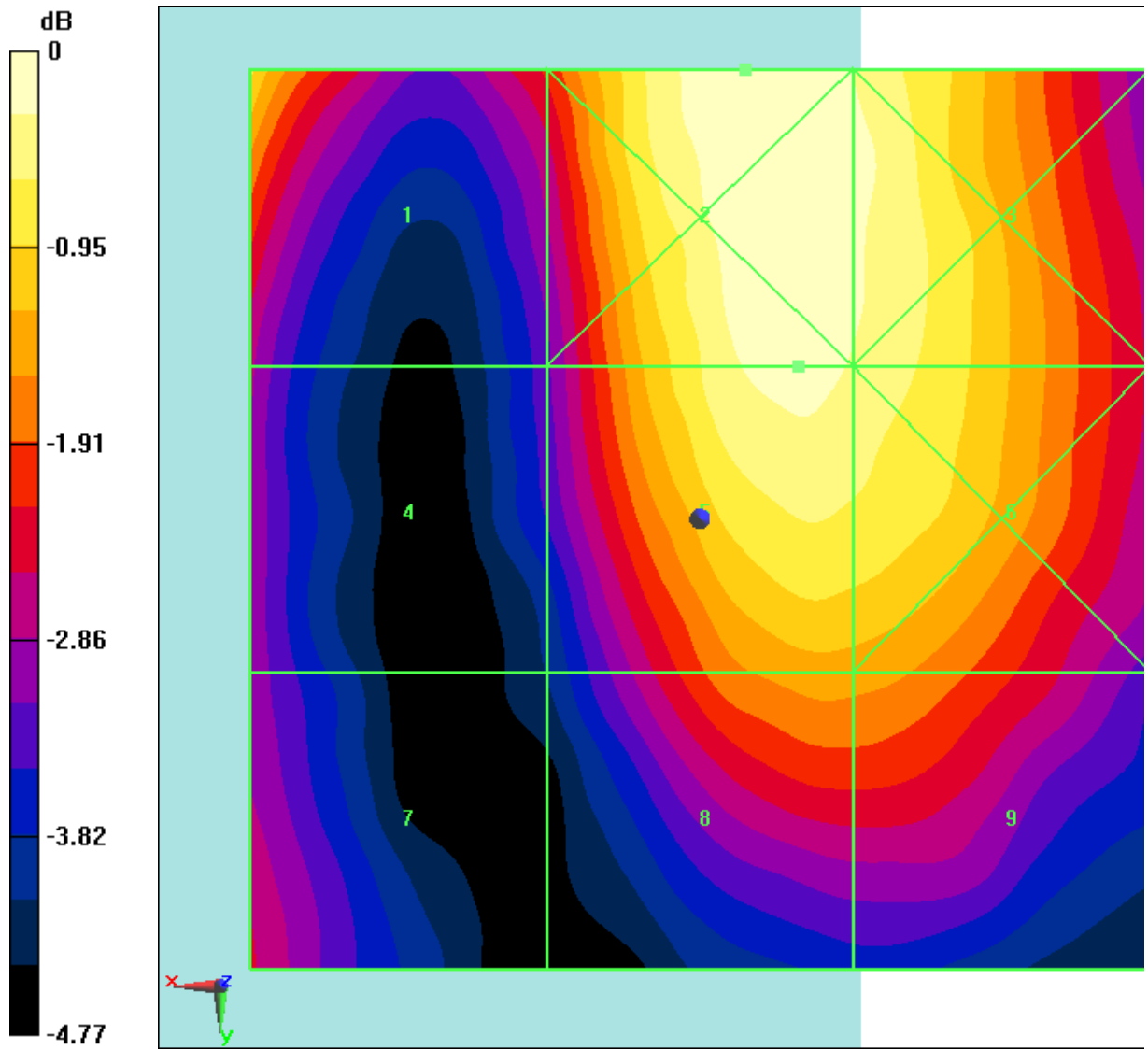
Fig B.13 HAC RF E-Field LTE Band41 Power Class 2 16QAM CH41055
