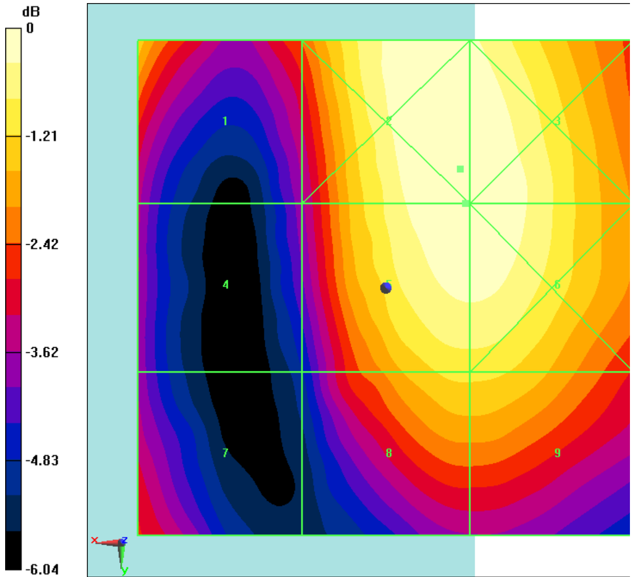
Fig B.24 HAC RF E-Field LTE Band41 Power Class 3 16QAM CH40620
