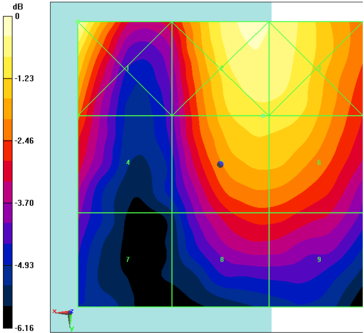
Fig B.7 HAC RF E-Field LTE Band41 Power Class 2 QPSK CH41490
