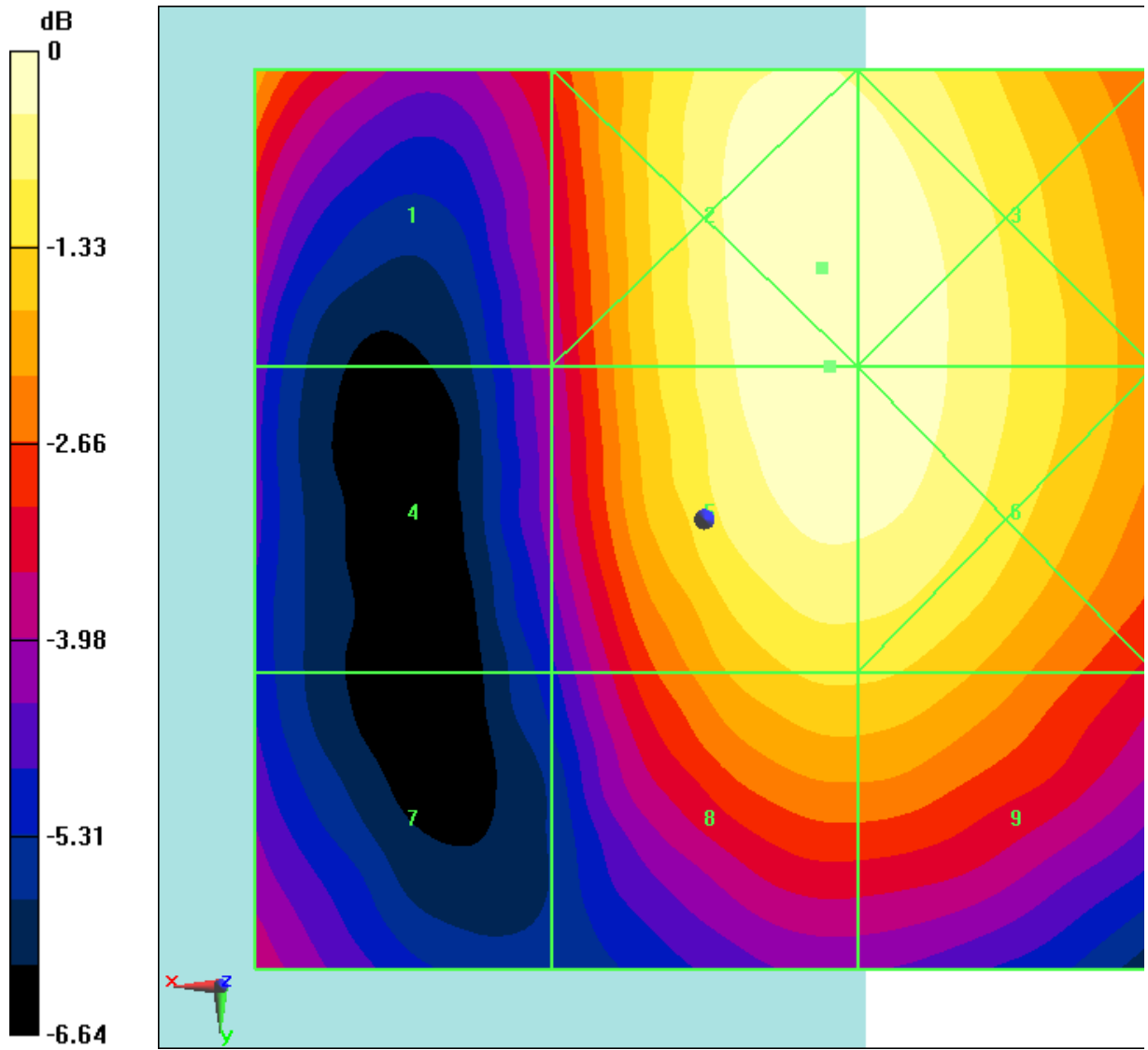
Fig B.15 HAC RF E-Field LTE Band41 Power Class 2 16QAM CH40185
