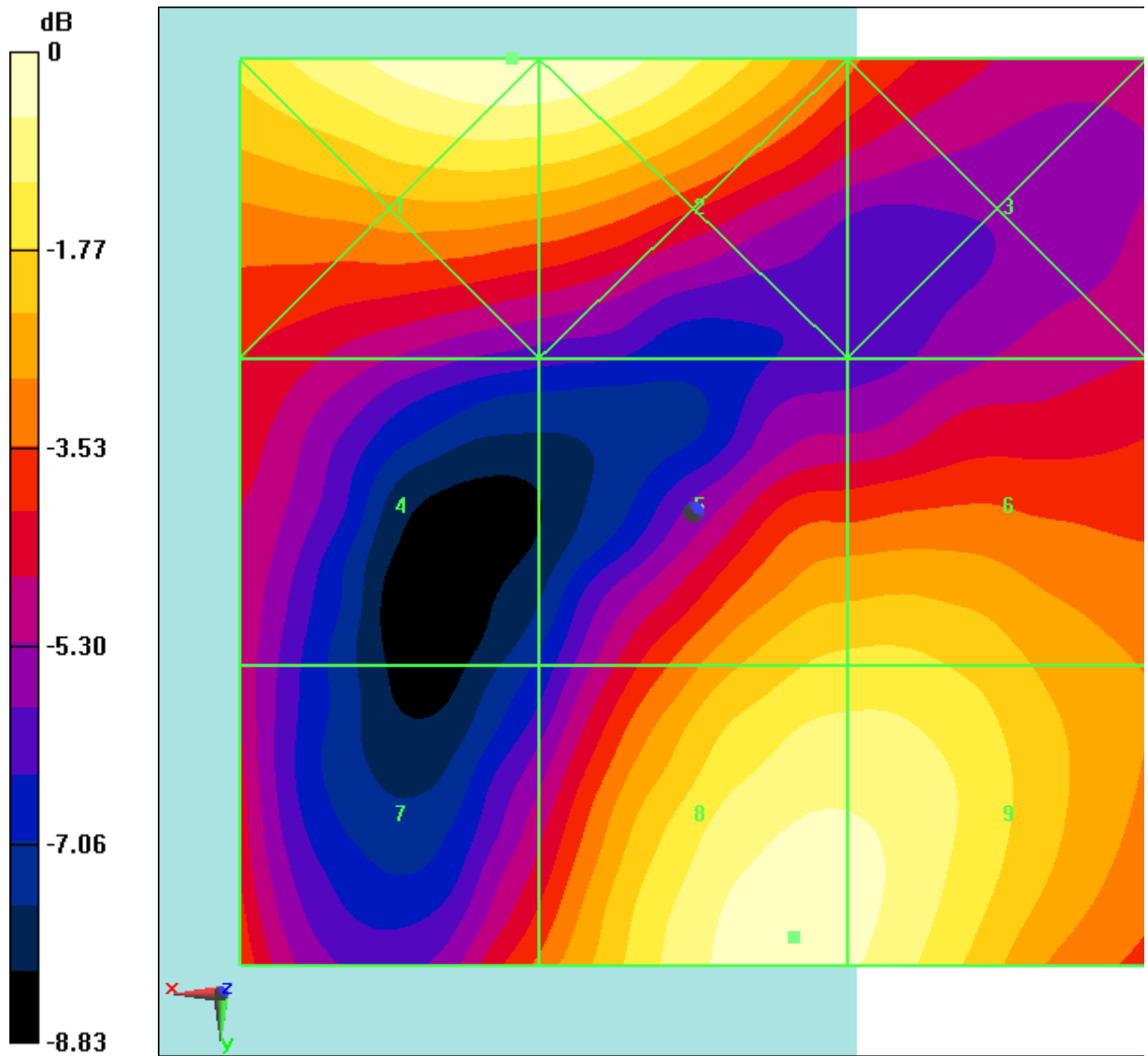
Fig B.19 HAC RF E-Field LTE Band41 Power Class 3 QPSK CH40620
