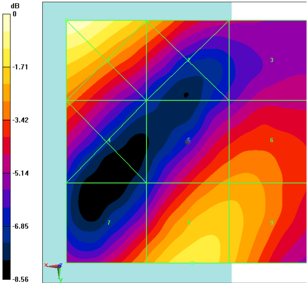
Fig B.21 HAC RF E-Field LTE Band41 Power Class 3 QPSK CH39750
