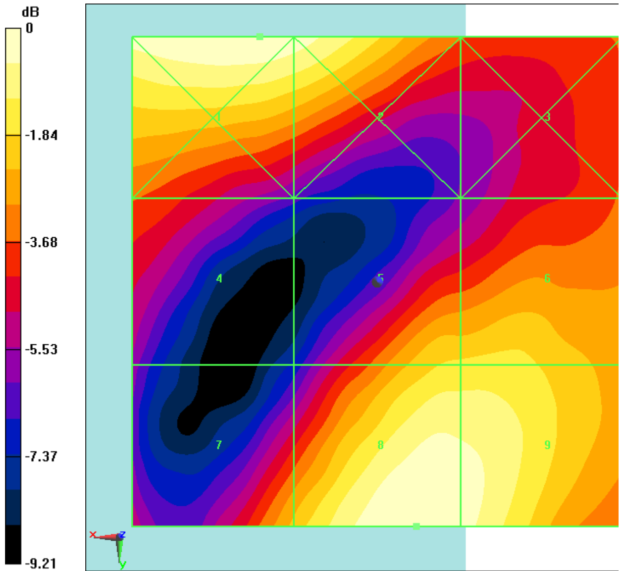
Fig B.20 HAC RF E-Field LTE Band41 Power Class 3 QPSK CH40185
