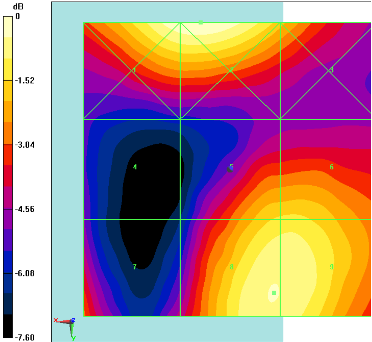
Fig B.18 HAC RF E-Field LTE Band41 Power Class 3 QPSK CH41055
