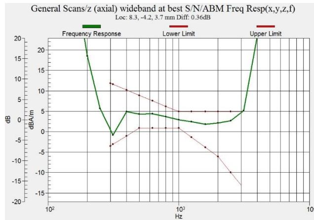
Figure C.16 Frequency Response of W1700 - OTT VoIP
