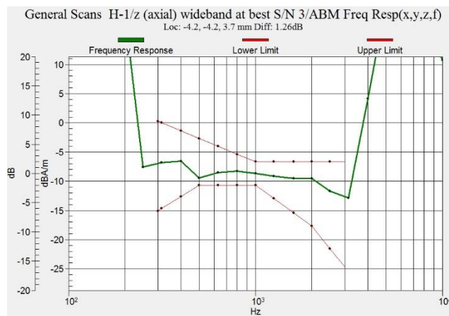
Figure C.18 Frequency Response of LTE B41 Power Class 3 - OTT VoIP
