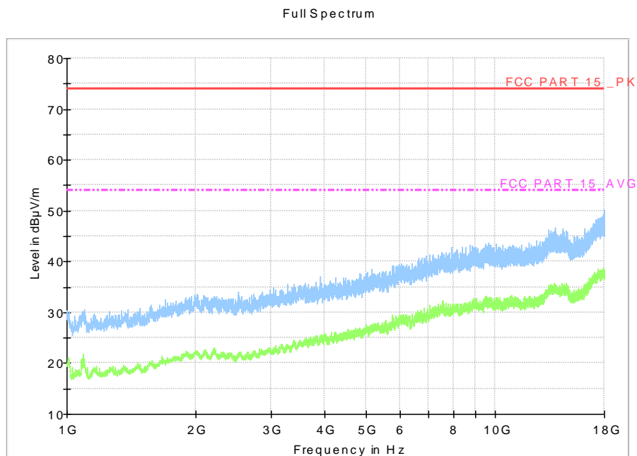
Fig A.5 Radiated Emission from 1GHz to 18GHz
