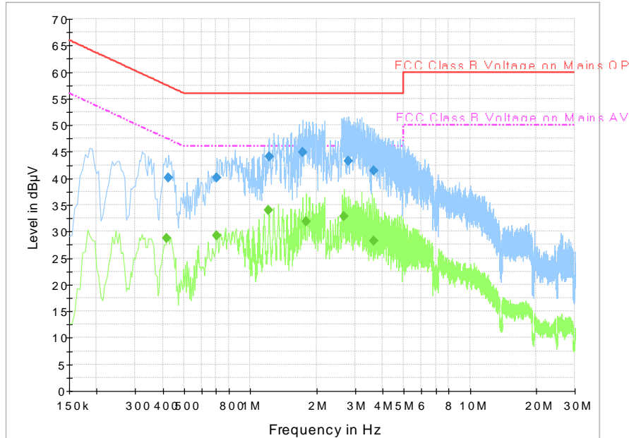
Fig A.18 Conducted Emission
