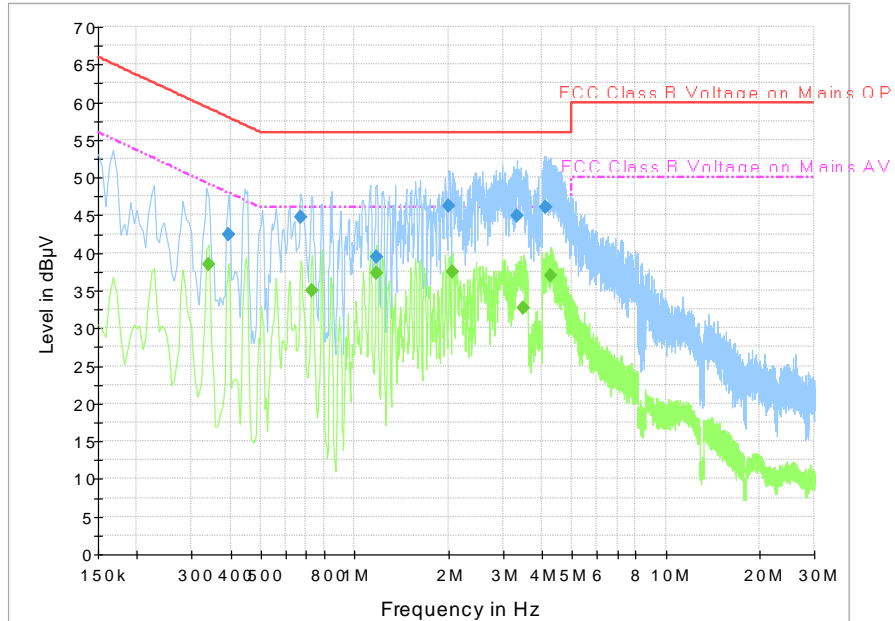
Fig A.17 Conducted Emission
