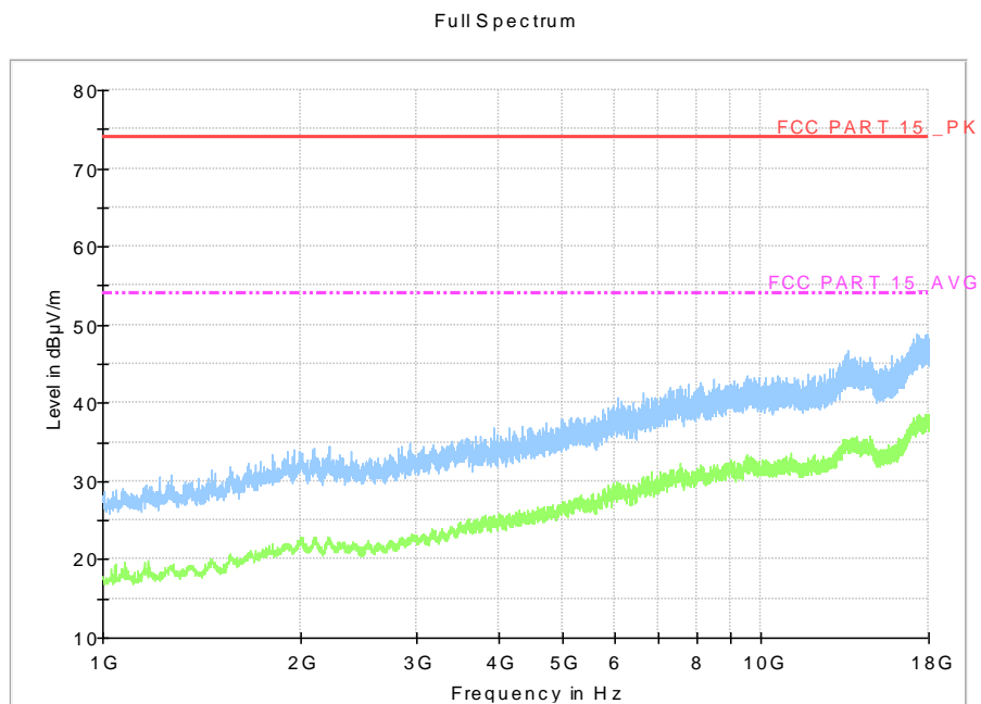
Fig A.9 Radiated Emission from 1GHz to 18GHz
