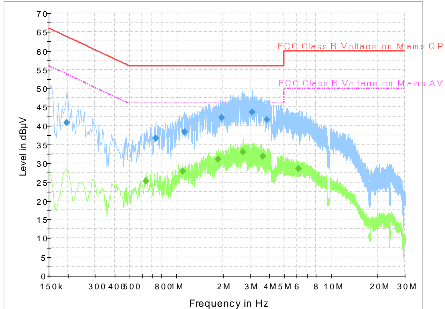
Fig A.16 Conducted Emission
