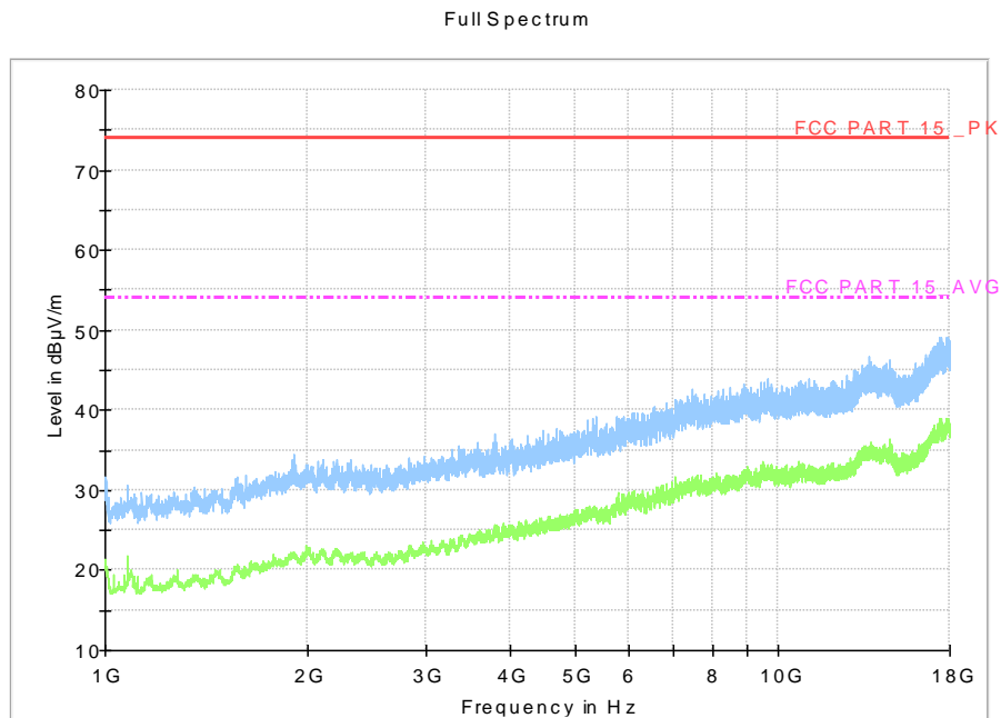
Fig A.7 Radiated Emission from 1GHz to 18GHz
