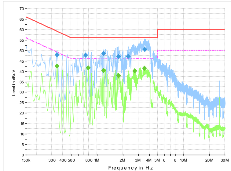
Fig A.15 Conducted Emission
