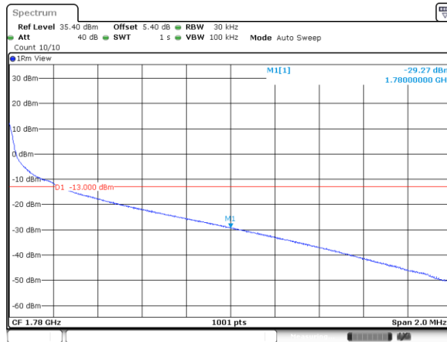
Band66_20MHz_QPSK_132572_100RB#0
