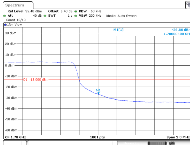
Band66_5MHz_QPSK_132647_25RB#0
