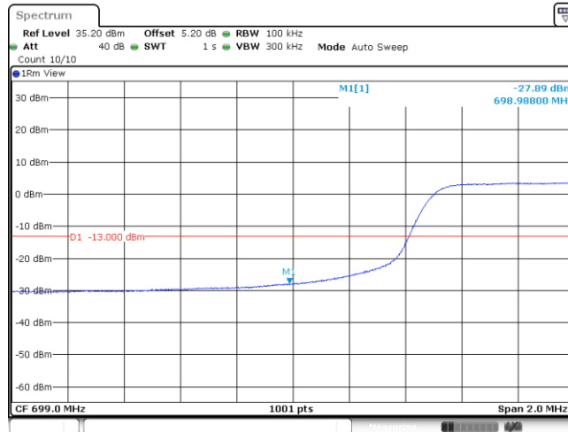
Band12_10MHz_16QAM_23060_50RB#0
