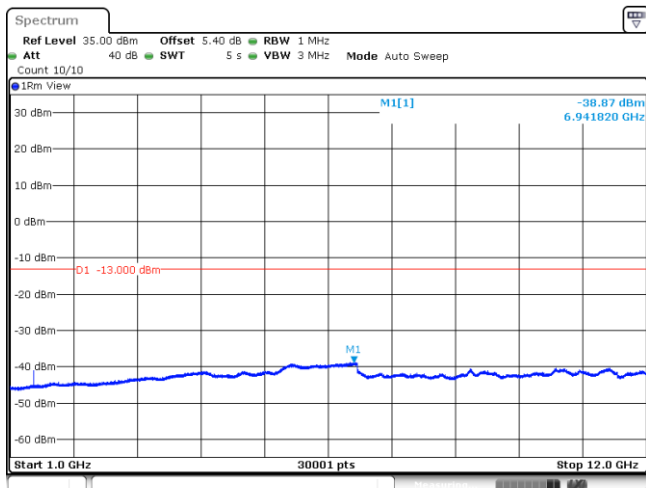
Band12_10MHz_16QAM_23095_1RB#0
