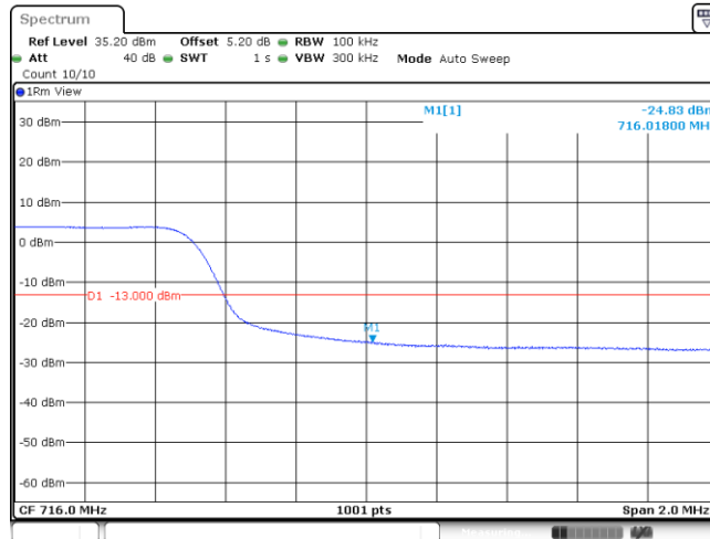
Band12_10MHz_QPSK_23130_50RB#0
