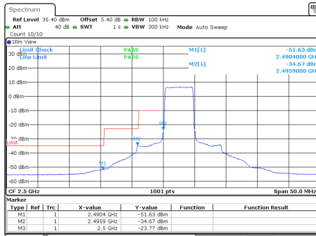
Band7_5MHz_QPSK_20775_25RB#0
