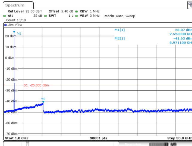
Band7_20MHz_16QAM_21100_1RB#0
