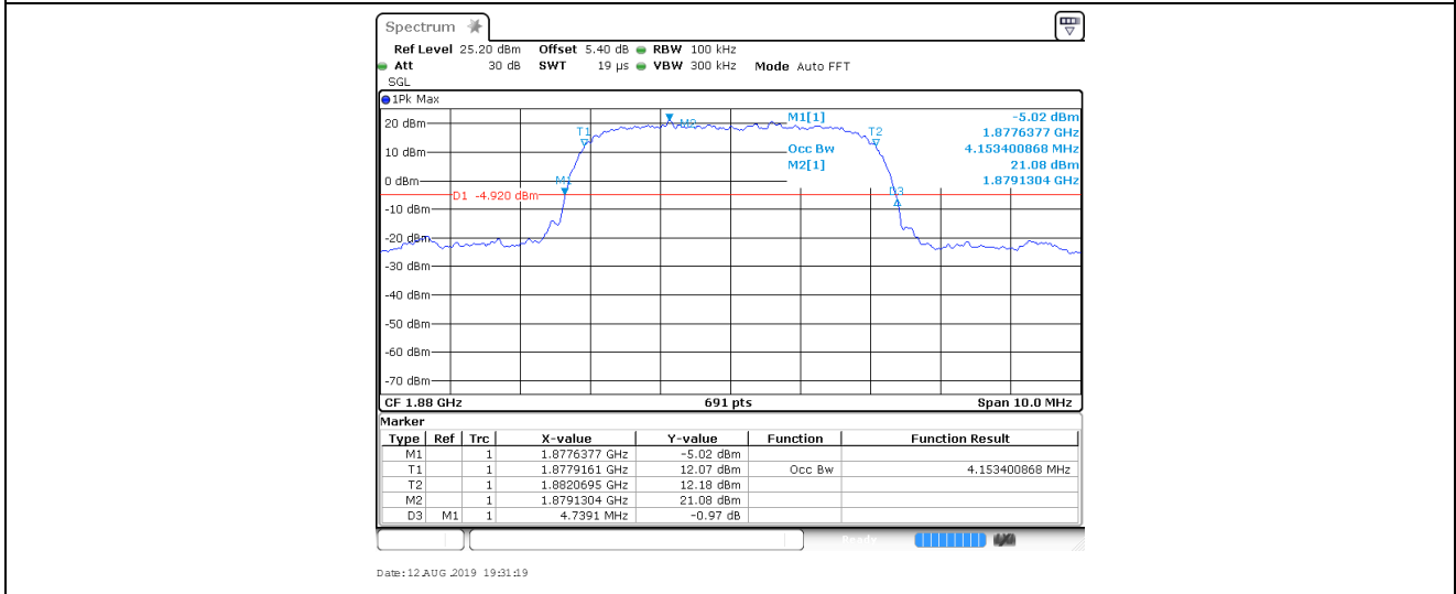
BAND II_QPSK_9400
