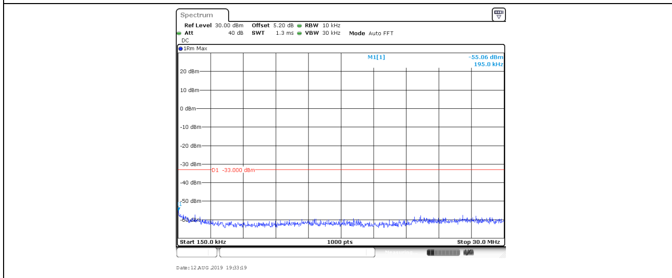
BAND II_QPSK_9262
