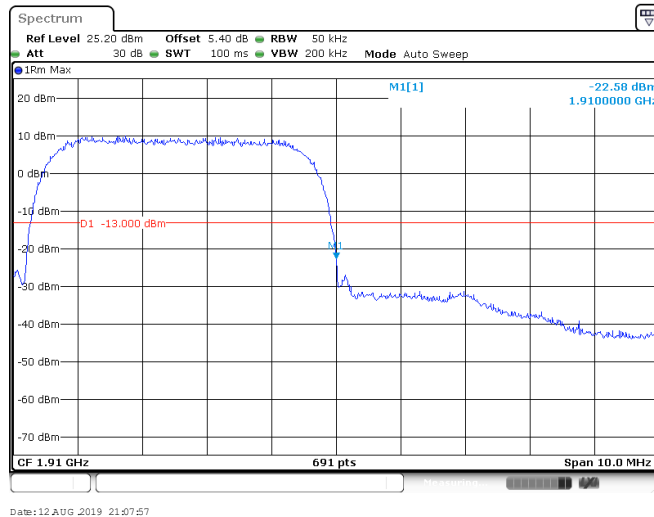
BAND II_16QAM_9538
