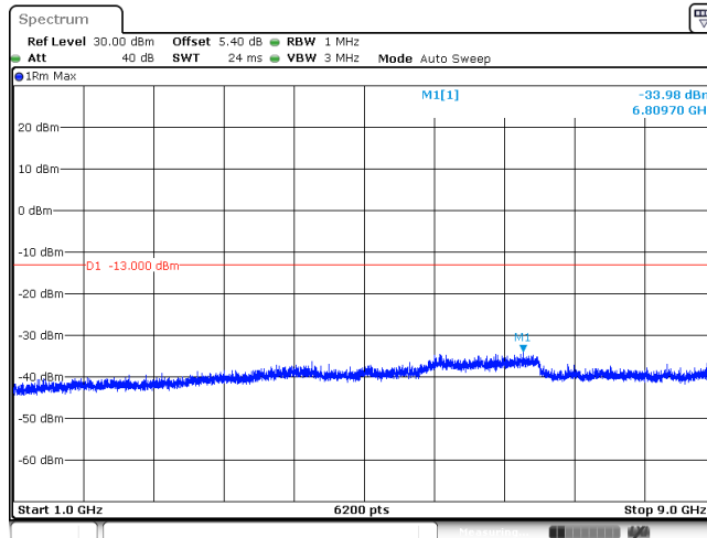
BAND V_QPSK_4233
