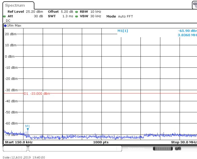
BAND V_QPSK_4132
