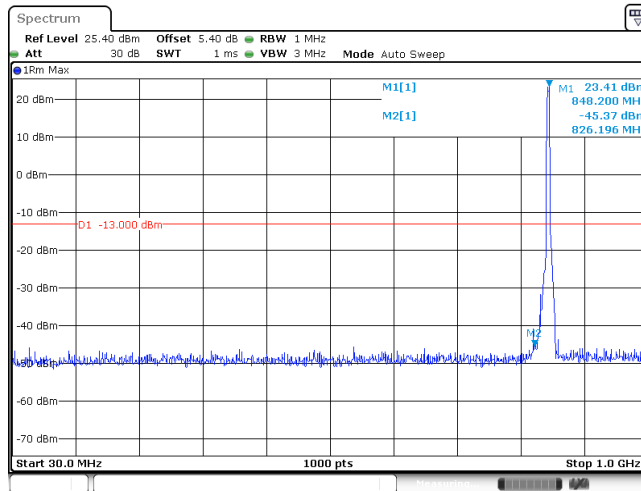
BAND V_QPSK_4233
