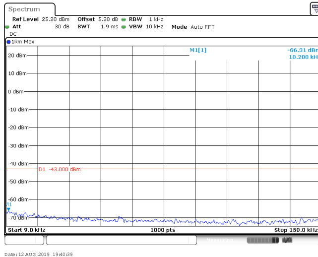
BAND V_QPSK_4132
