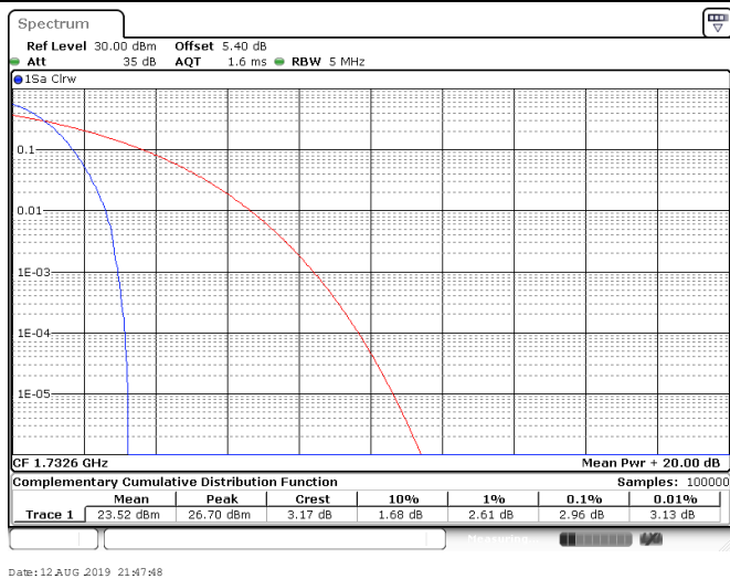
BAND IV_QPSK_1513
