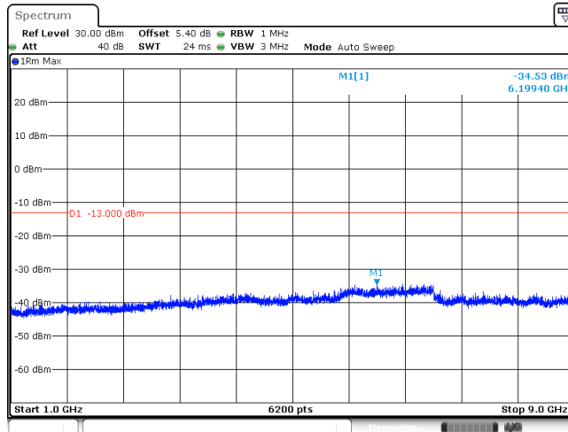
BAND V_QPSK_4182
