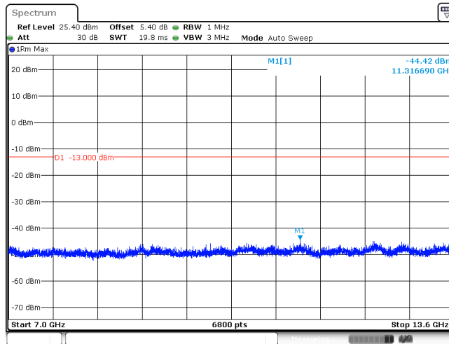
BAND IV_QPSK_1513
