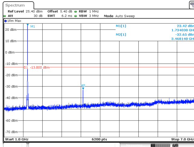
BAND IV_QPSK_1413
