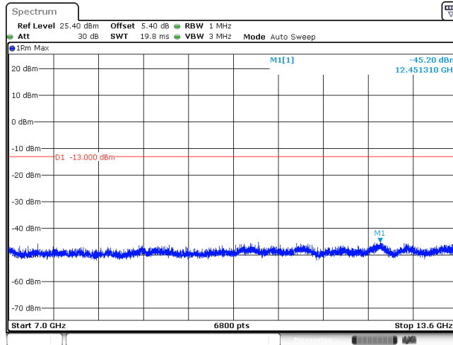
BAND IV_QPSK_1413
