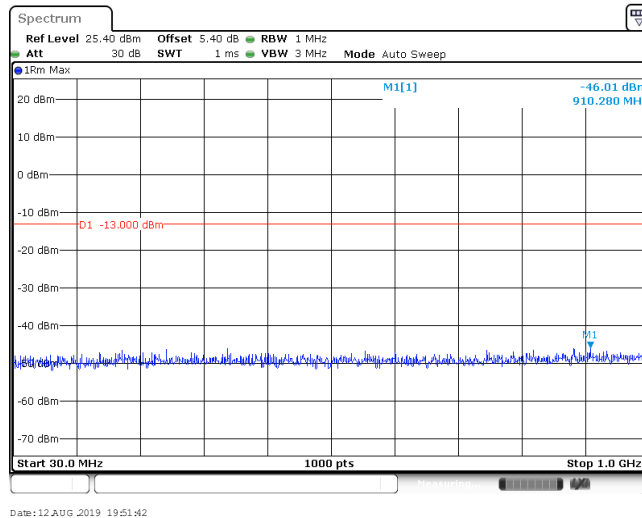
BAND IV_QPSK_1312
