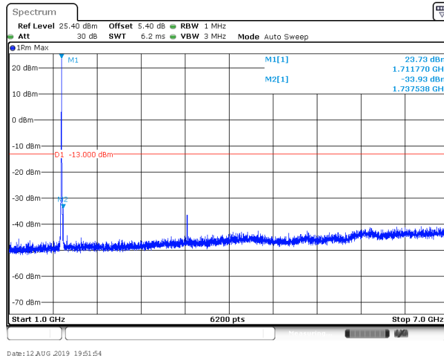
BAND IV_QPSK_1312
