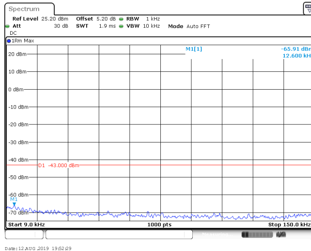
BAND IV_QPSK_1413
