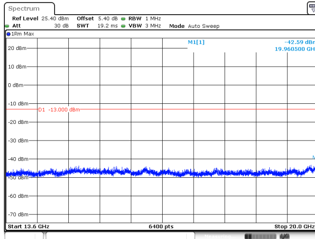
BAND II_QPSK_9262
