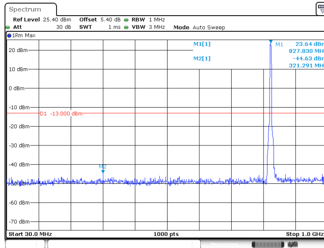
BAND V_QPSK_4132
