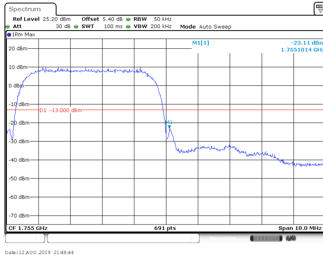
BAND IV_QPSK_1513
