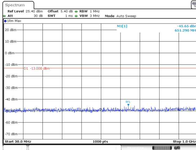
BAND IV_QPSK_1513
