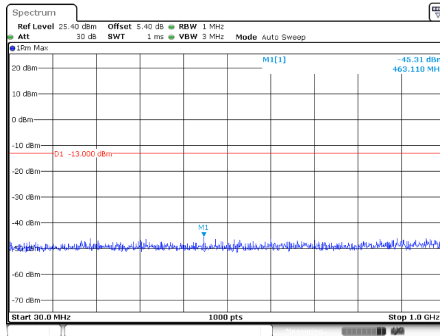
BAND IV_QPSK_1413
