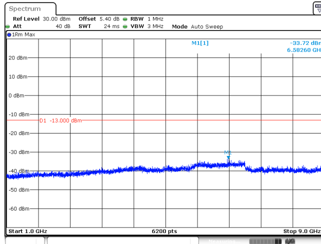
BAND V_QPSK_4132
