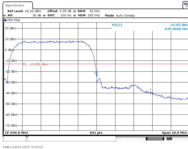
BAND V_16QAM_4233
