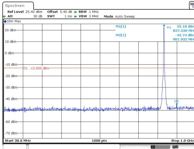
BAND V_QPSK_4182
