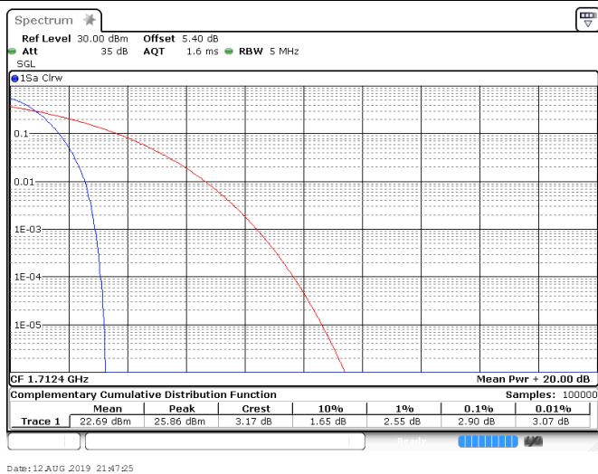
BAND IV_QPSK_1413
