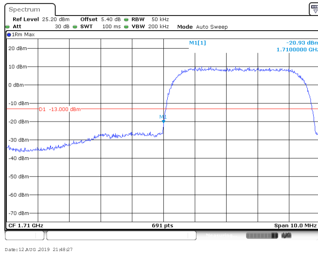
BAND IV_QPSK_1312
