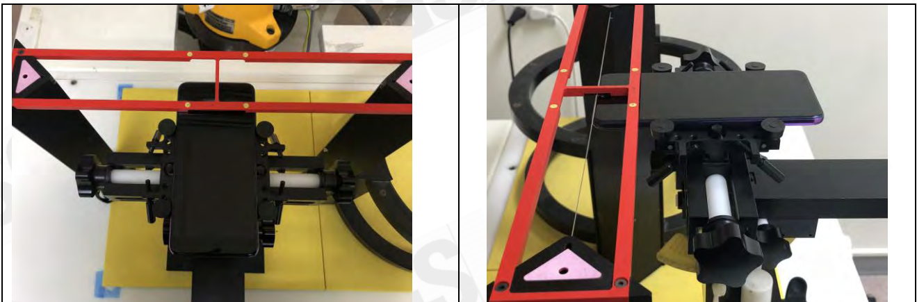
Fig. 1 Photograph of the DASY 5 measurement system
