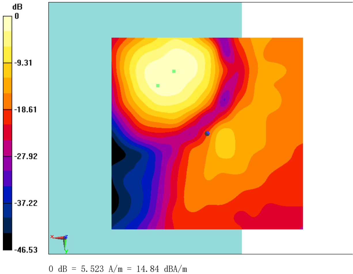
Fig B.24 T-Coil WiFi-2.4G
