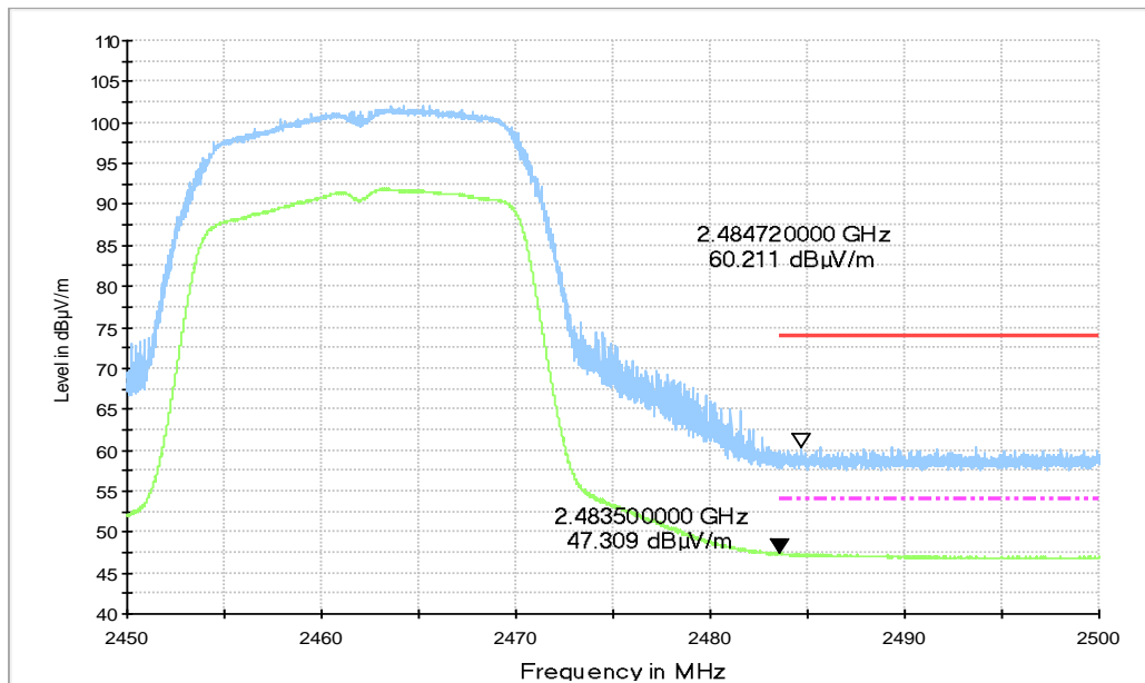
RE - Power-2.45GHz-2.5GHz
