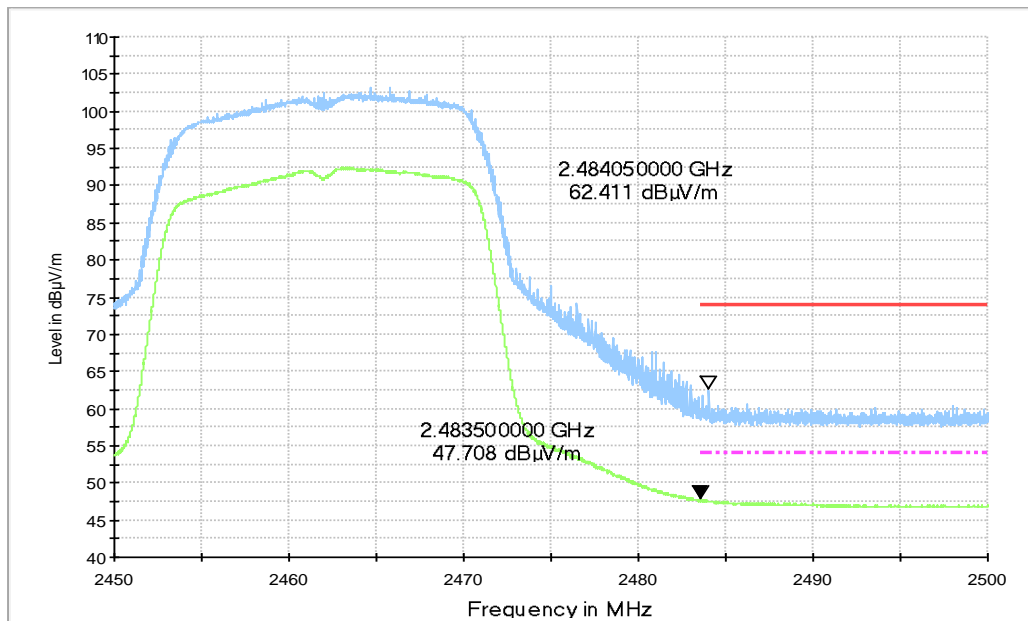
RE - Power-2.45GHz-2.5GHz
