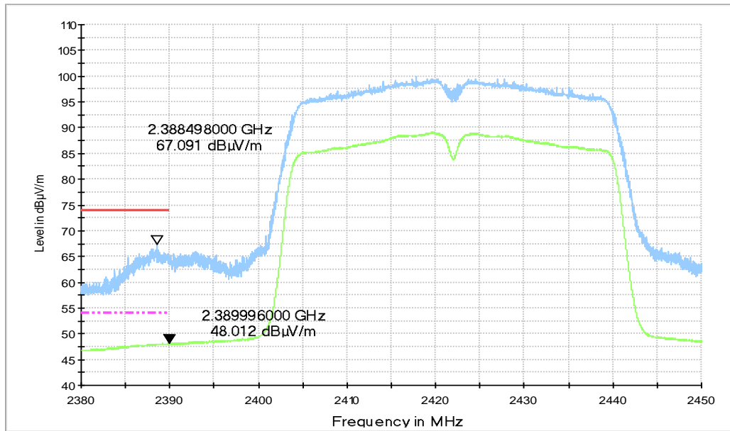
RE - Power-2.38GHz-2.45GHz
