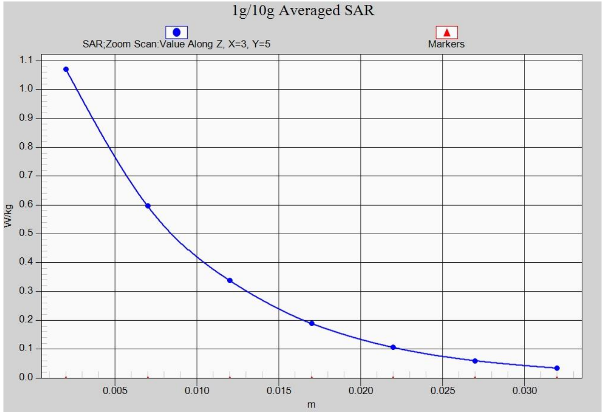
Fig. 25-1 Z-Scan at power reference point (LTE Band30)
