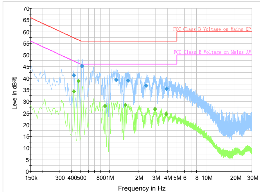
Fig.A.7.2 AC Powerline Conducted Emission-802.11b
