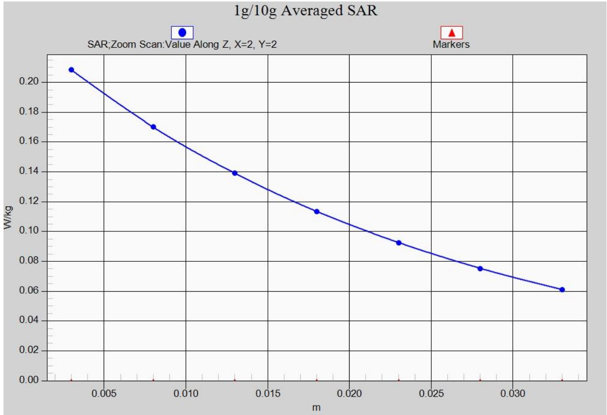
Fig. 25-1 Z-Scan at power reference point (LTE Band71)
