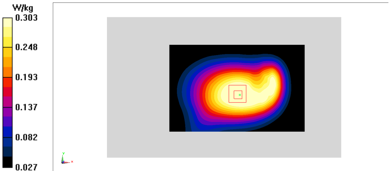
Fig.26 LTE Band71
