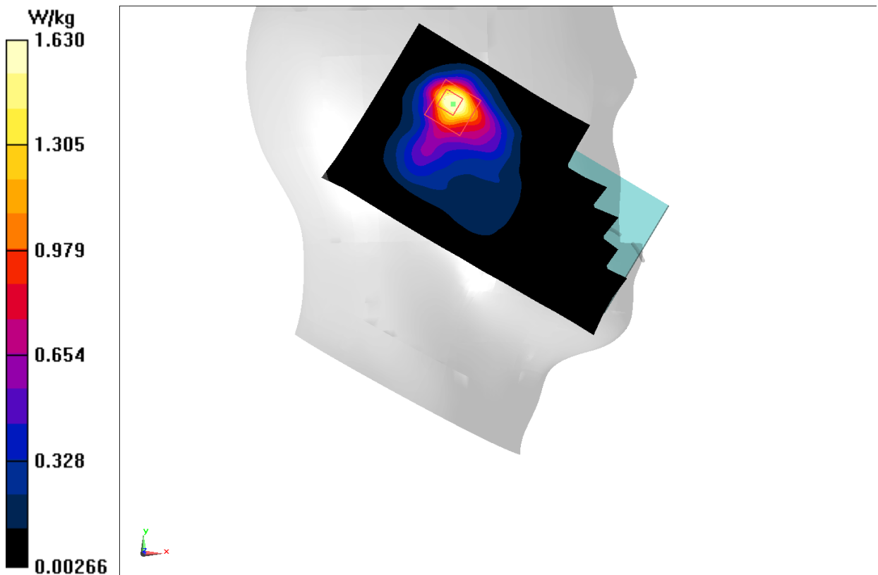
Fig.27 2450 MHz
