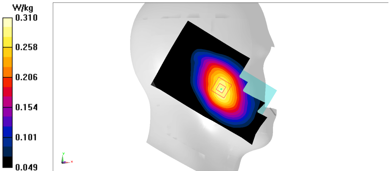
Fig.18 LTE Band12
