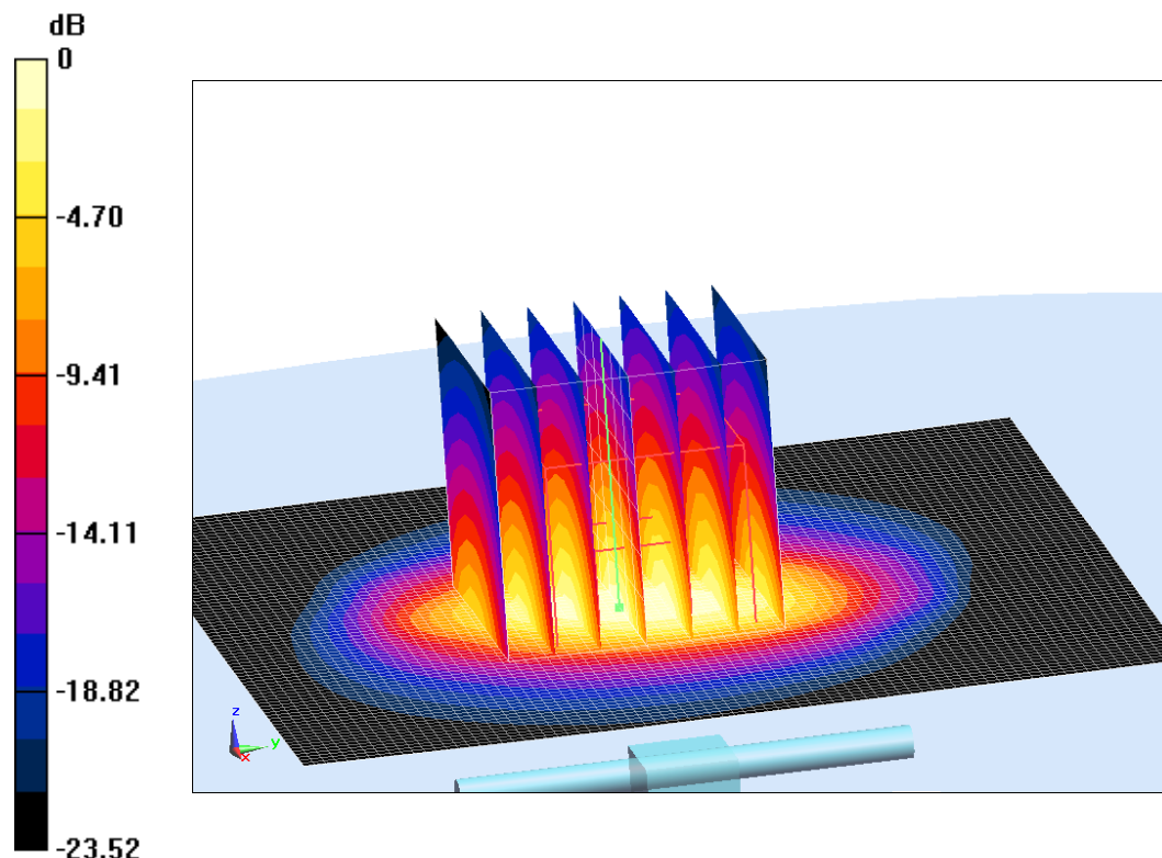
Fig.B.15 validation 2600 MHz 250mW
