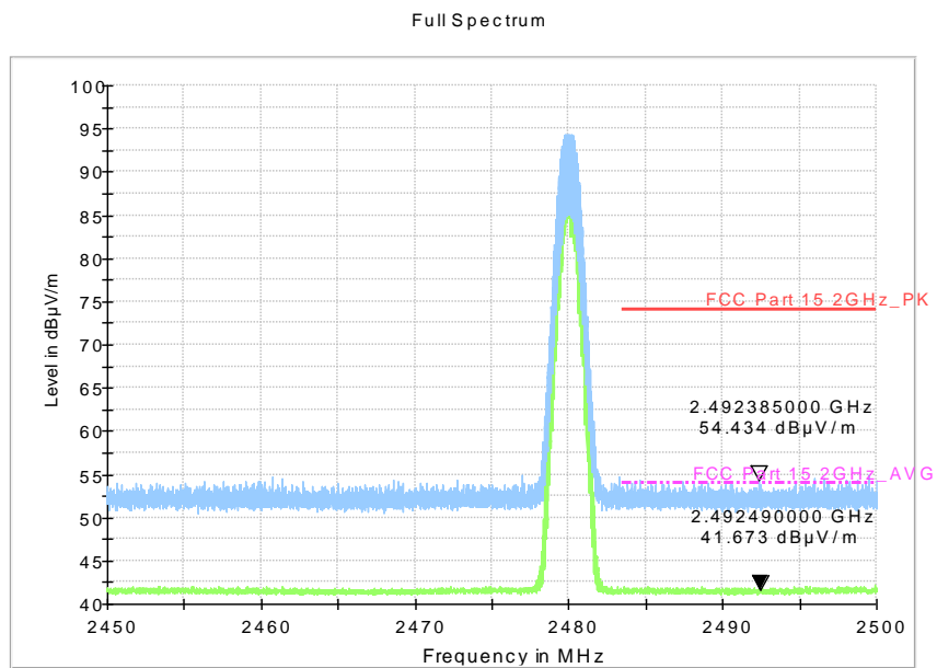
Fig.59. Radiated emission (Power) GFSK, high channel
