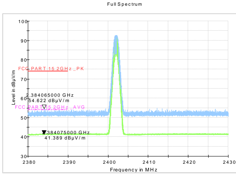
Fig.58. Radiated emission (Power): GFSK, low channel
