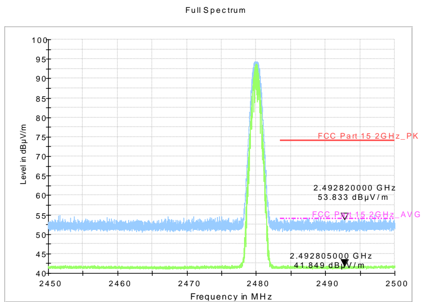
Fig.63. Radiated emission (Power): 8DPSK, high channel
