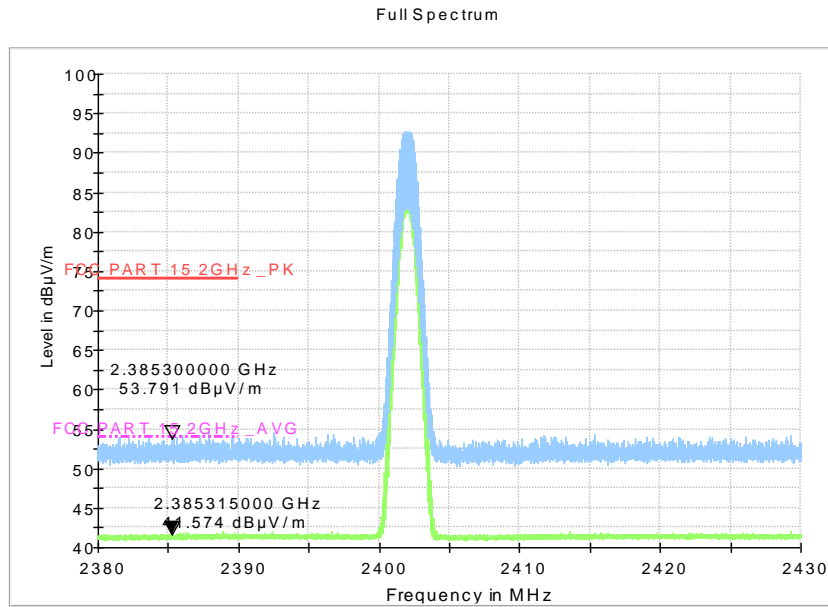
Fig.60. Radiated emission (Power): \pi/4 DQPSK, low channel
