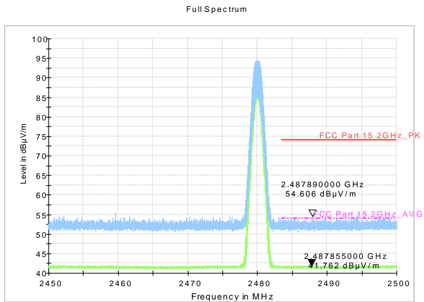
Fig.61. Radiated emission (Power): \pi/4 DQPSK, high channel
