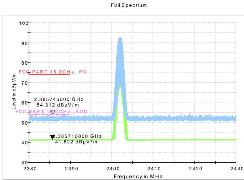
Fig.62. Radiated emission (Power): 8DPSK, low channel
