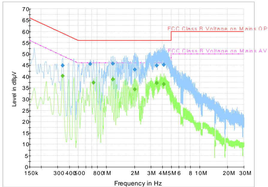
Fig.A.7.3 AC Power line Conducted Emission-802.11b
