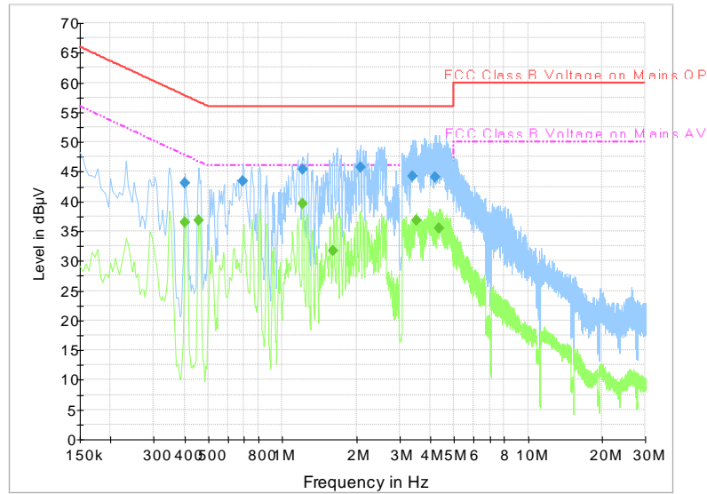
Fig.A.7.5 AC Power line Conducted Emission-802.11b
