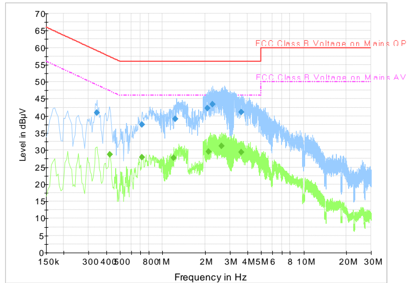
Fig.A.7.4 AC Power line Conducted Emission-802.11b
