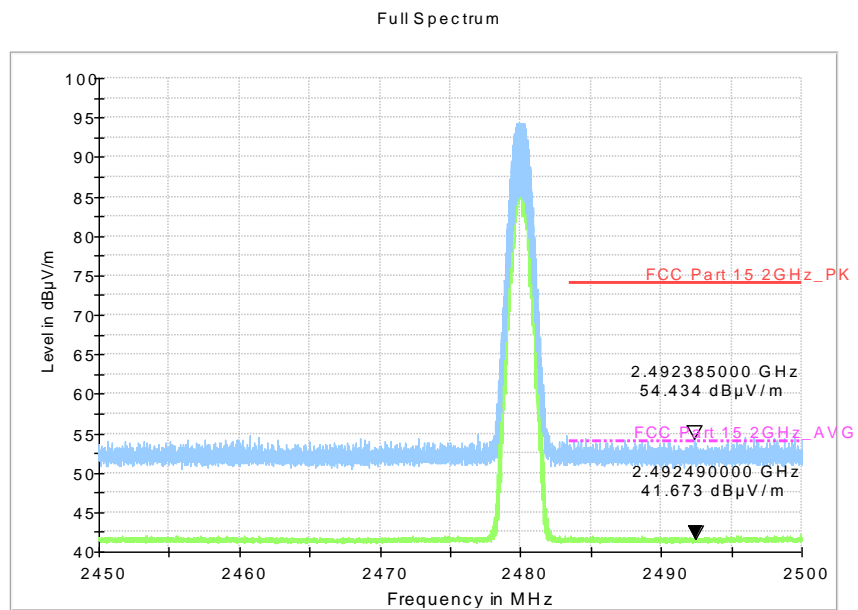
Fig.59. Radiated emission (Power) GFSK, high channel
