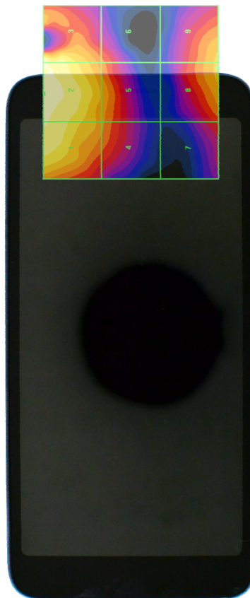
Figure 17-4 E-Field WD Scan overlay
