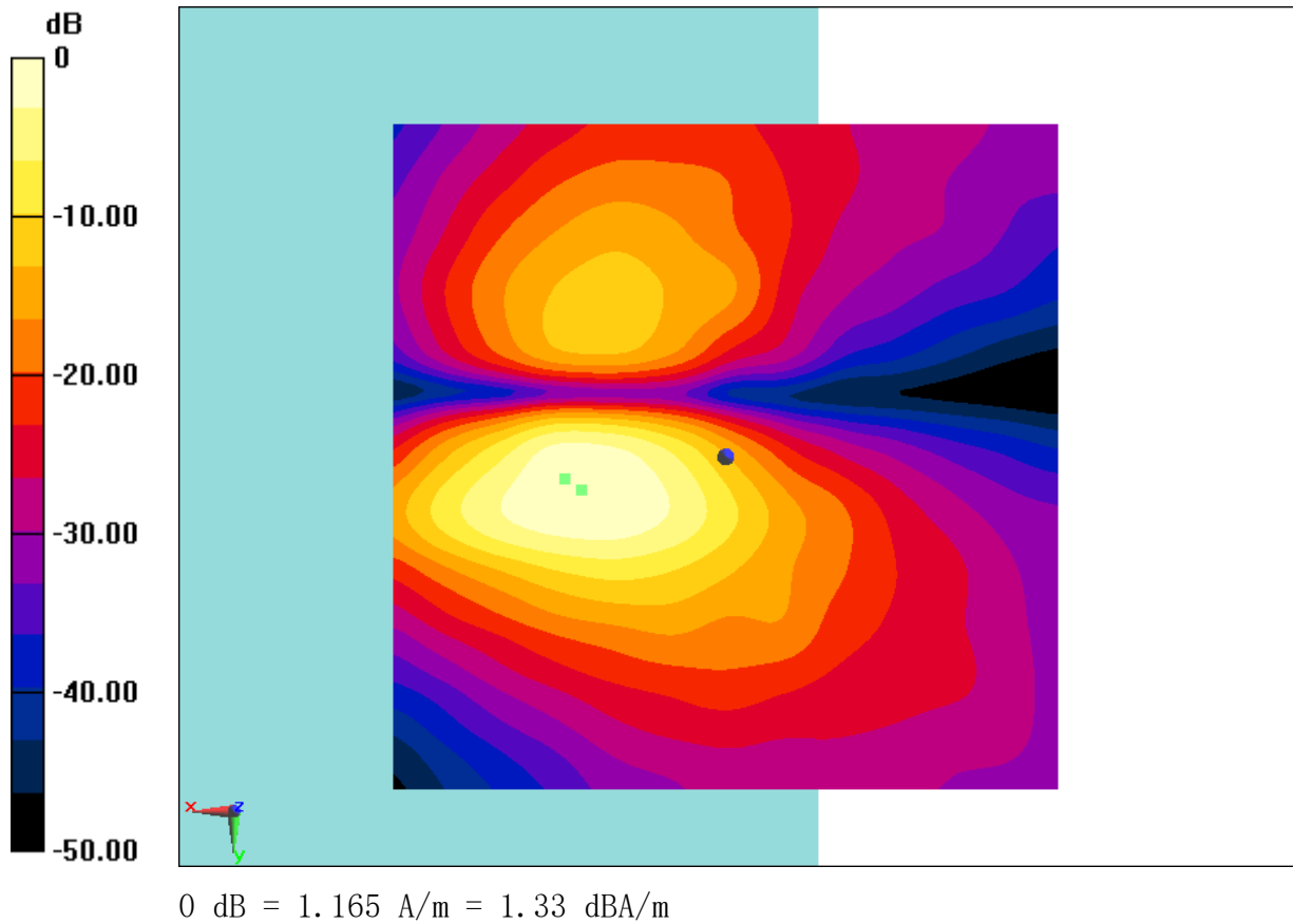
Fig B.19 T-Coil LTE B71
