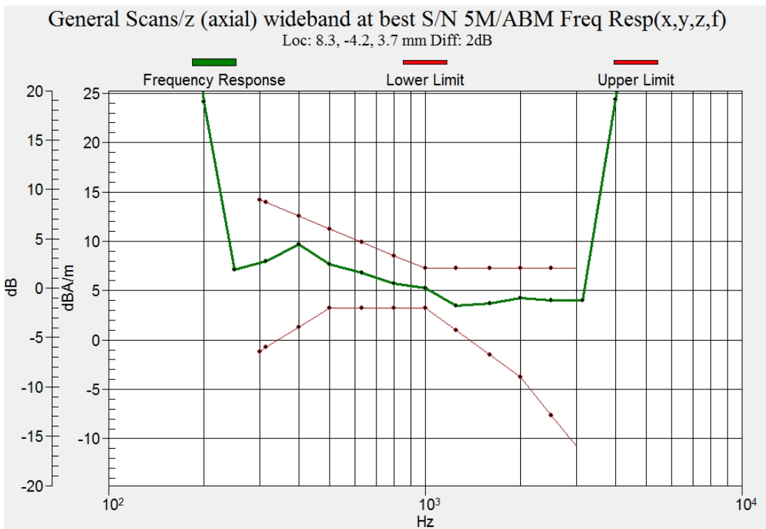
Figure C.8 Frequency Response of LTE B12
