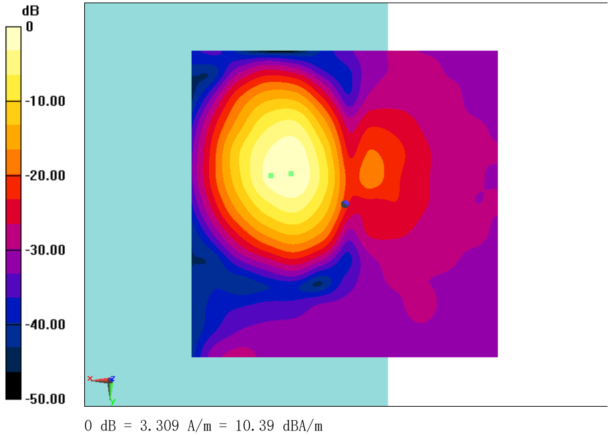
Fig B.20 T-Coil LTE B71
