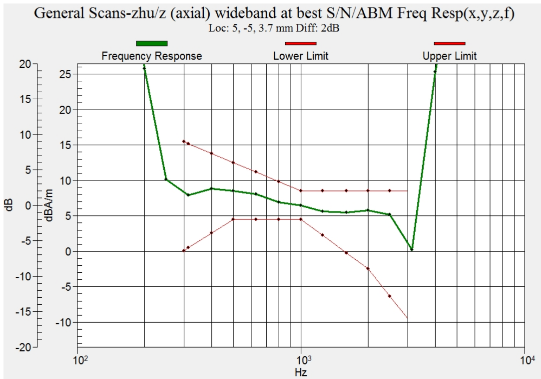
Figure C.11 Frequency Response of WiFi-2.4G
