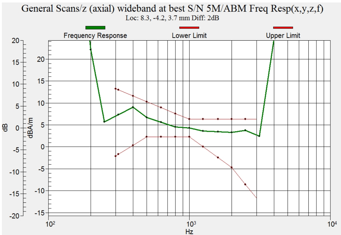
Figure C.10 Frequency Response of LTE B71
