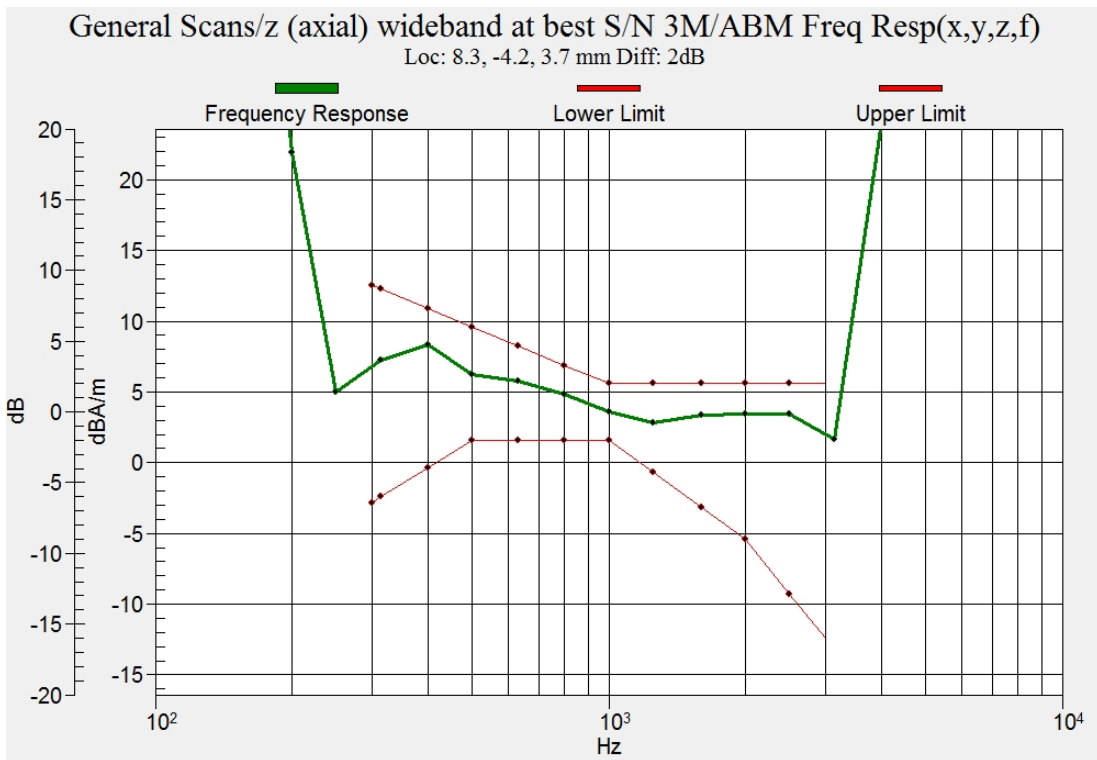
Figure C.9 Frequency Response of LTE B66
