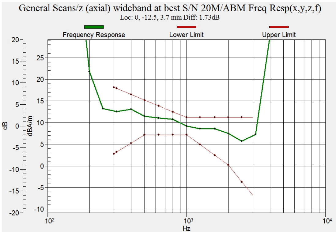
Figure C.11 Frequency Response of LTE B71
