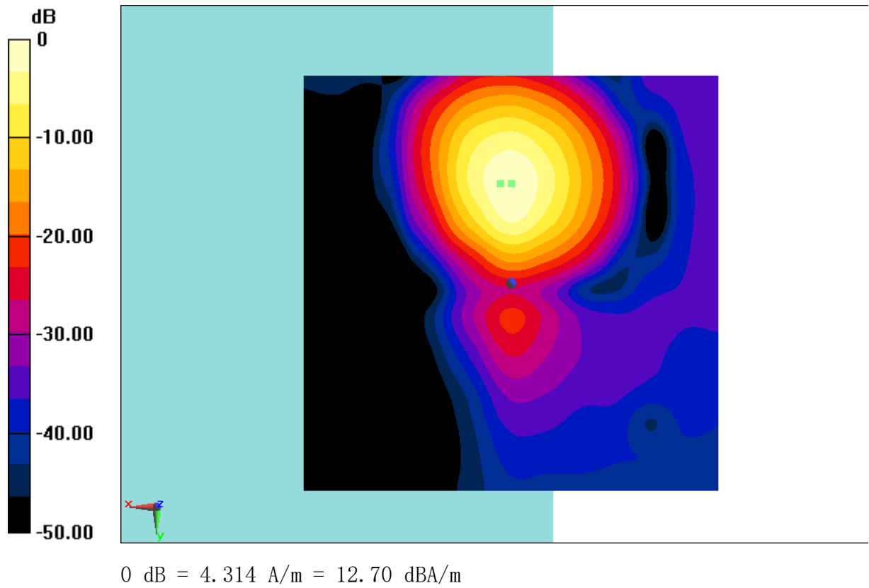
Fig B.10 T-Coil WCDMA 1700
