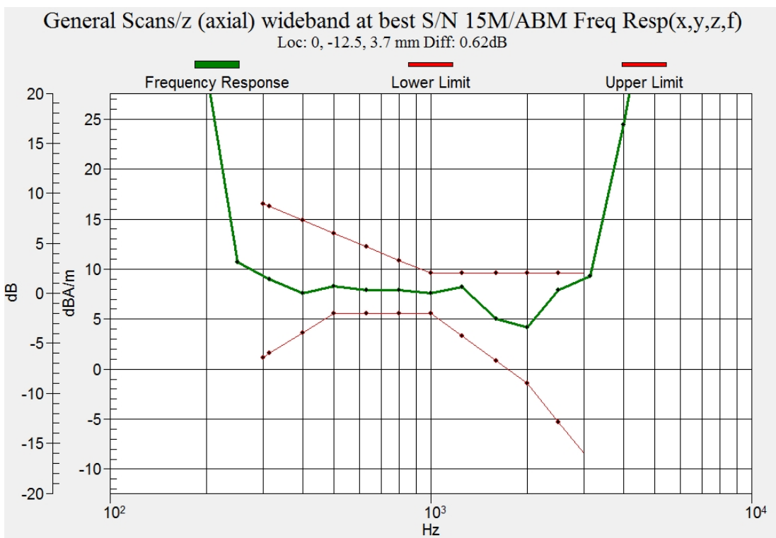
Figure C.10 Frequency Response of LTE B66
