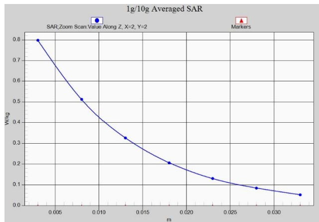
Fig.A.1- 15 Z-Scan at power reference point (LTE Band2)
