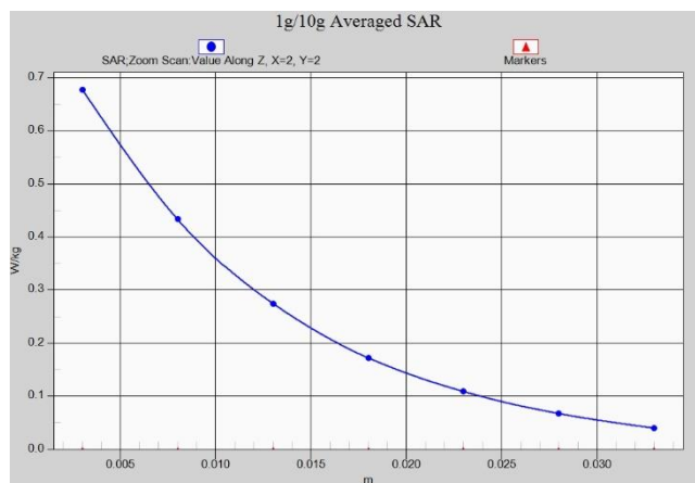
Fig.A.1- 12 Z-Scan at power reference point (W1900)
