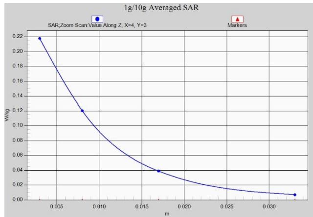
Fig.A.1- 29 Z-Scan at power reference point (WLAN)
