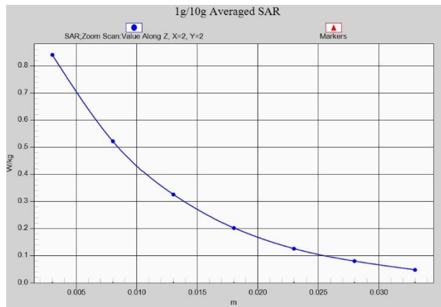
Fig.A.1- 13 Z-Scan at power reference point (W1900)
