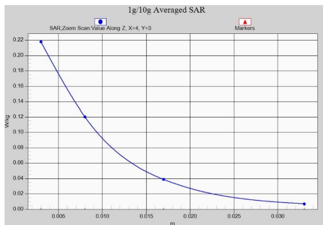
Fig.A.1- 30 Z-Scan at power reference point (WLAN)
