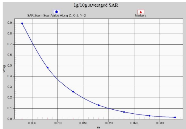
Fig.A.1- 21 Z-Scan at power reference point (LTE Band7)
