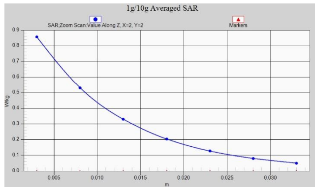
Fig.A.1- 16 Z-Scan at power reference point (LTE Band2)
