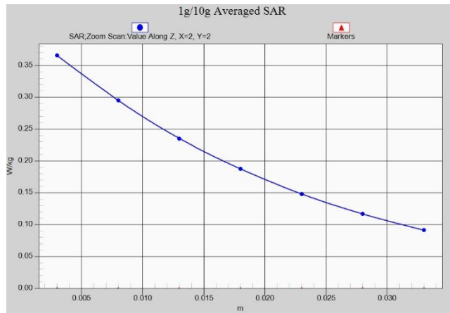
Fig.A.1- 27 Z-Scan at power reference point (LTE Band71)
