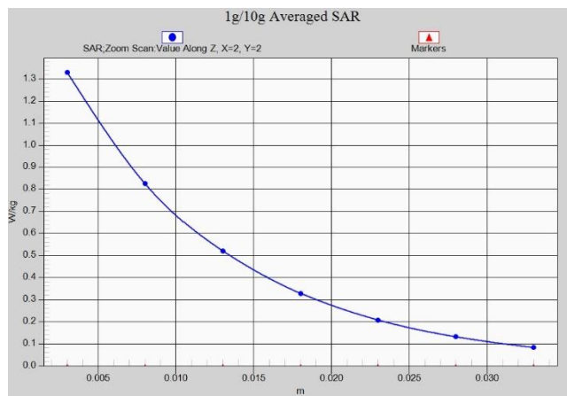
Fig.A.1- 26 Z-Scan at power reference point (LTE Band66)
