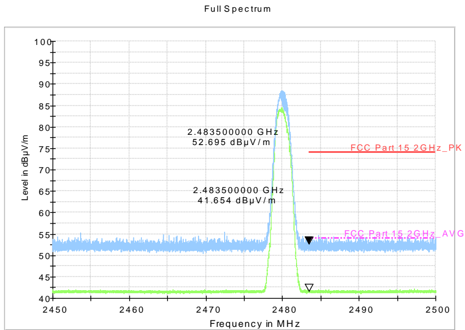
Fig.63. Radiated emission (Power): 8DPSK, high channel
