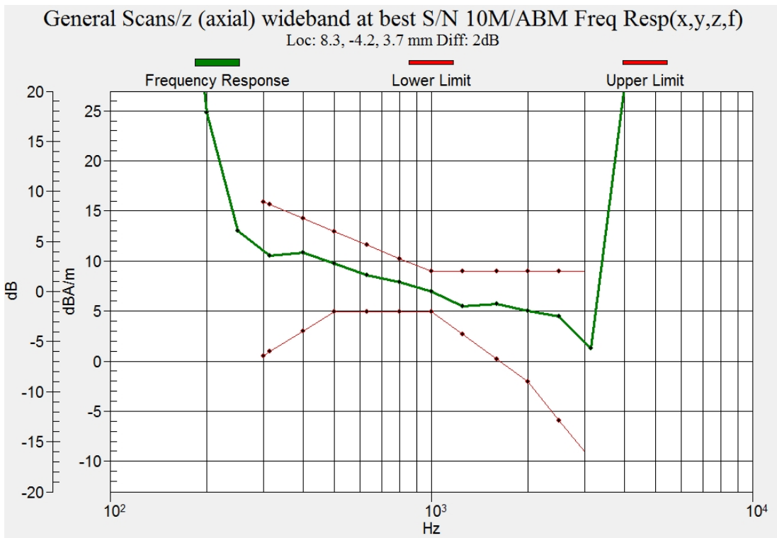
Figure C.10 Frequency Response of LTE B14
