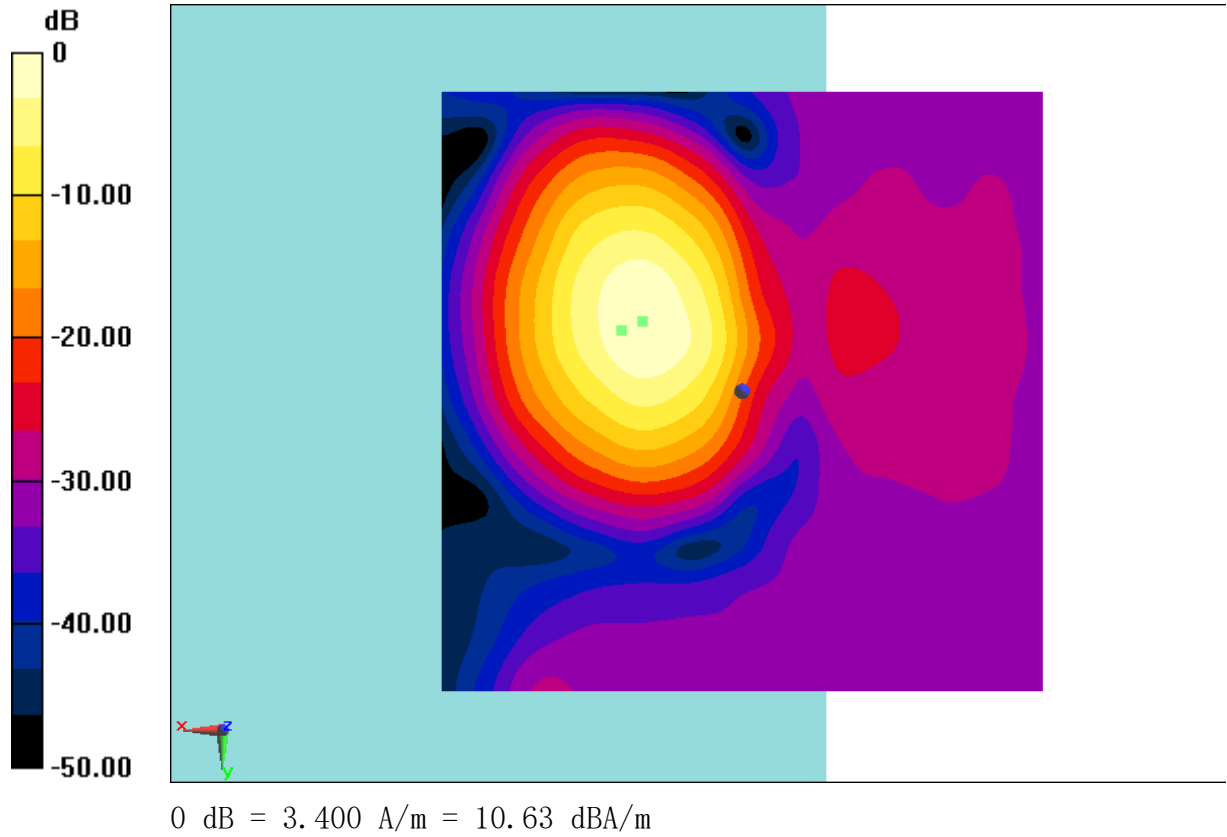
Fig B.18 T-Coil LTE B12
