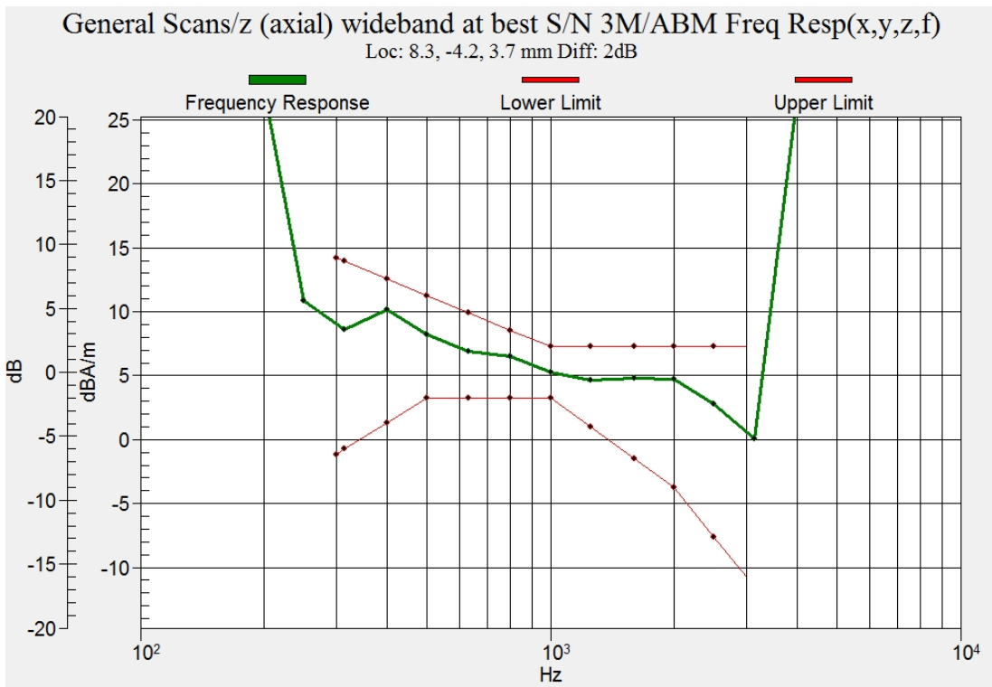
Figure C.7 Frequency Response of LTE B4
