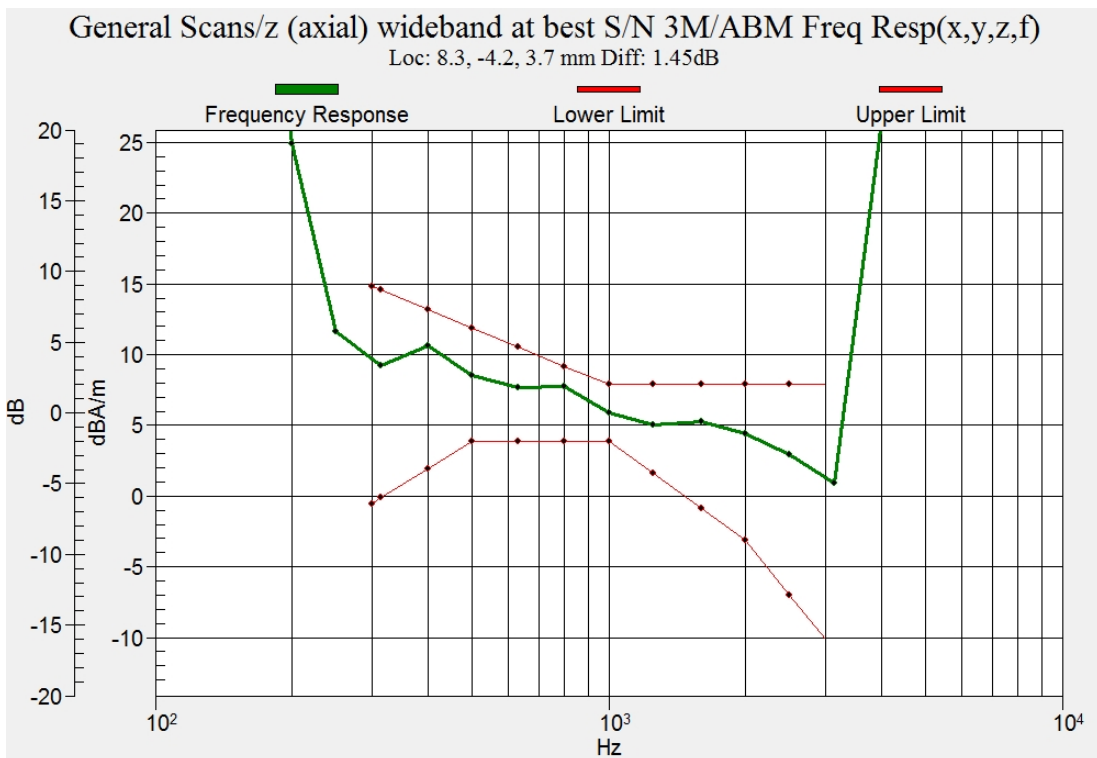
Figure C.8 Frequency Response of LTE B5
