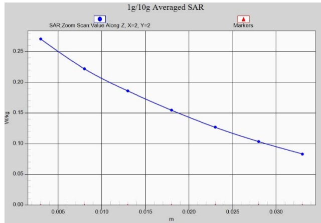
Fig.A.1- 19 Z-Scan at power reference point (LTE band14)
