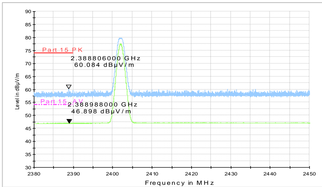
RE - Power-2.38GHz-2.45GHz
