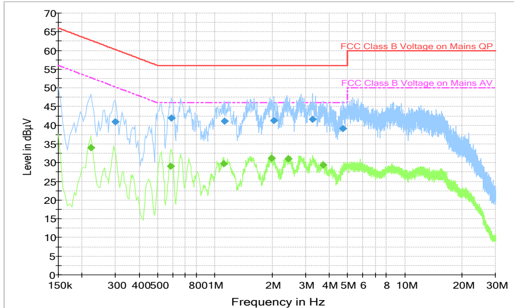
Fig A.2 Conducted Emission
