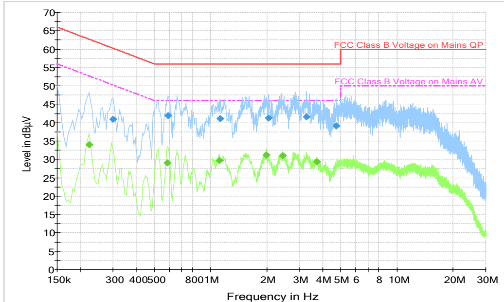
Fig A.1 Conducted Emission
