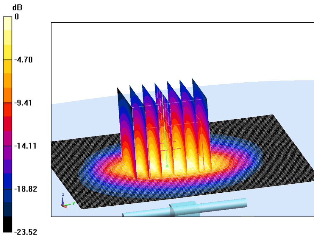
Fig.J.9-3 validation 2600 MHz 250mW
