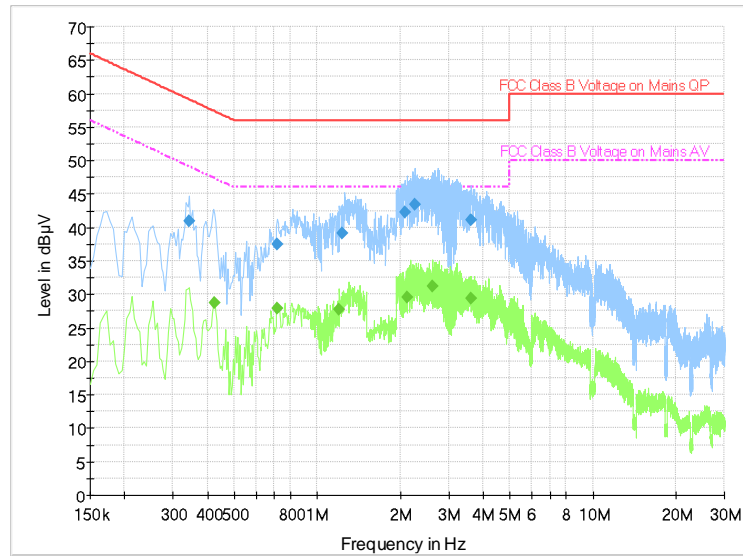
Fig.A.7.4 AC Power line Conducted Emission-802.11b
