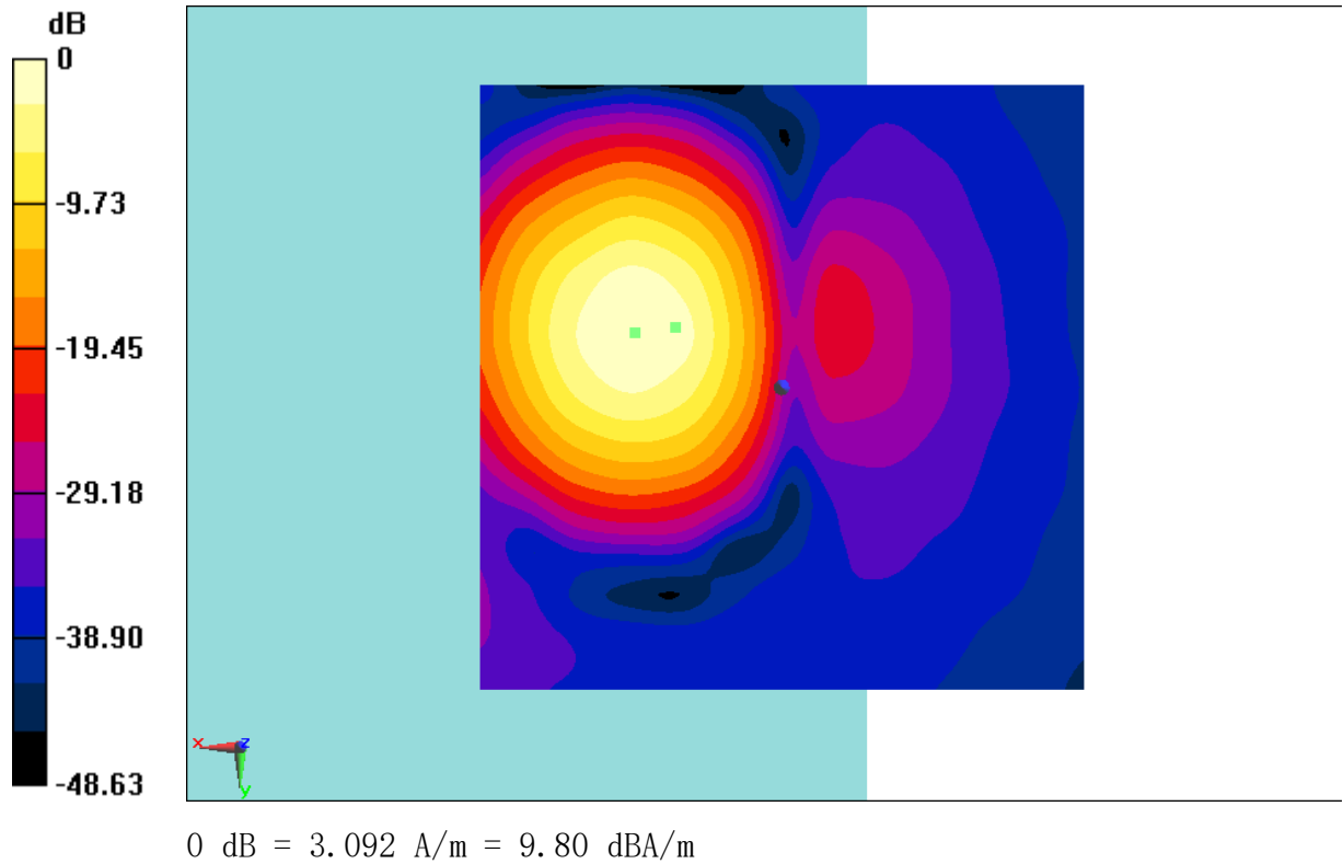
Fig B.18 T-Coil LTE B13
