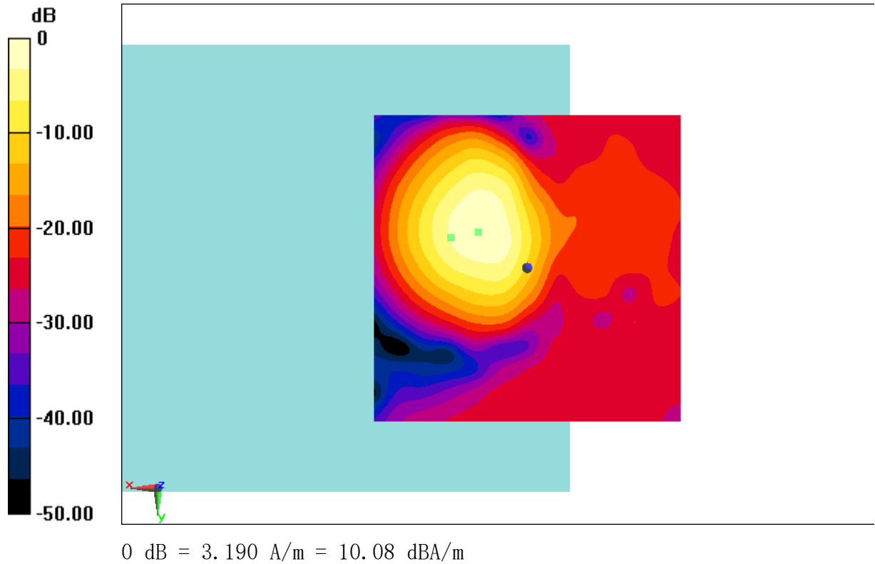
Fig B.10 T-Coil WCDMA 1700
