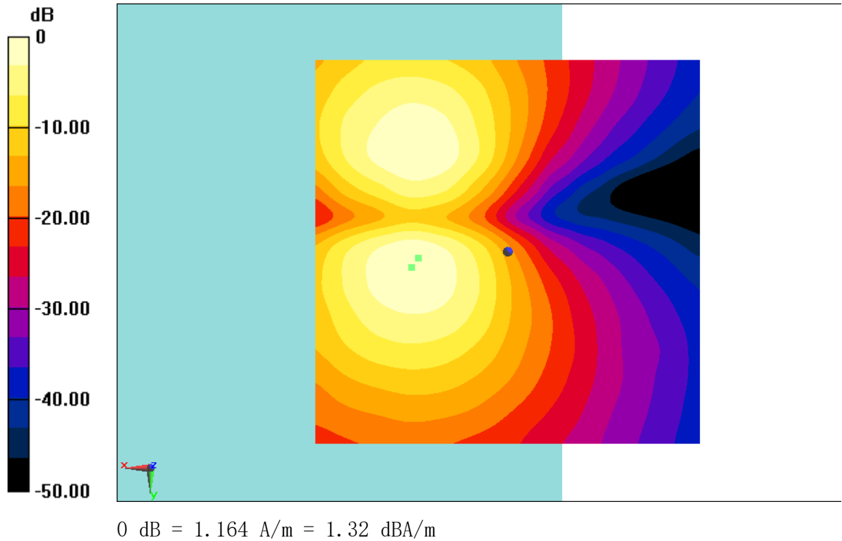
Fig B.21 T-Coil LTE B71
