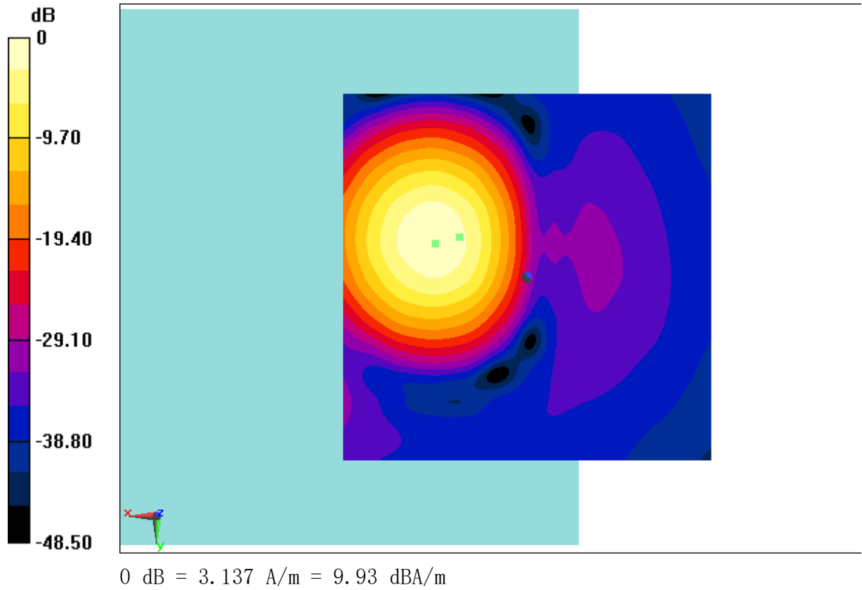
Fig B.12 T-Coil LTE B2
