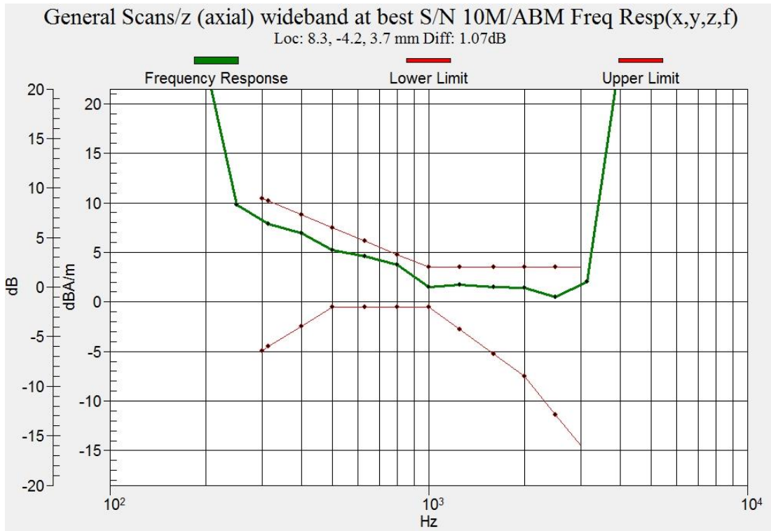
Figure C.9 Frequency Response of LTE B13
