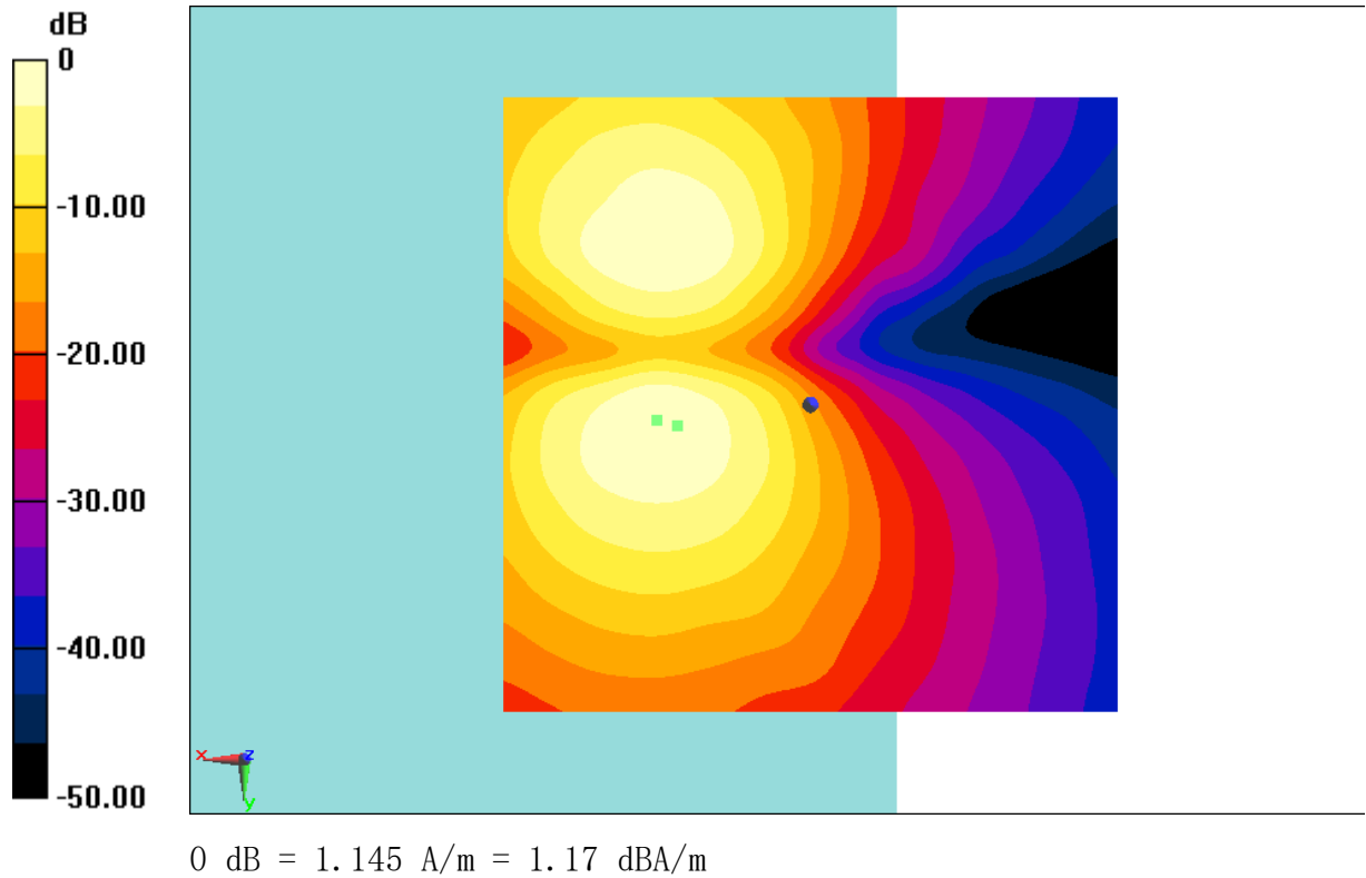
Fig B.15 T-Coil LTE B12
