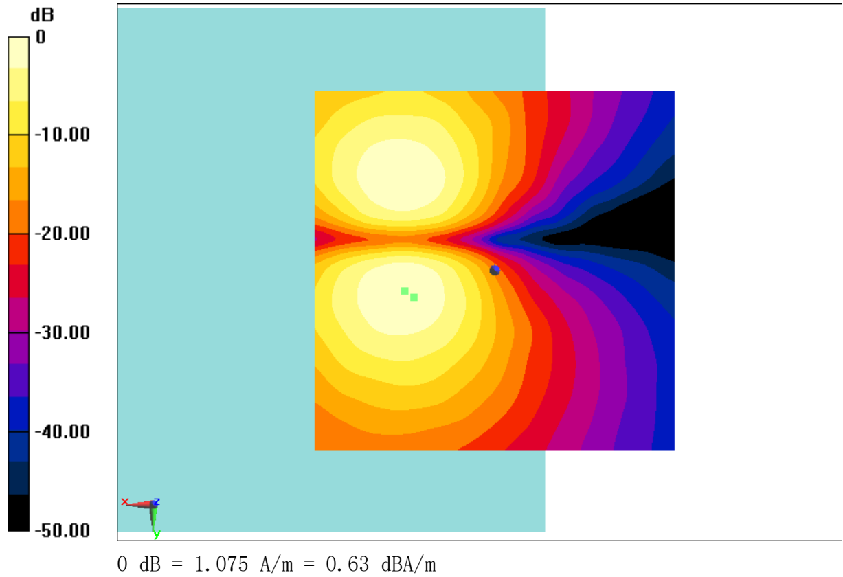
Fig B.13 T-Coil LTE B5
