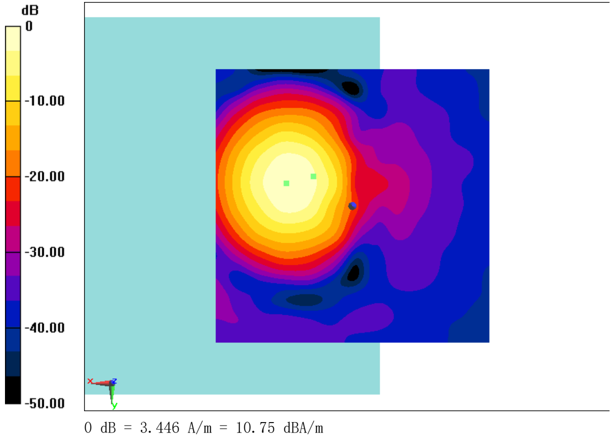
Fig B.24 T-Coil WiFi-2.4G
