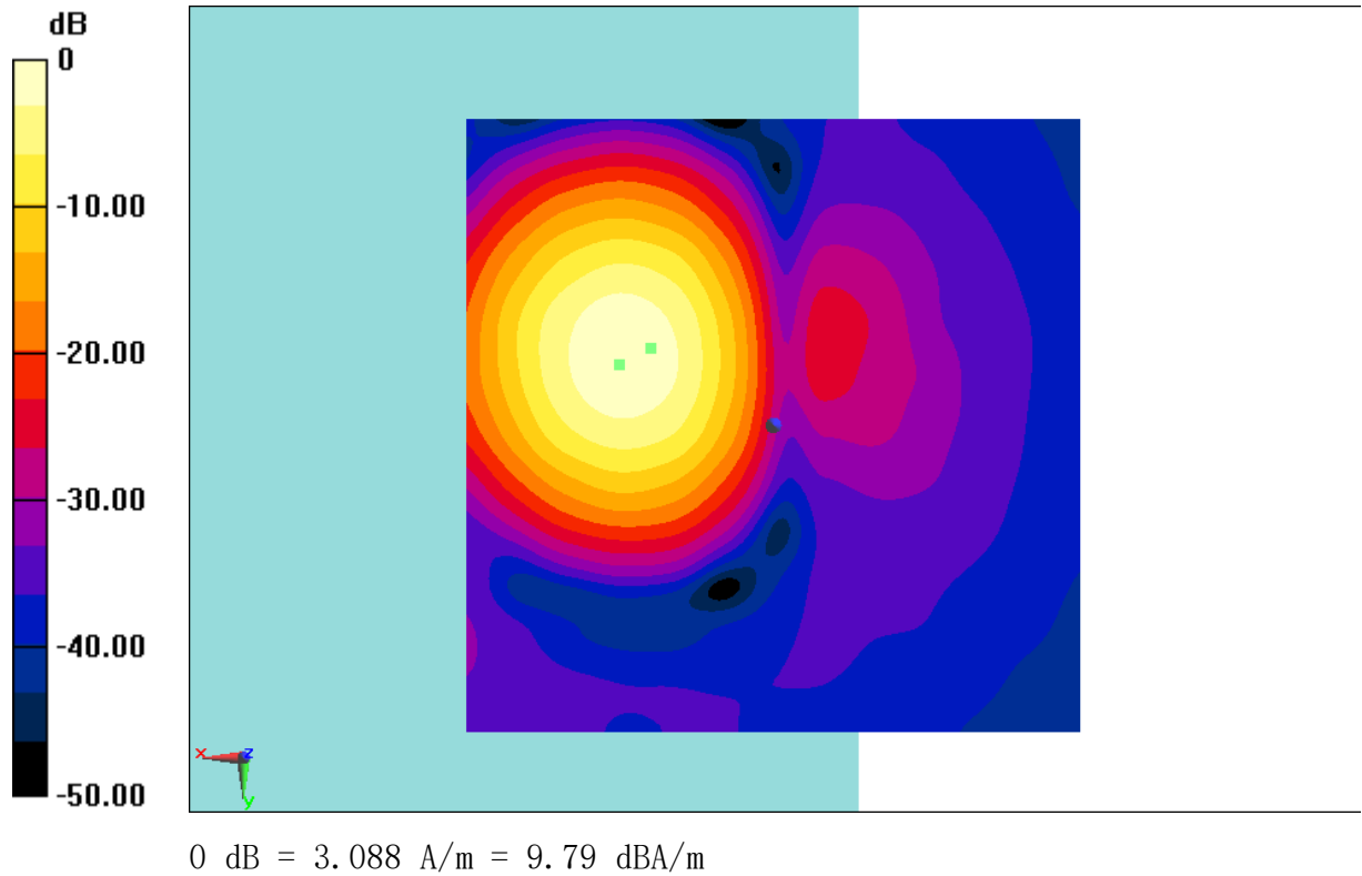
Fig B.16 T-Coil LTE B12
