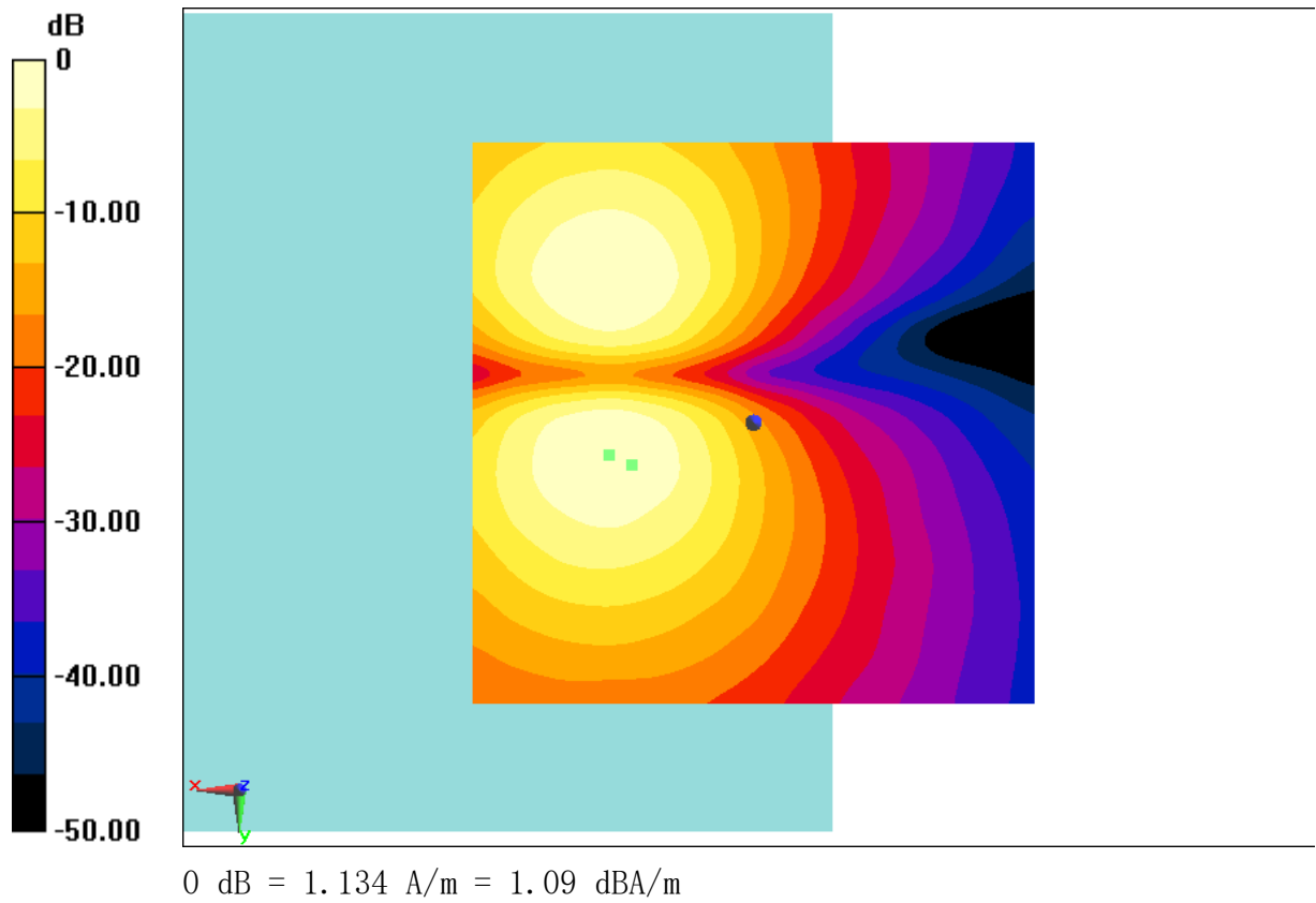
Fig B.11 T-Coil LTE B2
