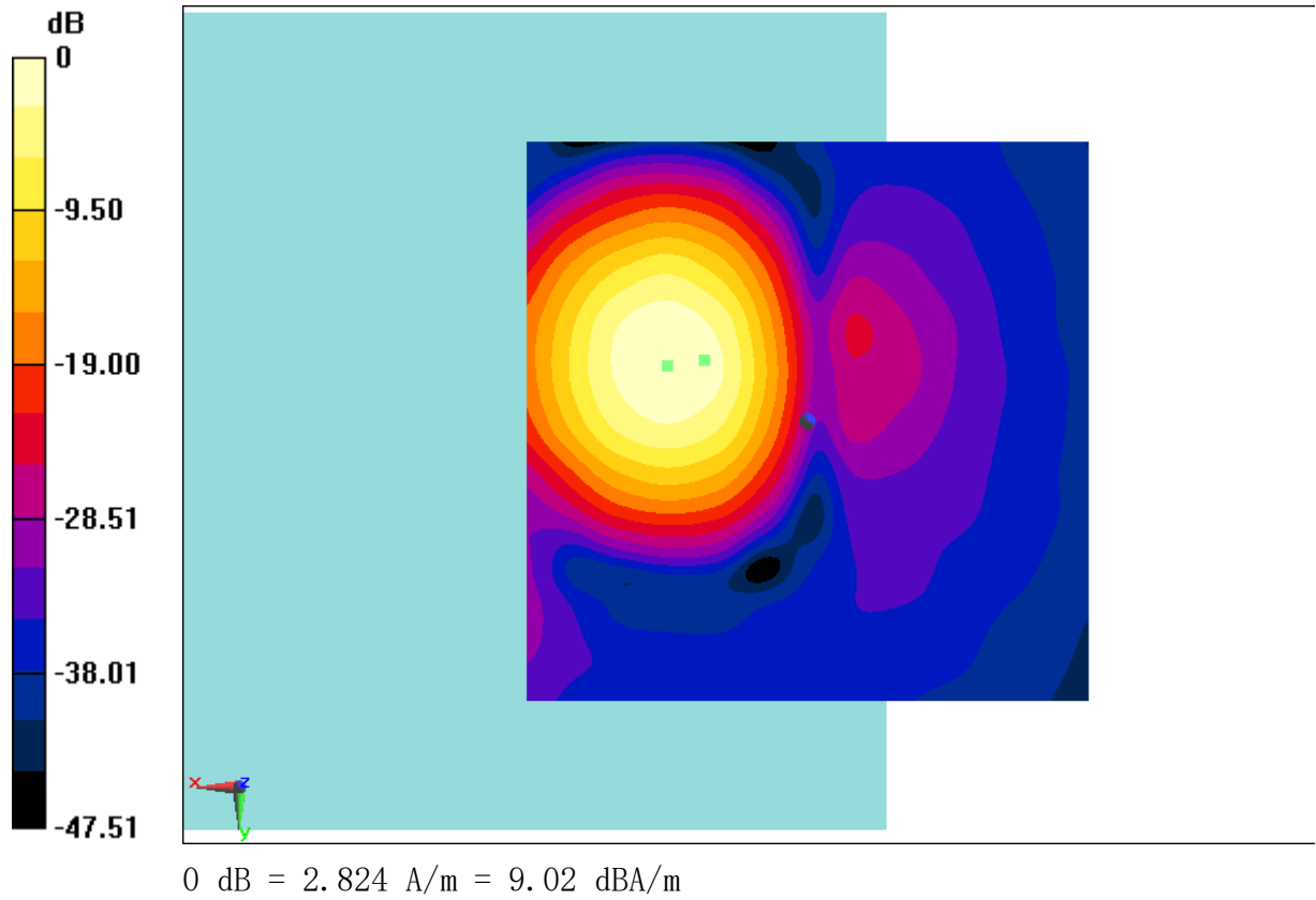
Fig B.14 T-Coil LTE B5
