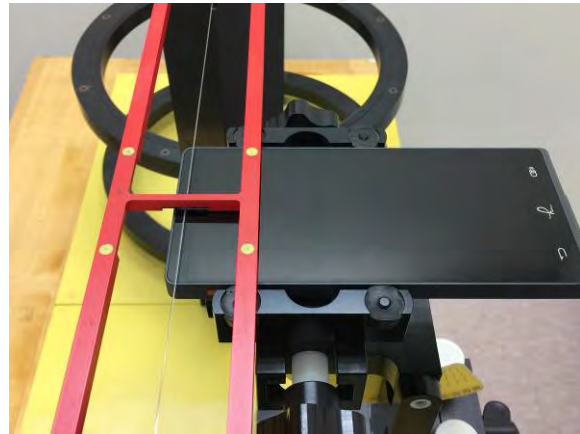
Fig. 1 Photograph of the DASY 5 measurement system
