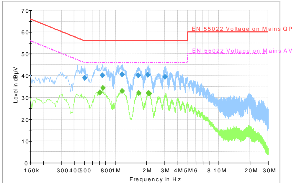
Fig A.14 Conducted Emission
