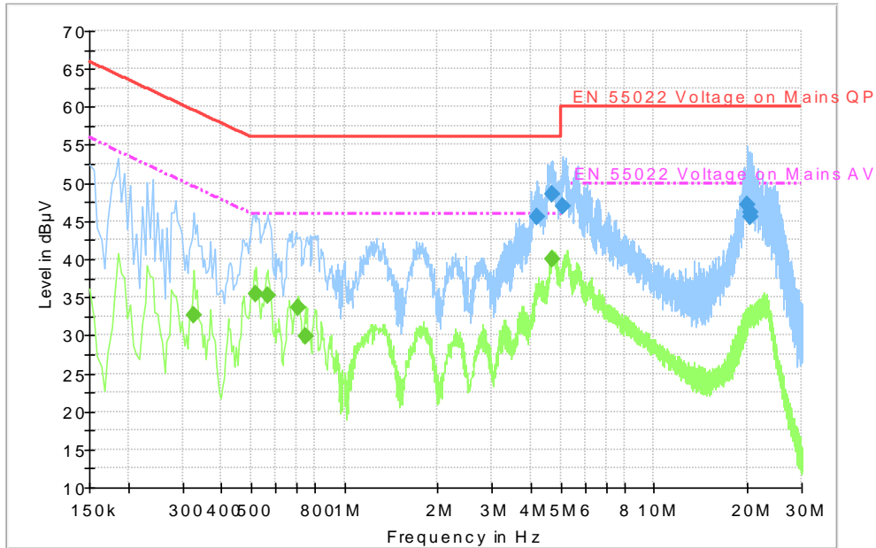
Fig A.15 Conducted Emission
