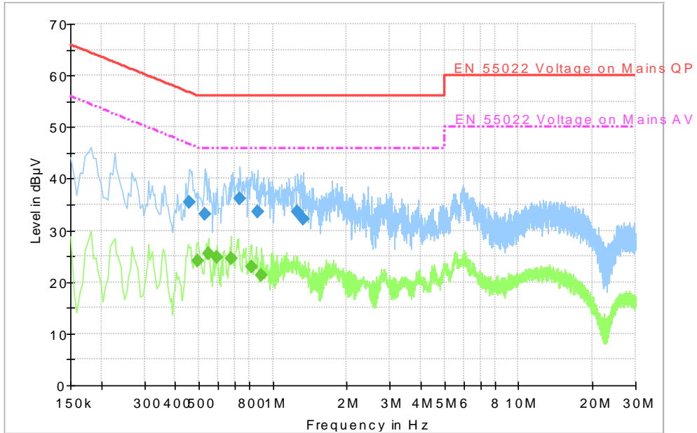
Fig A.13 Conducted Emission
