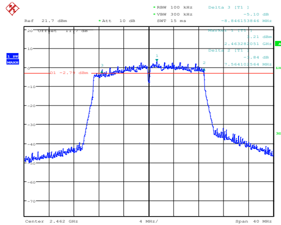
Fig.A.4.9 Occupied 6dB Bandwidth (802.11n-HT20, Ch 11)
