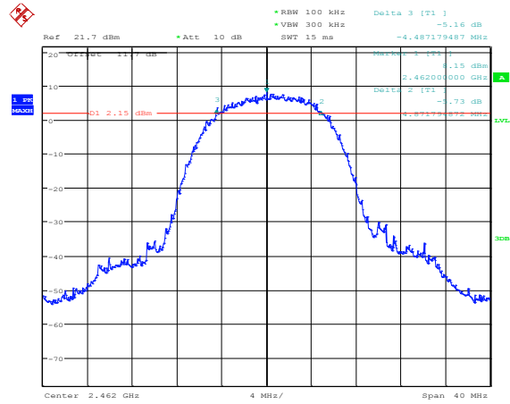
Fig.A.4.3 Occupied 6dB Bandwidth (802.11b, Ch 11)
