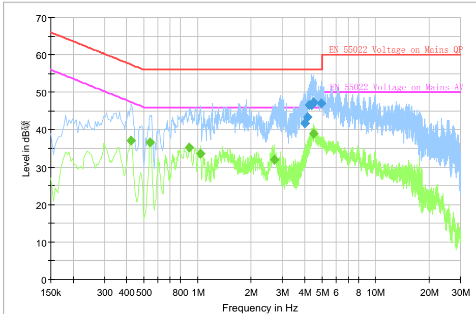
Fig A.17 Conducted Emission
