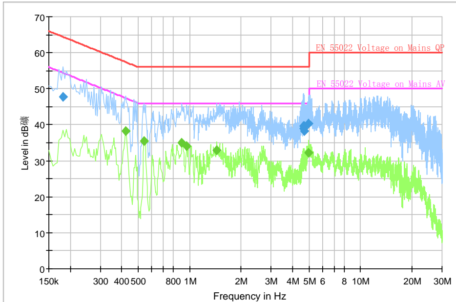
Fig A.19 Conducted Emission
