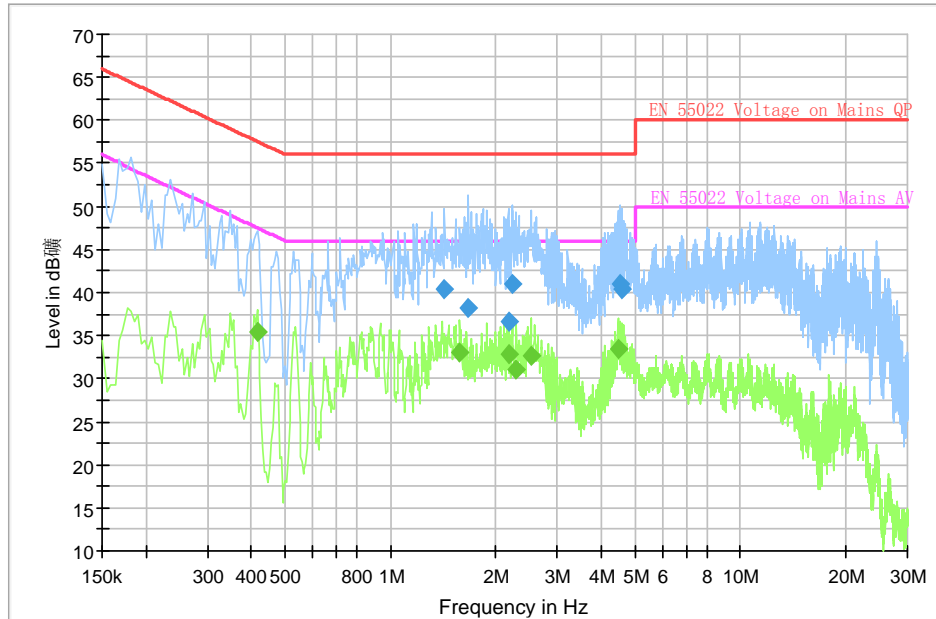
Fig A.18 Conducted Emission
