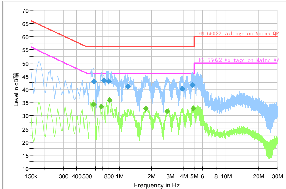
Fig A.16 Conducted Emission
