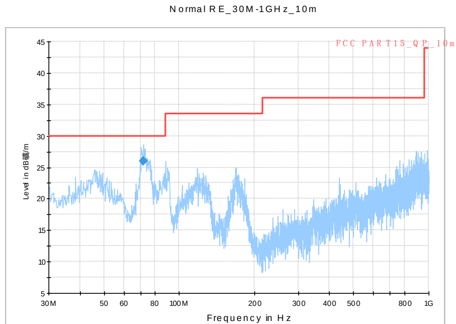
Fig.9 Radiated Emission from 30MHz to 1GHz
