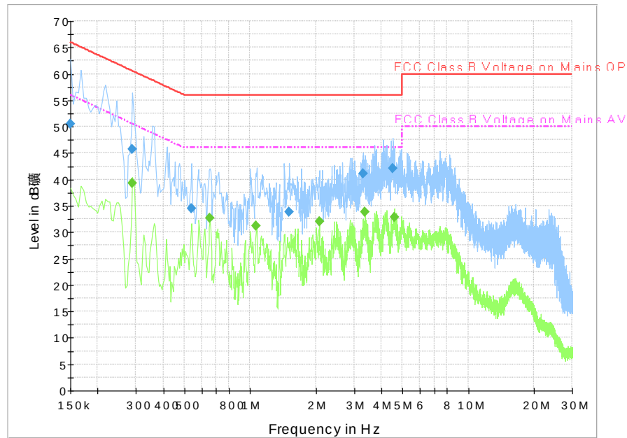
Fig.18 Conducted Emission
