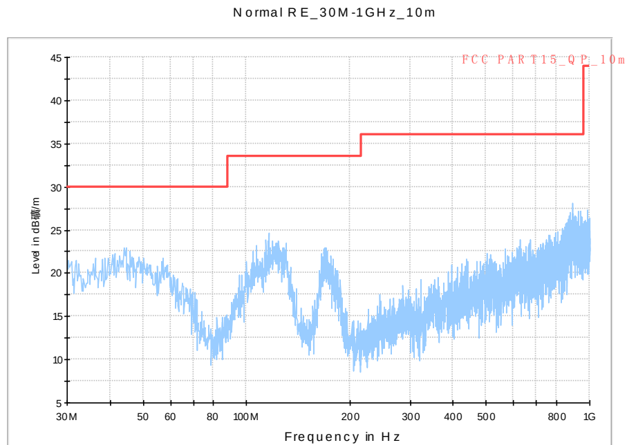
Fig.7 Radiated Emission from 30MHz to 1GHz
