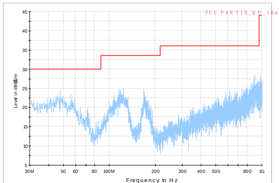
Fig.11 Radiated Emission from 30MHz to 1GHz
