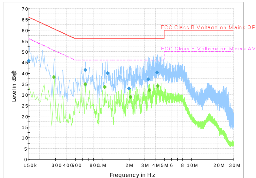
Fig.19 Conducted Emission
