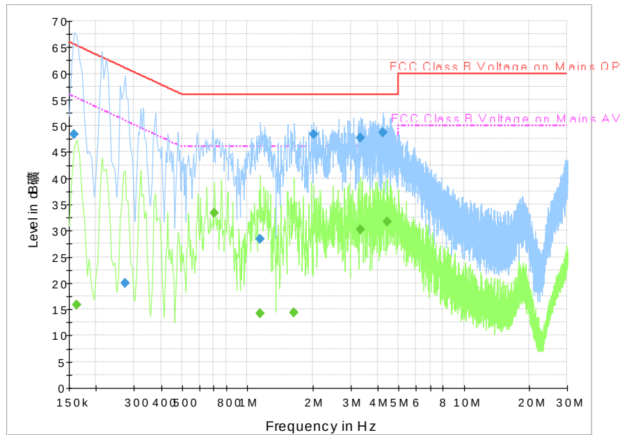
Fig.16 Conducted Emission
