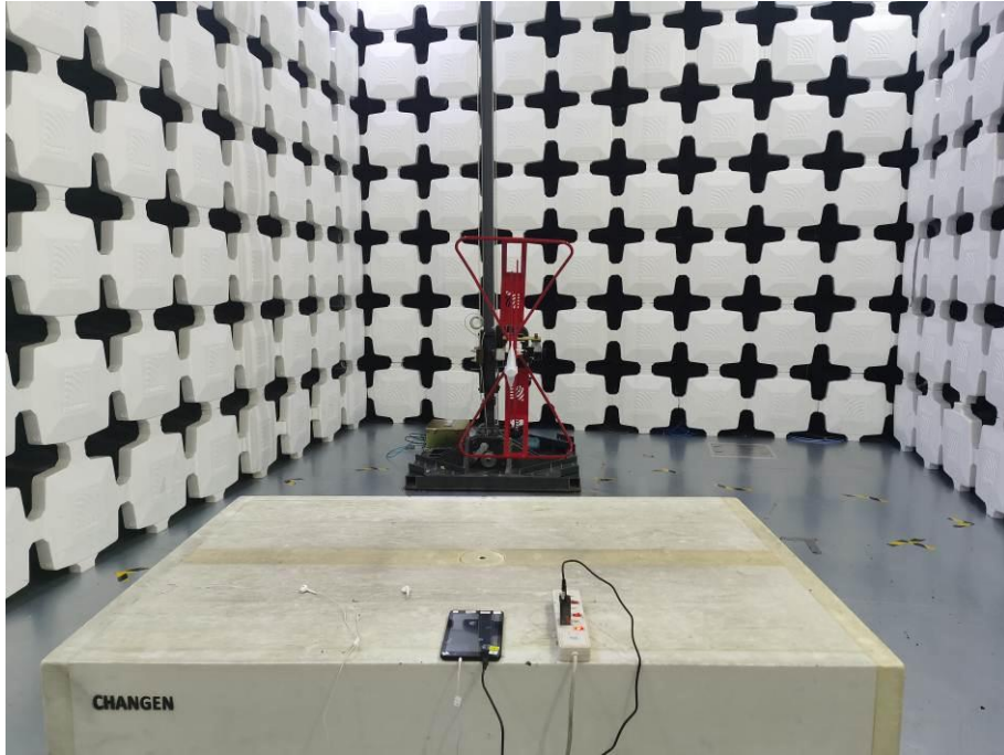
7. Radiated Emissions (Part 15B Charging Mode with FM Mode,30MHz-1GHz)
