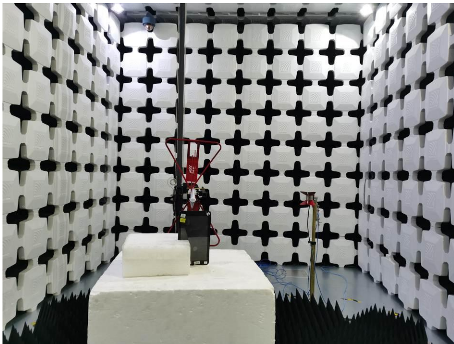
12. Radiated Emissions (Part 15C&Part 15E, 1GHz -18GHz)
