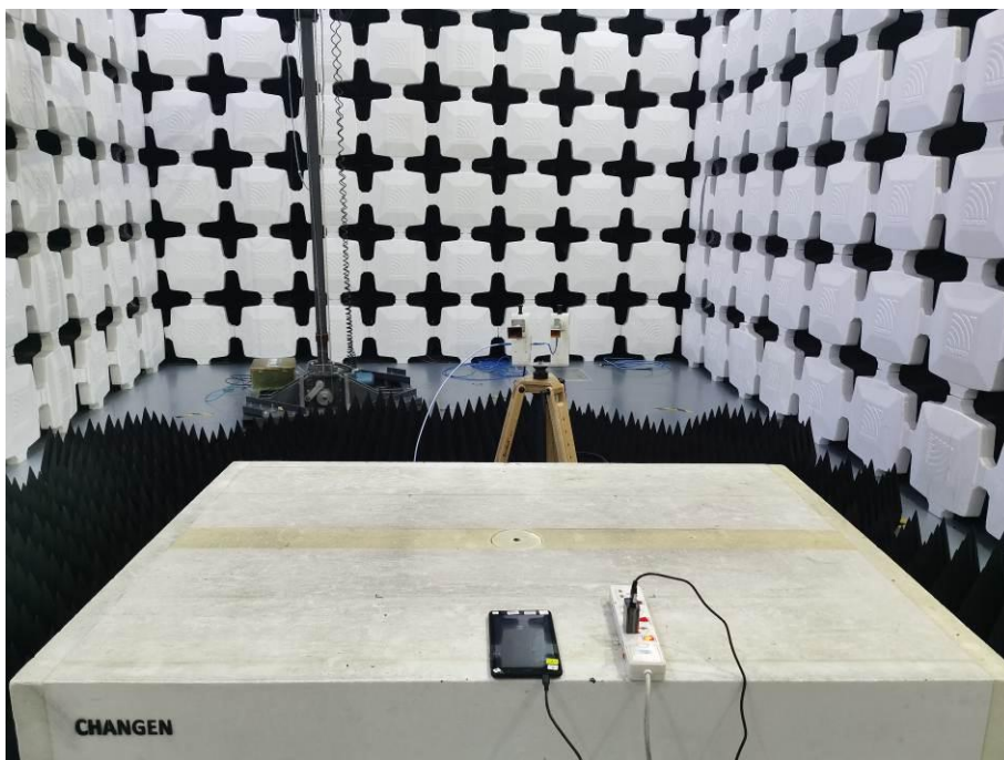
6. Radiated Emissions (Part 15B Charging Mode,18GHz-30GHz)
