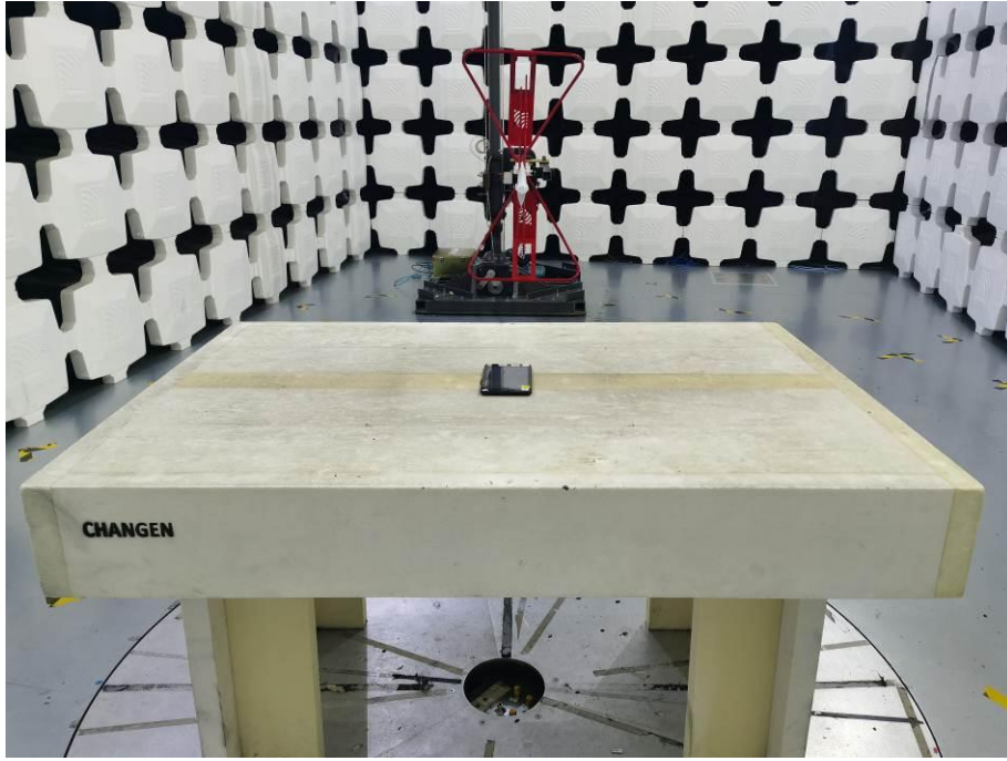
11. Radiated Emissions (Part 15C&Part 15E,30MHz-1GHz)
