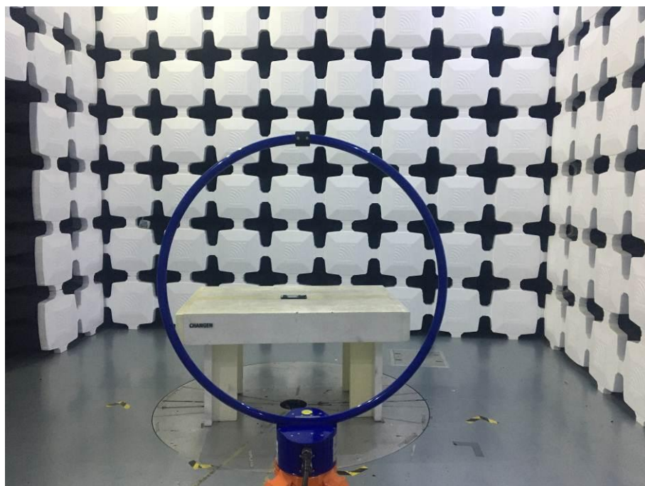
10. Radiated Emissions (Part 15C&Part 15E, 9kHz-30MHz)
