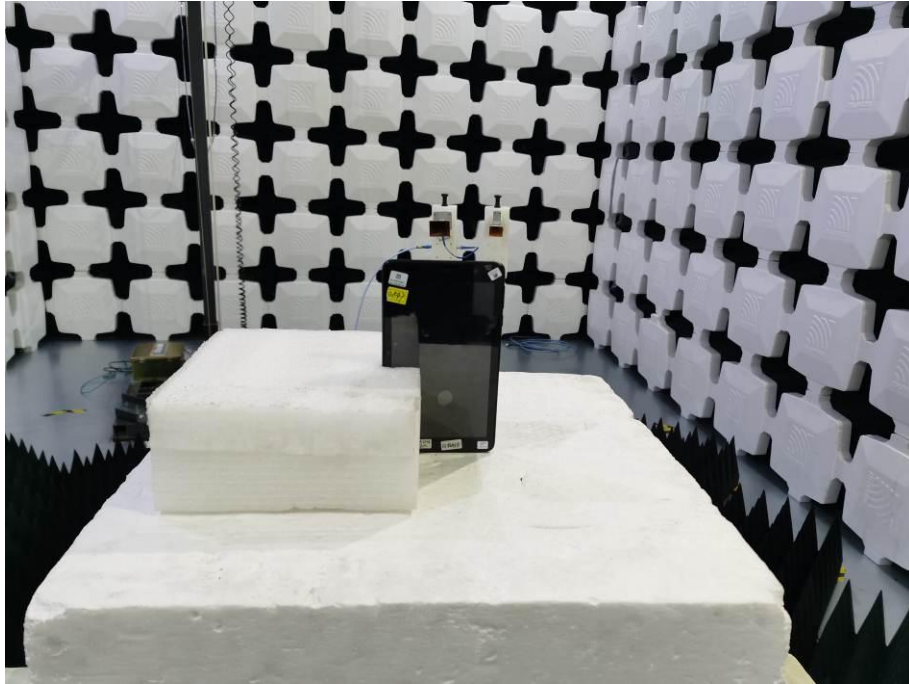
15. Radiated Emissions (Part 22/24/27, 18GHz-40GHz)
