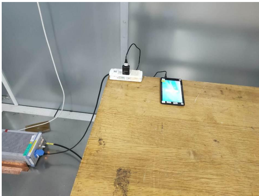
16. Conducted Emission (Part 15B, Charging Mode )
