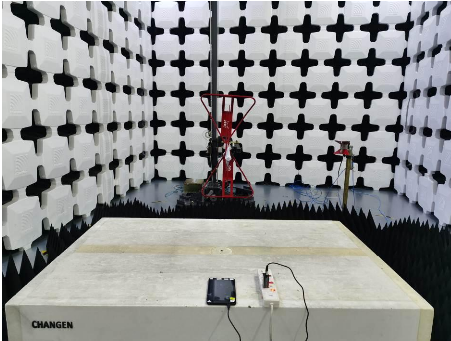
5. Radiated Emissions (Part 15B Charging Mode,1GHz-18GHz)
