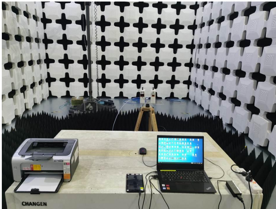
3. Radiated Emissions (Part 15B Data Transfer Mode,18GHz-30GHz)
