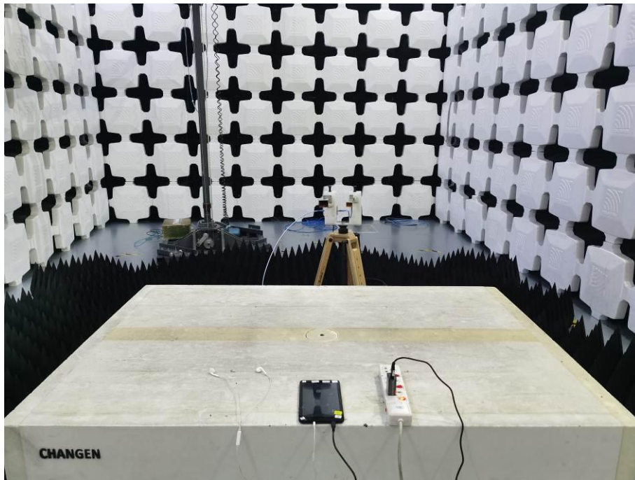
9. Radiated Emissions (Part 15B Charging Mode with FM Mode, 18GHz-30GHz)
