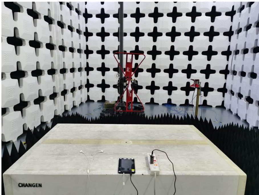
8. Radiated Emissions (Part 15B Charging Mode with FM Mode,1GHz-18GHz)
