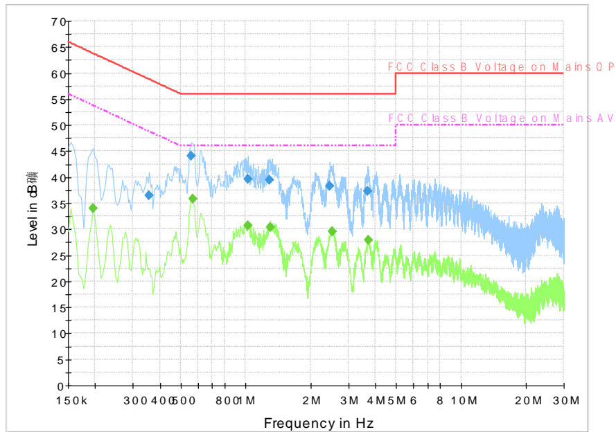
Fig. 24 Conducted Emission(802.11a, Ch40, TX)
