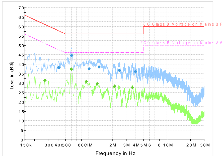
Fig. 23 Conducted Emission(802.11a, Ch40, TX)
