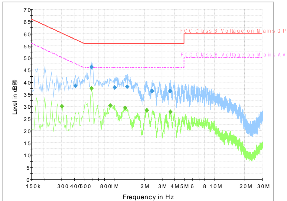
Fig. 25 Conducted Emission(802.11a, IDLE)
