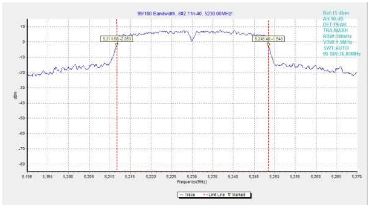
Fig. 79 99% Occupied bandwidth (802.11n-HT40, 5230MHz)
