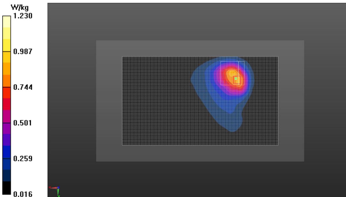
Fig.9 LTE Band 12
