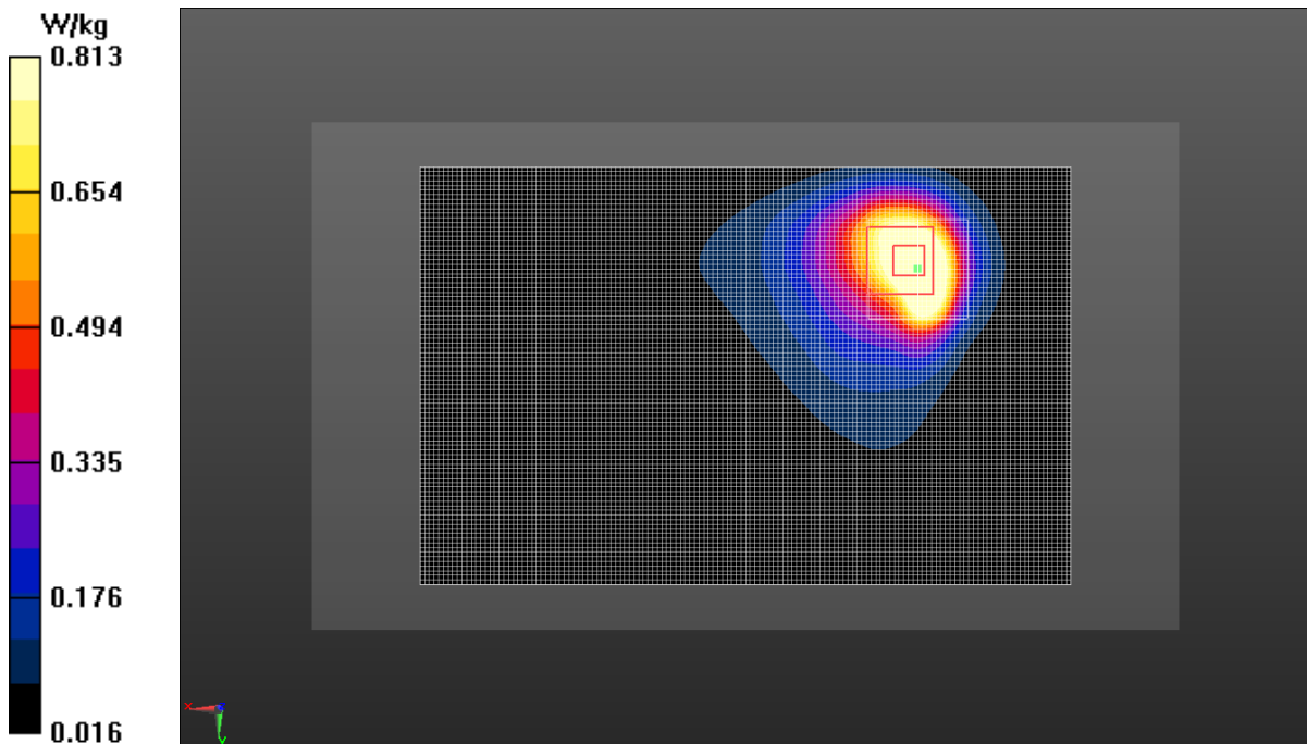
Fig.1 GSM 850 MHz
