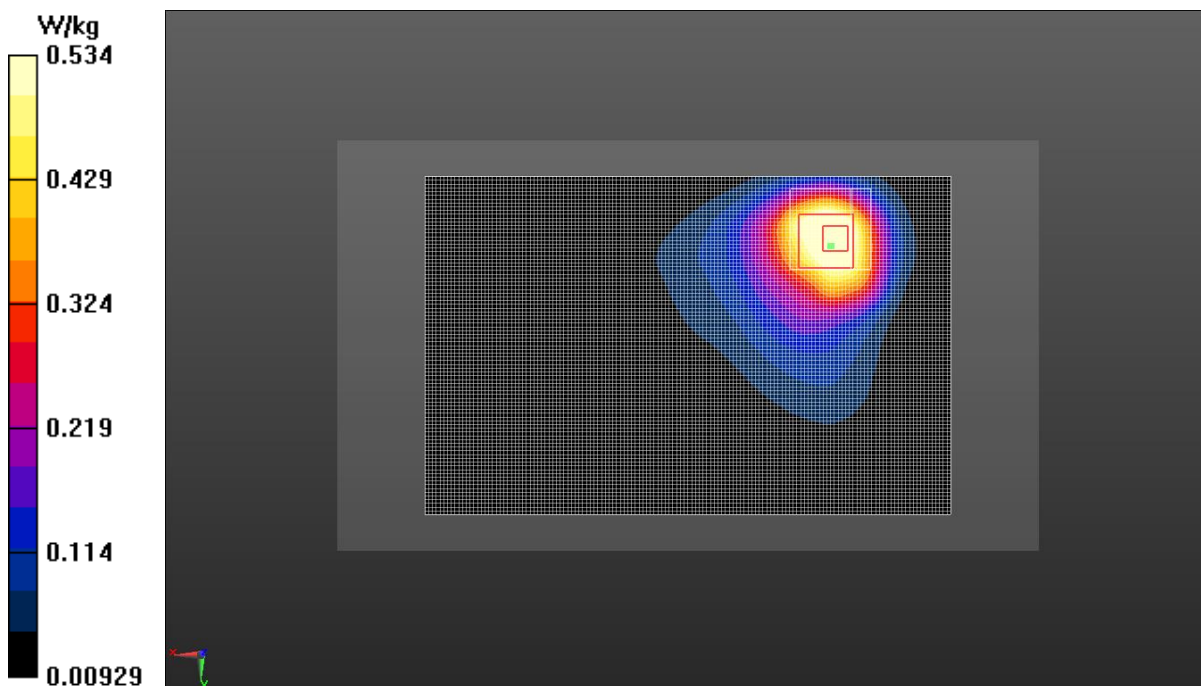
Fig.7 LTE Band 5
